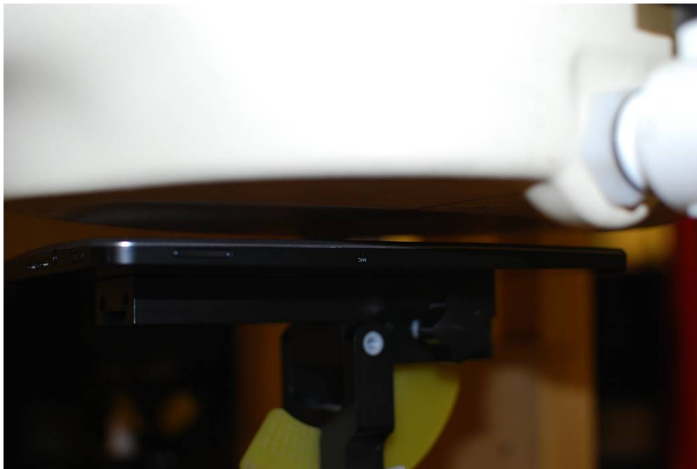
Figure 20-2 SAR Test Setup Photo – Back at 1.0 cm
