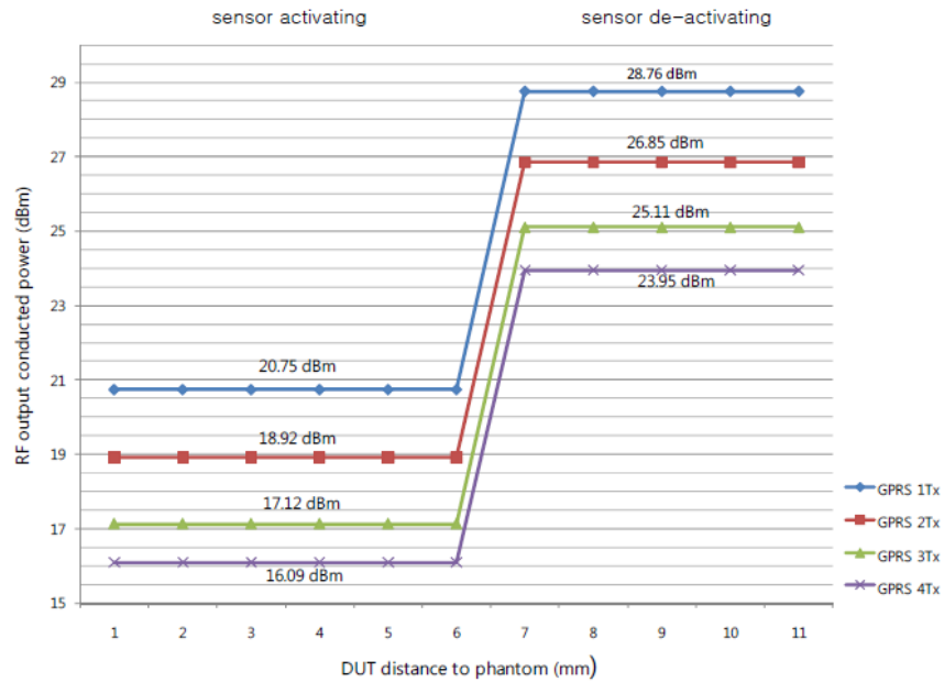
Figure 10-13 GPRS1900 Back off Power Reduction Graph – Top Edge at 45° Angle
