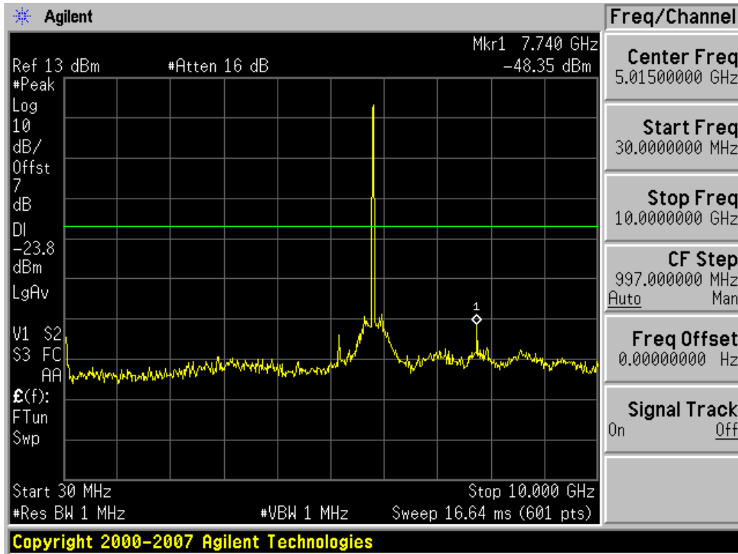
Plot 6-51. Conducted Spurious Plot (802.11a – Ch. 165)
