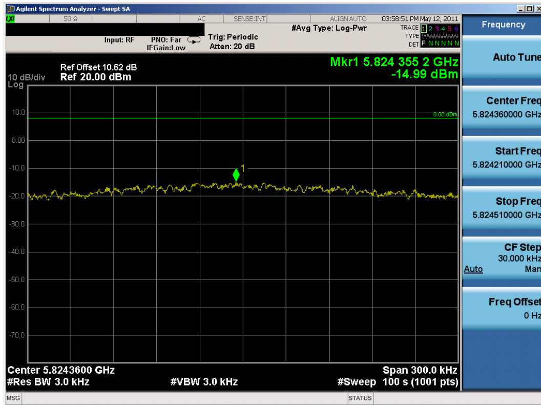
Plot 6-24. Power Spectral Density Plot (802.11a – Ch. 165)
