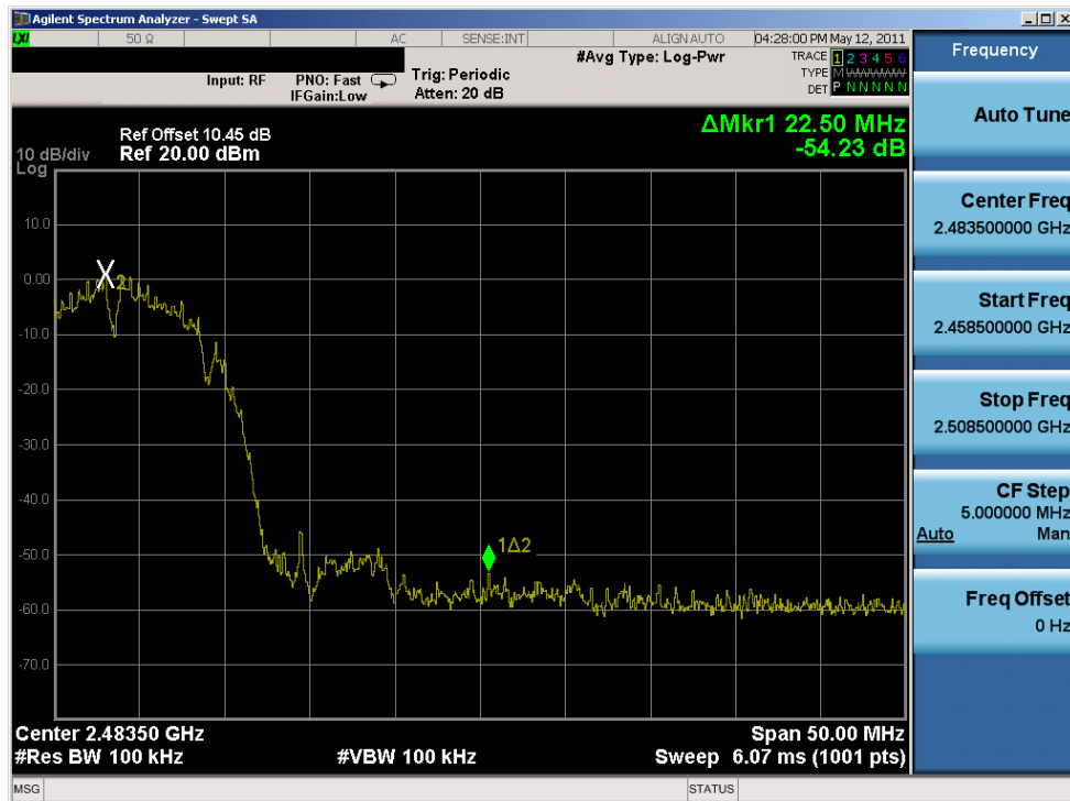
Plot 6-32. Band Edge Plot (802.11b – Ch. 11)
