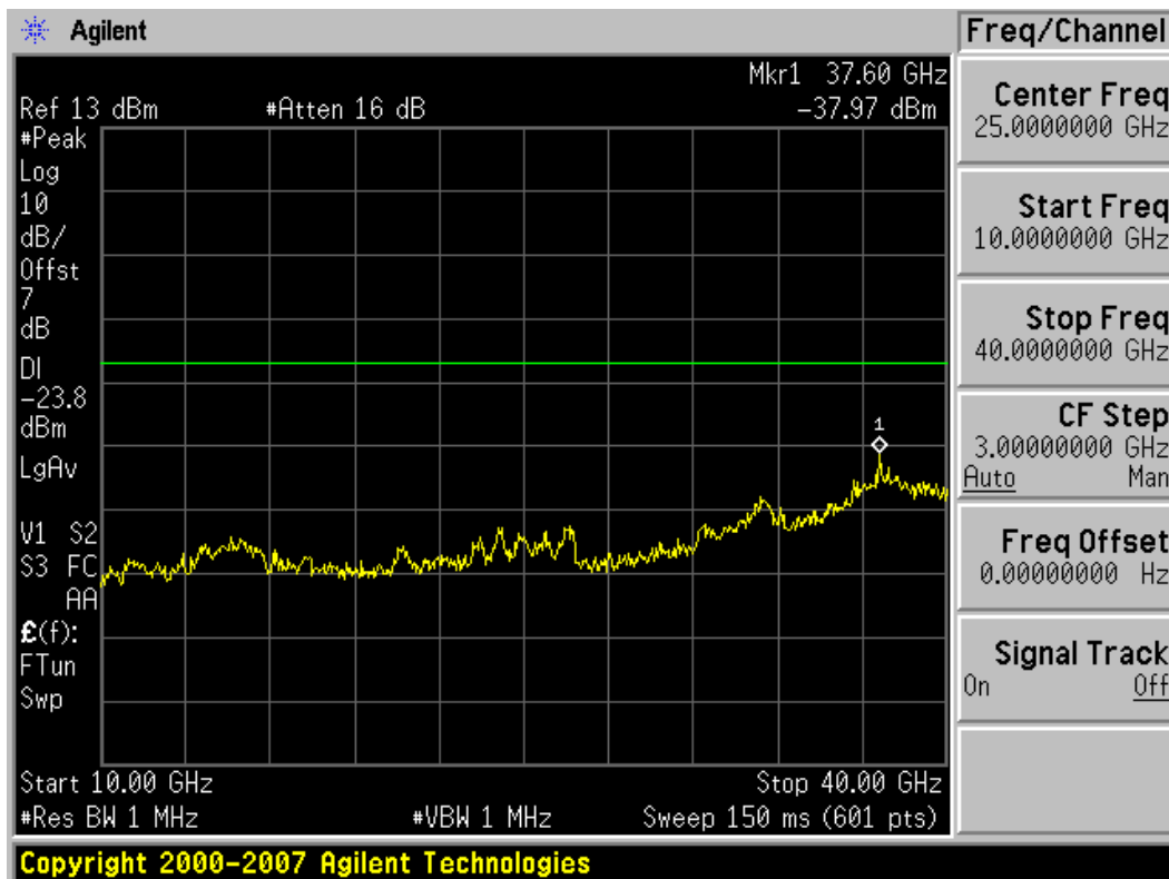
Plot 6-52. Conducted Spurious Plot (802.11a – Ch. 165)
