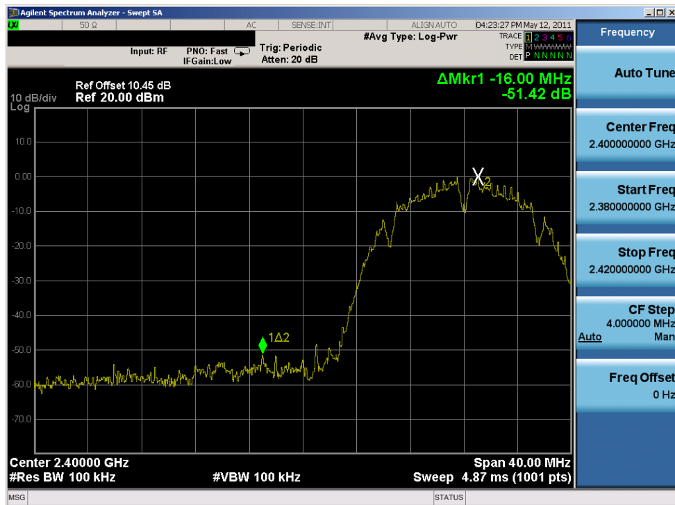
Plot 6-31. Band Edge Plot (802.11b – Ch. 1)
