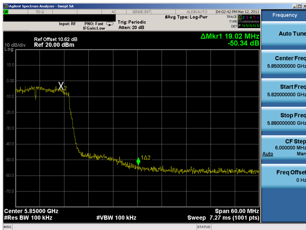
Plot 6-36. Band Edge Plot (802.11a – Ch. 165)
