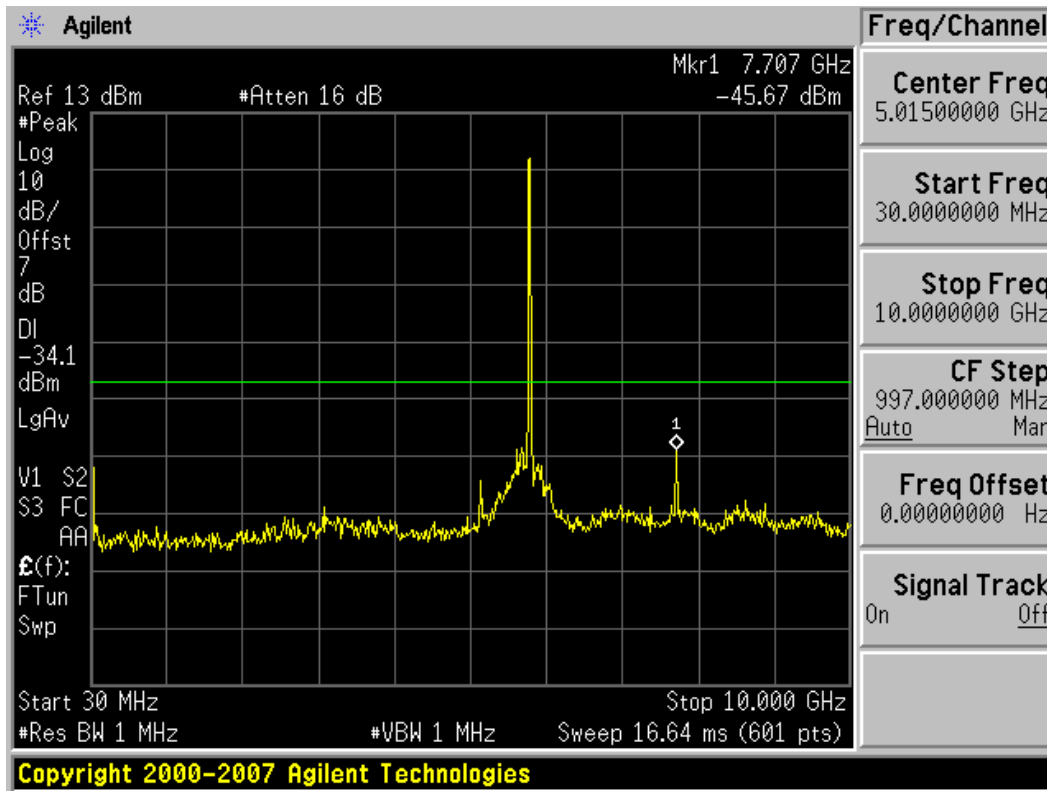
Plot 6-49. Conducted Spurious Plot (802.11a – Ch. 157)
