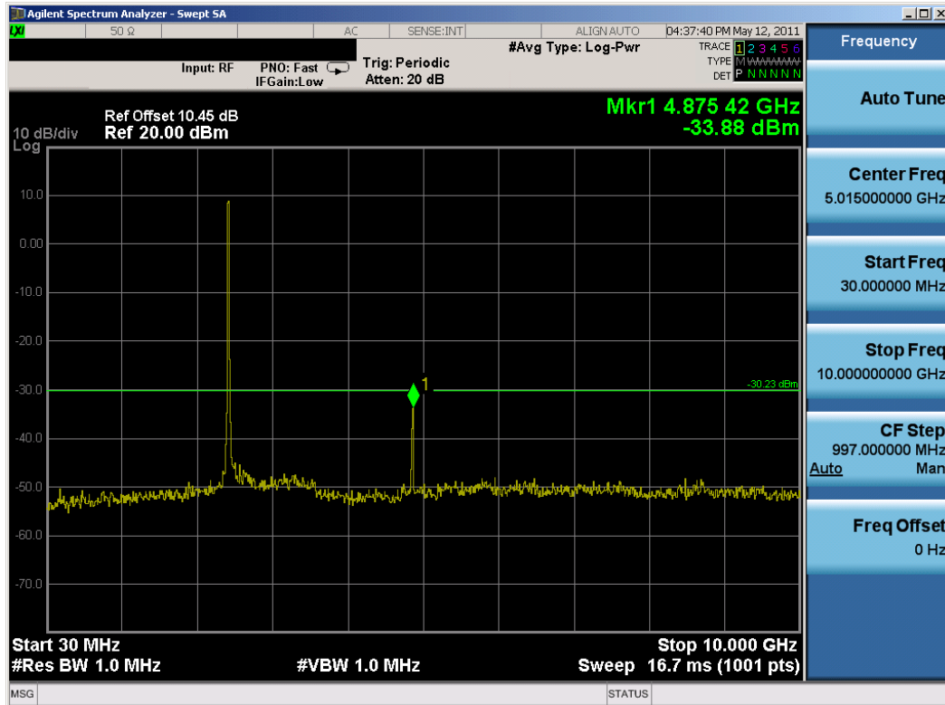
Plot 6-43. Conducted Spurious Plot (802.11g – Ch. 6)
