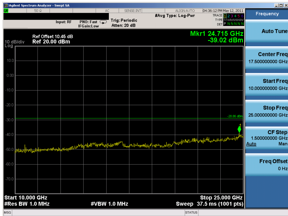
Plot 6-42. Conducted Spurious Plot (802.11g – Ch. 1)
