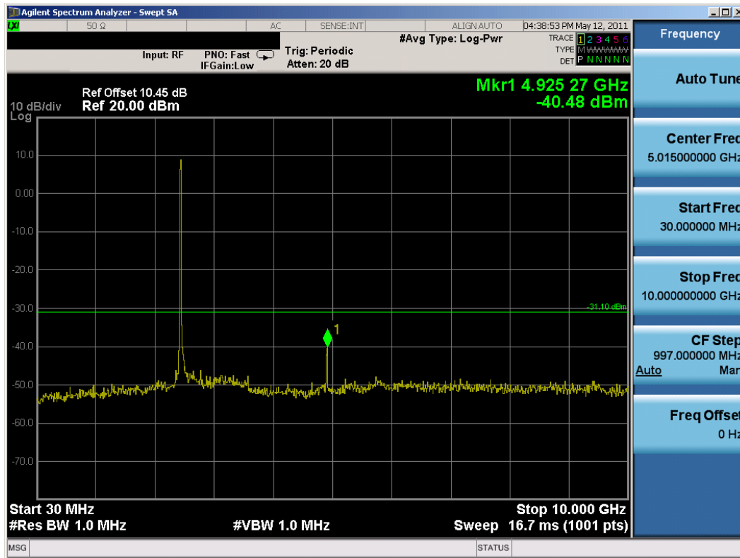
Plot 6-45. Conducted Spurious Plot (802.11g – Ch. 11)
