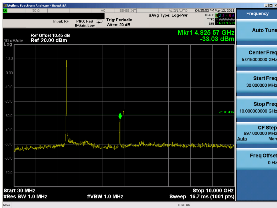
Plot 6-41. Conducted Spurious Plot (802.11g – Ch. 1)
