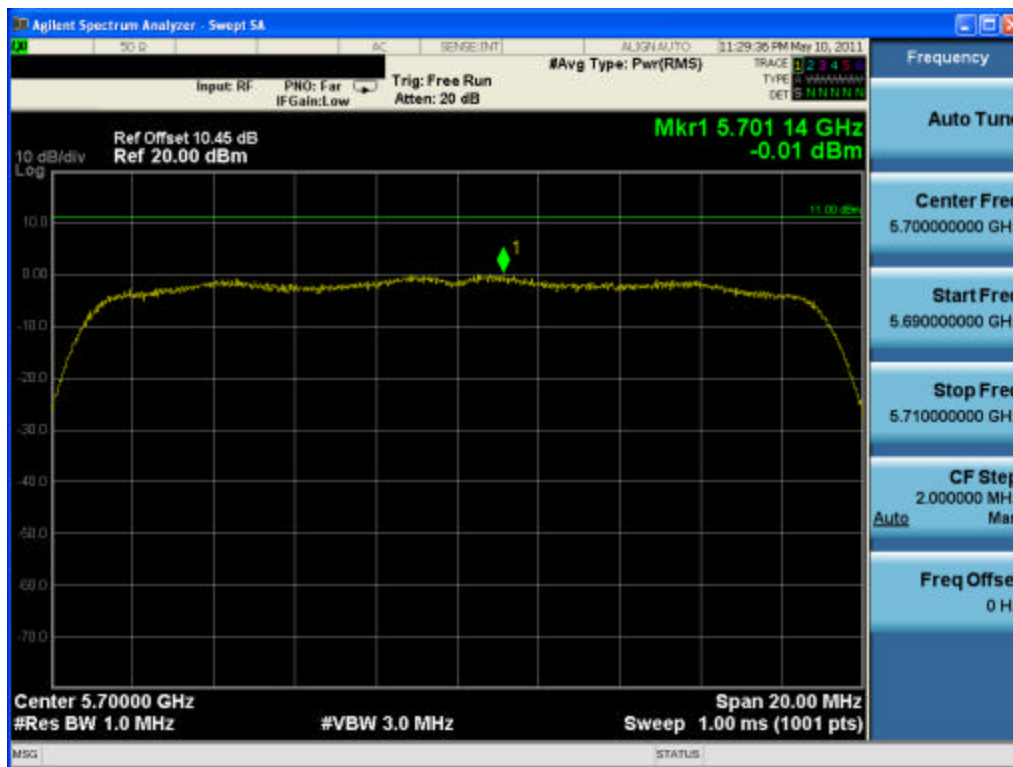
Plot 6-36. Peak Power Spectral Density Plot (802.11n (UNII) – Ch. 140)
