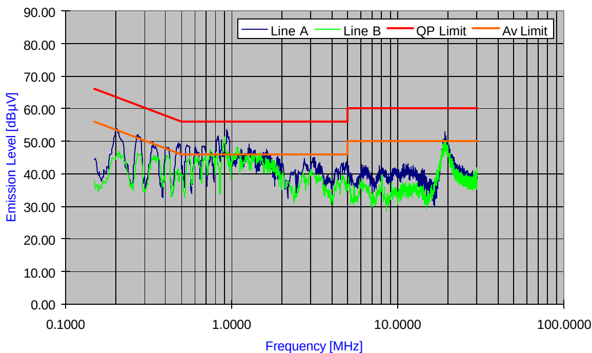
Plot 6-57. Line Conducted Plot with 802.11a (UNII-III Band)
