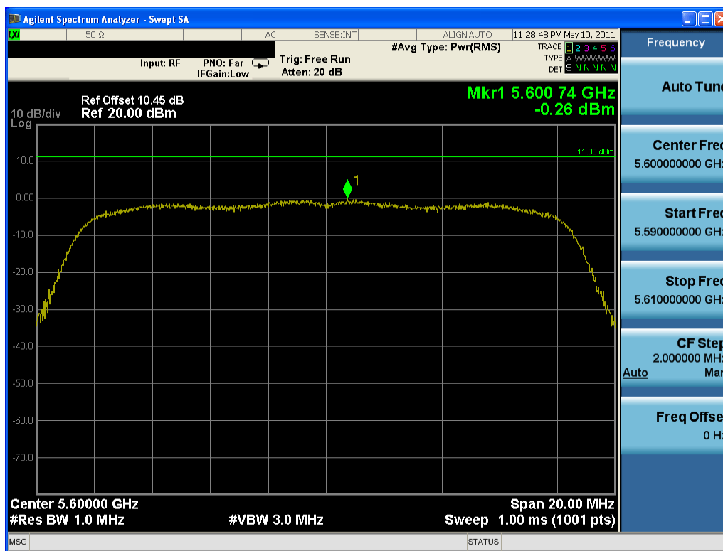
Plot 6-32. Peak Power Spectral Density Plot (802.11a (UNII) – Ch. 120)
