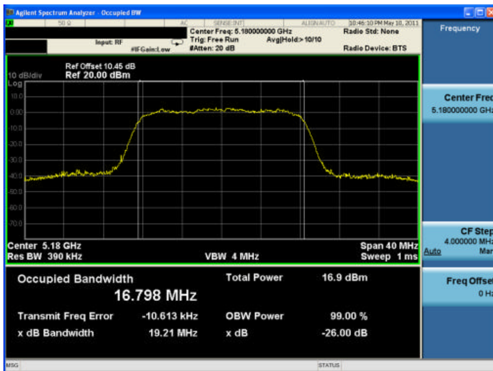
Plot 6-1. 26dB Bandwidth Plot (802.11a (UNII) – Ch. 36)
