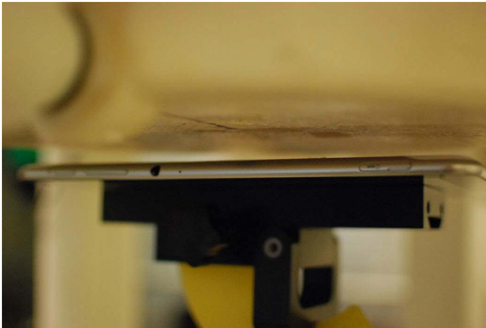
SAR Test Setup Photograph 2 – Back at 1.0 cm
