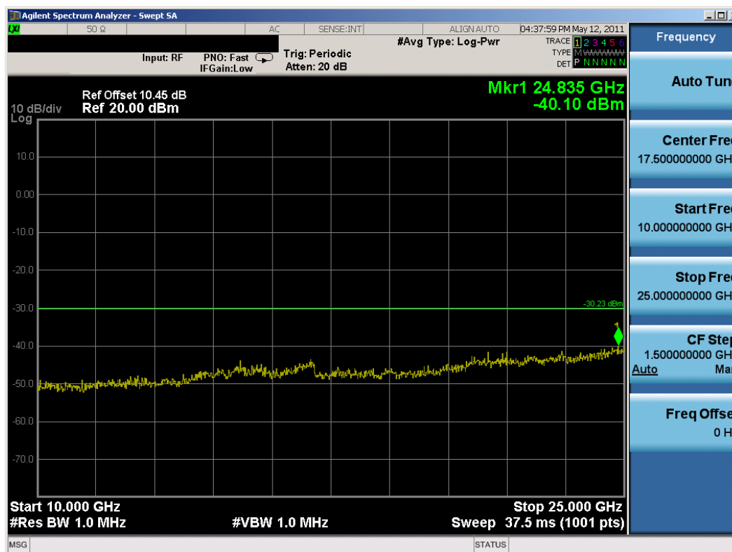
Plot 6-44. Conducted Spurious Plot (802.11g – Ch. 6)
