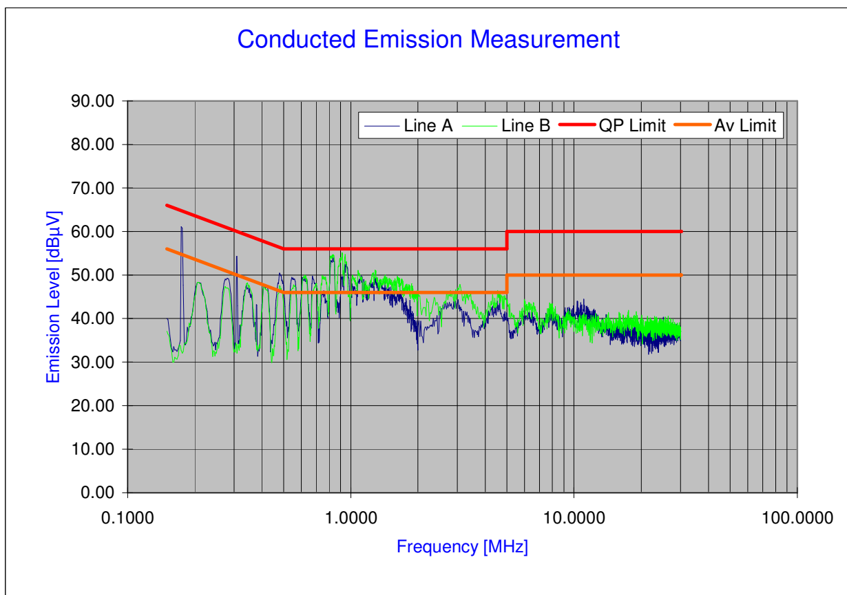
Plot 6-56. Line Conducted Plot with 802.11n
