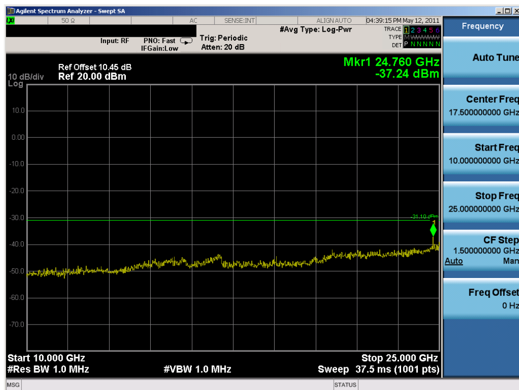
Plot 6-46. Conducted Spurious Plot (802.11g – Ch. 11)
