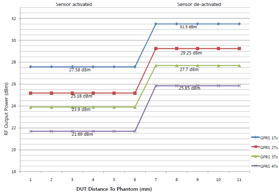
Figure 9-6 GPRS 850 Back off Power Reduction Graph - Top at 0° Angle
