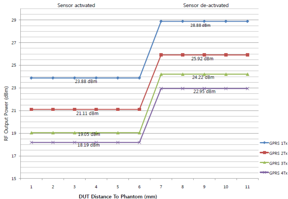
Figure 9-7 GPRS 1900 Back off Power Reduction Graph - Top at 0° Angle
