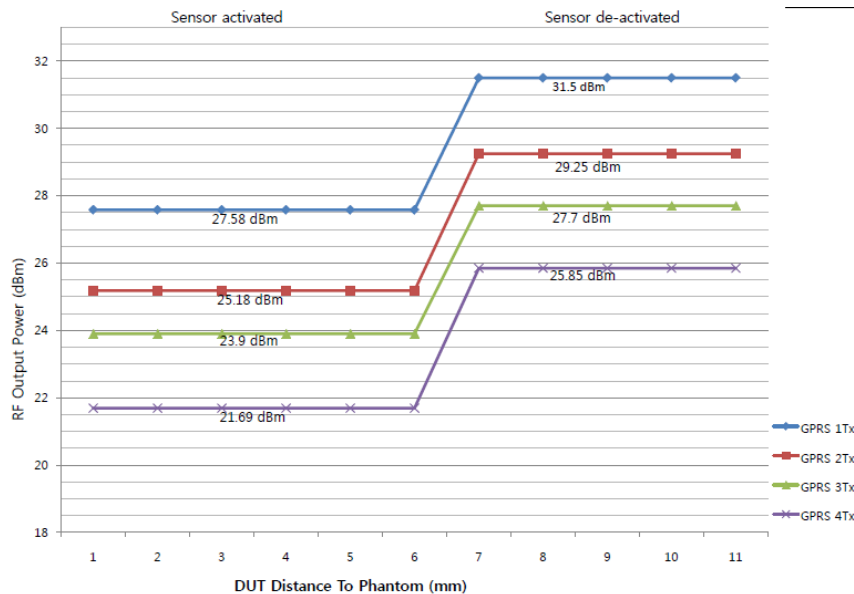
Figure 9-8 GPRS 850 Back off Power Reduction Graph - Top Edge at 60° Angle
