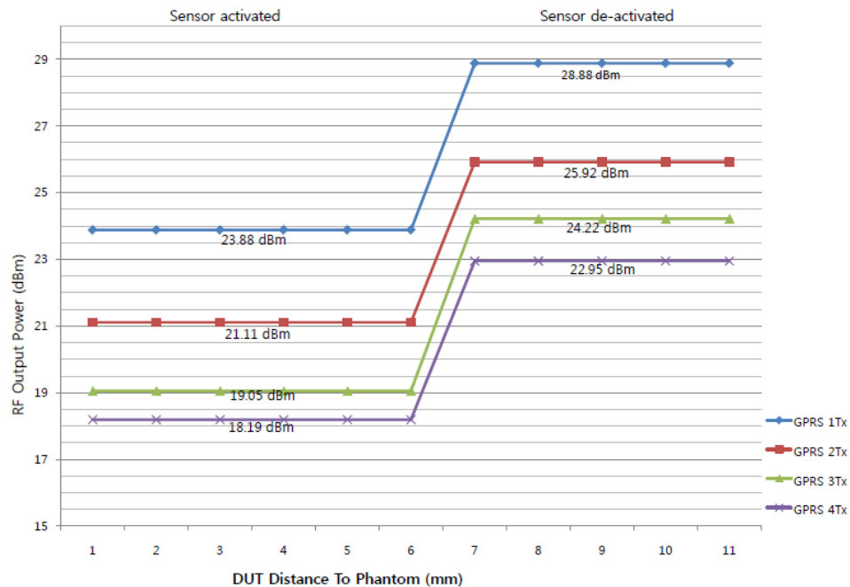
Figure 9-13 GPRS 1900 Back off Power Reduction Graph - Left Edge at 60° Angle
