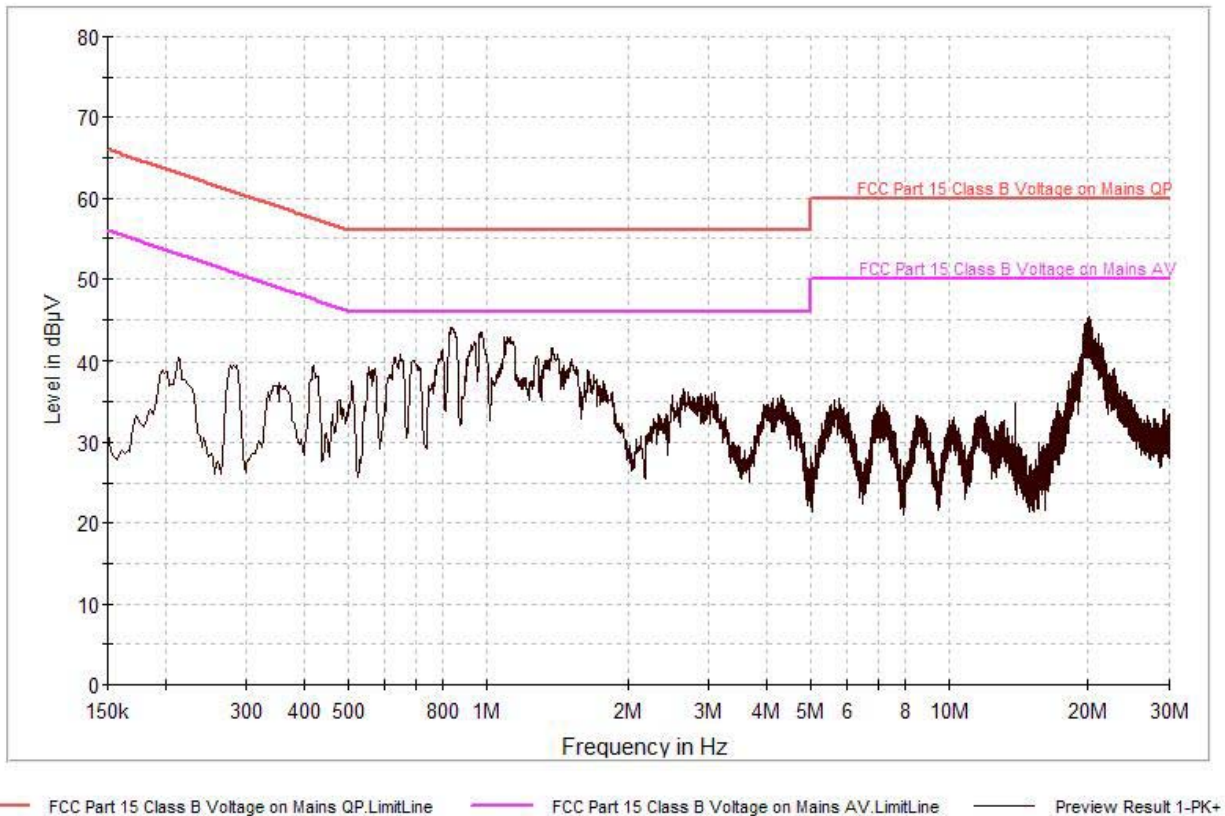
Plot 6-23. Line Conducted Plot with Bluetooth ON (N)
