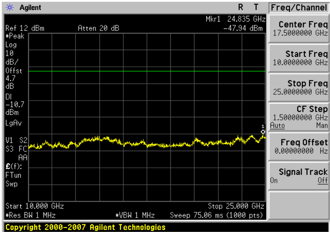
Plot 6-17. Conducted Spurious Plot (Bluetooth, 3Mbps – Ch. 0)
