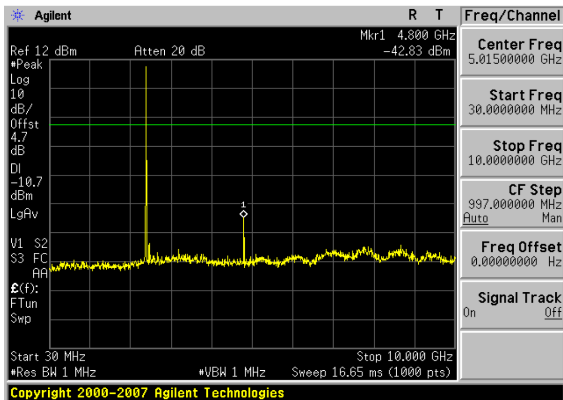
Plot 6-16. Conducted Spurious Plot (Bluetooth, 3Mbps – Ch. 0)
