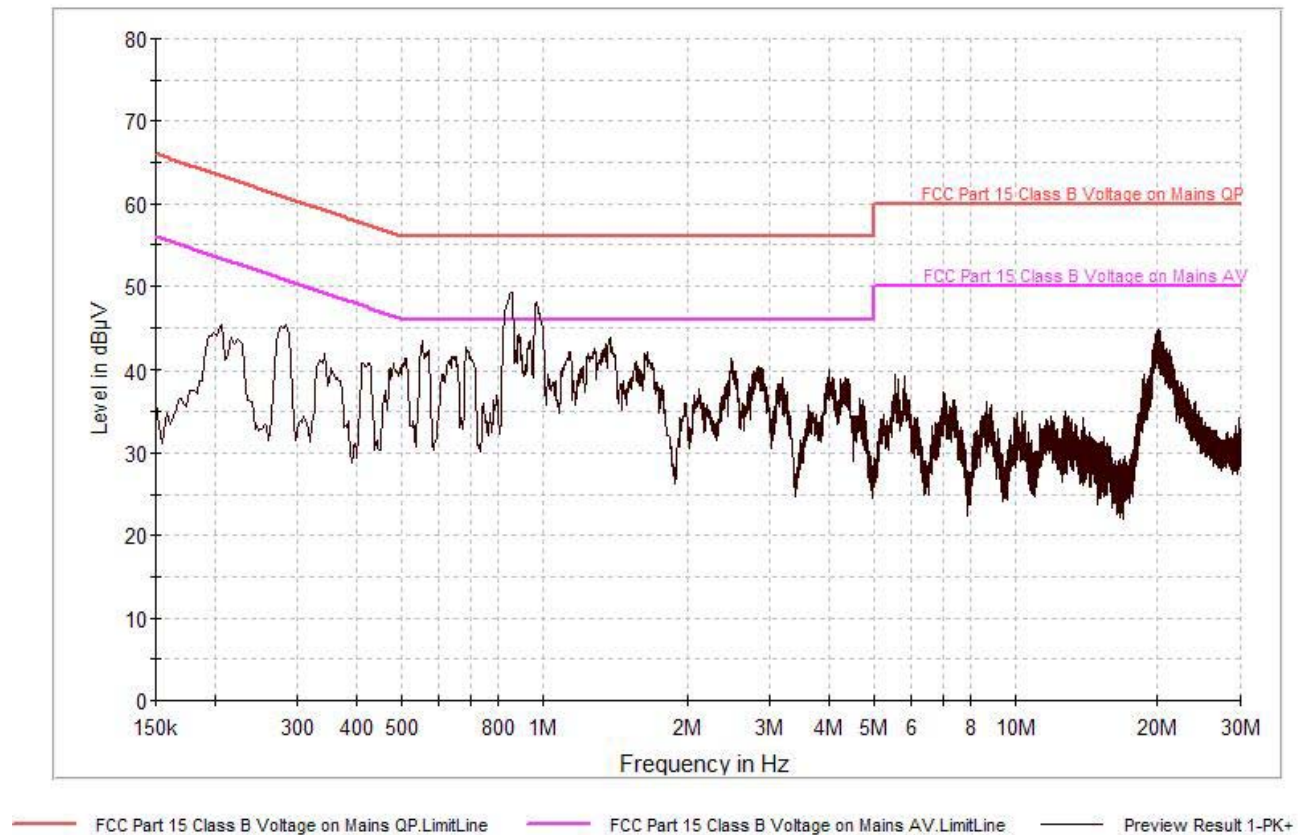
Plot 6-22. Line Conducted Plot with Bluetooth ON (L1)
