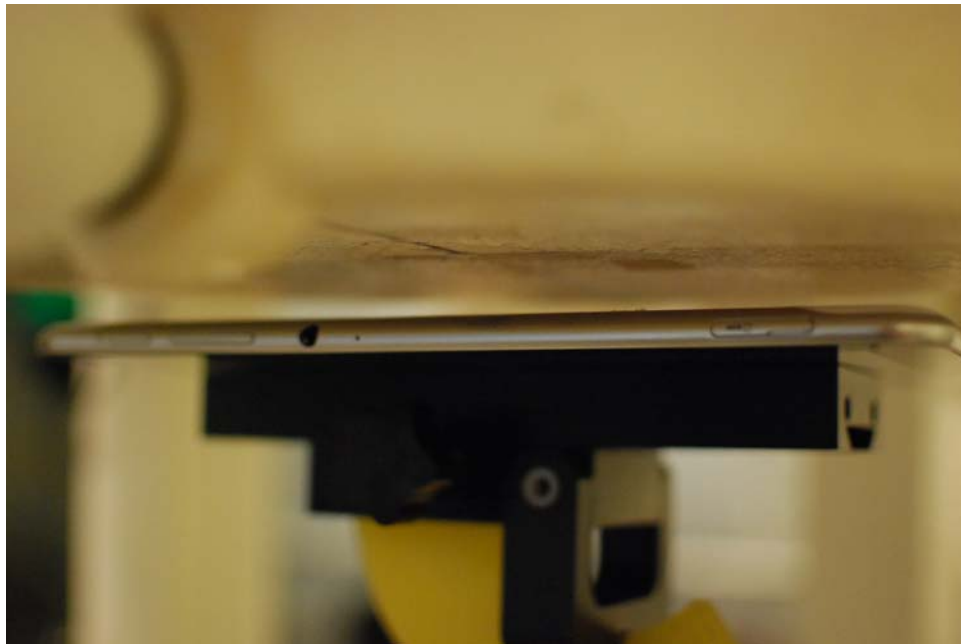
SAR Test Setup Photo 2: Back at 1.0 cm
