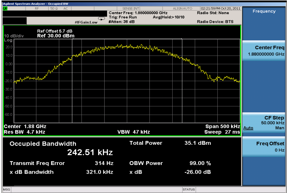
Plot 7-27. Occupied Bandwidth Plot (PCS GSM Mode – Ch. 661)
