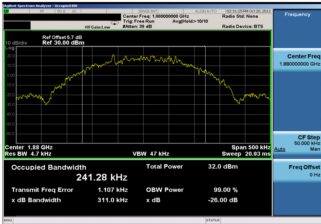
Plot 7-32. Occupied Bandwidth Plot (EDGE1900 Mode – Ch. 661)
