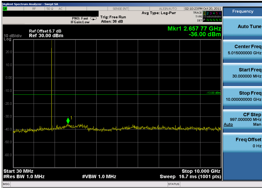
Plot 7-25. Conducted Spurious Plot (PCS GSM Mode – Ch. 661)
