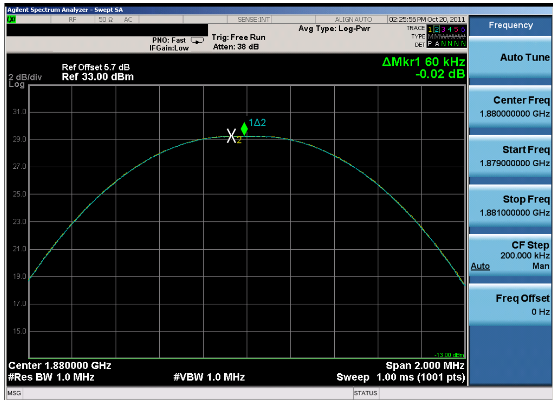
Plot 7-28. Peak-Average Ratio Plot (PCS GSM Mode – Ch. 661)
