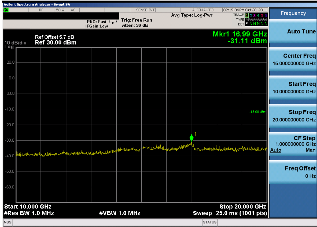
Plot 7-23. Conducted Spurious Plot (PCS GSM Mode – Ch. 512)
