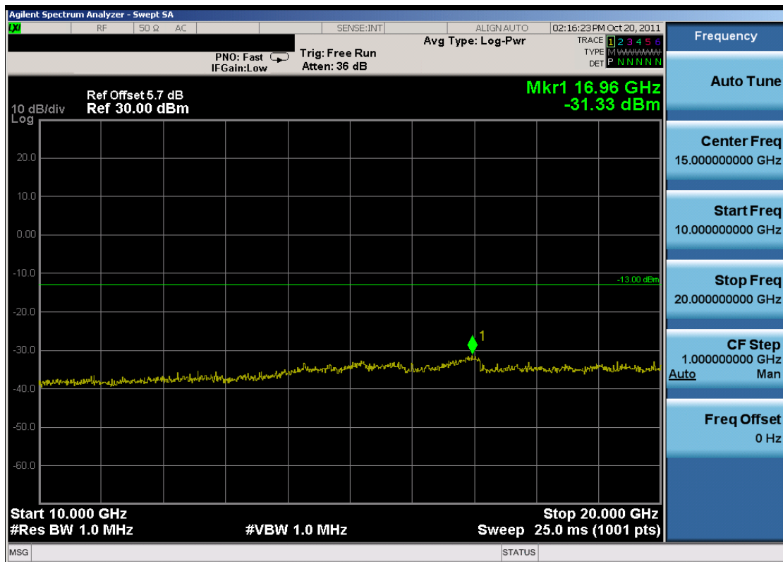
Plot 7-30. Conducted Spurious Plot (PCS GSM Mode – Ch. 810)
