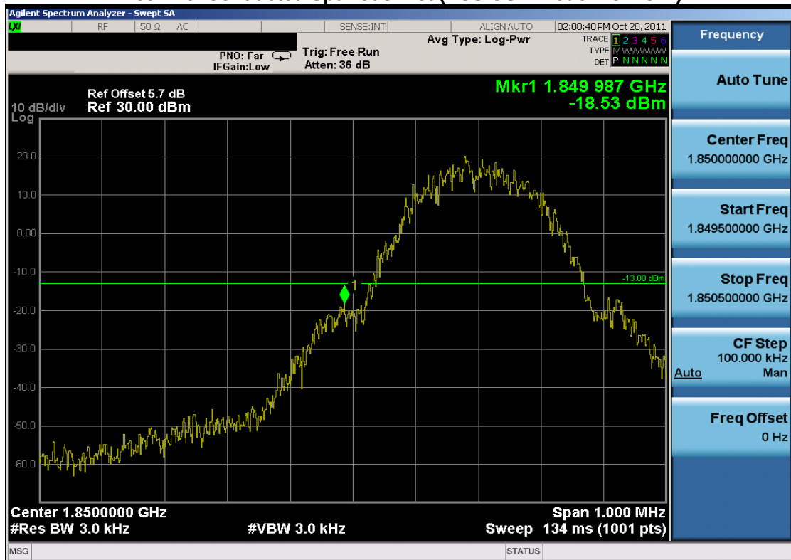
Plot 7-24. Band Edge Plot (PCS GSM Mode – Ch. 512)
