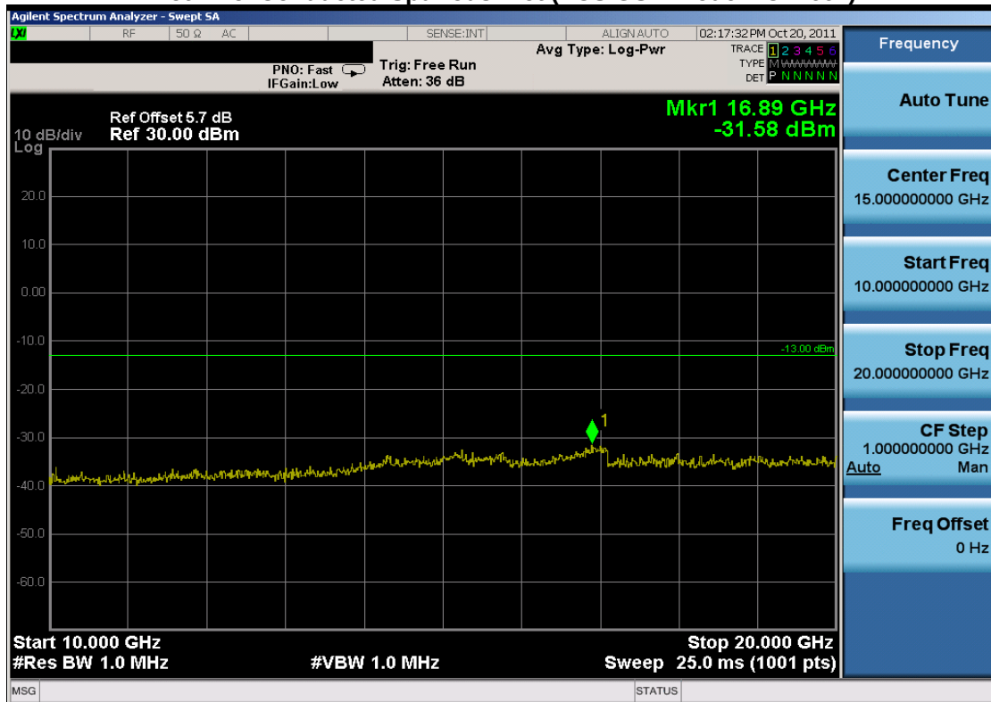
Plot 7-26. Conducted Spurious Plot (PCS GSM Mode – Ch. 661)
