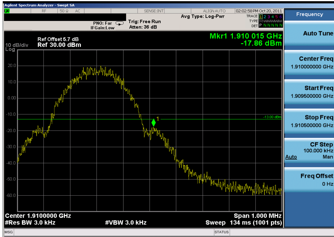
Plot 7-31. Band Edge Plot (PCS GSM Mode – Ch. 810)
