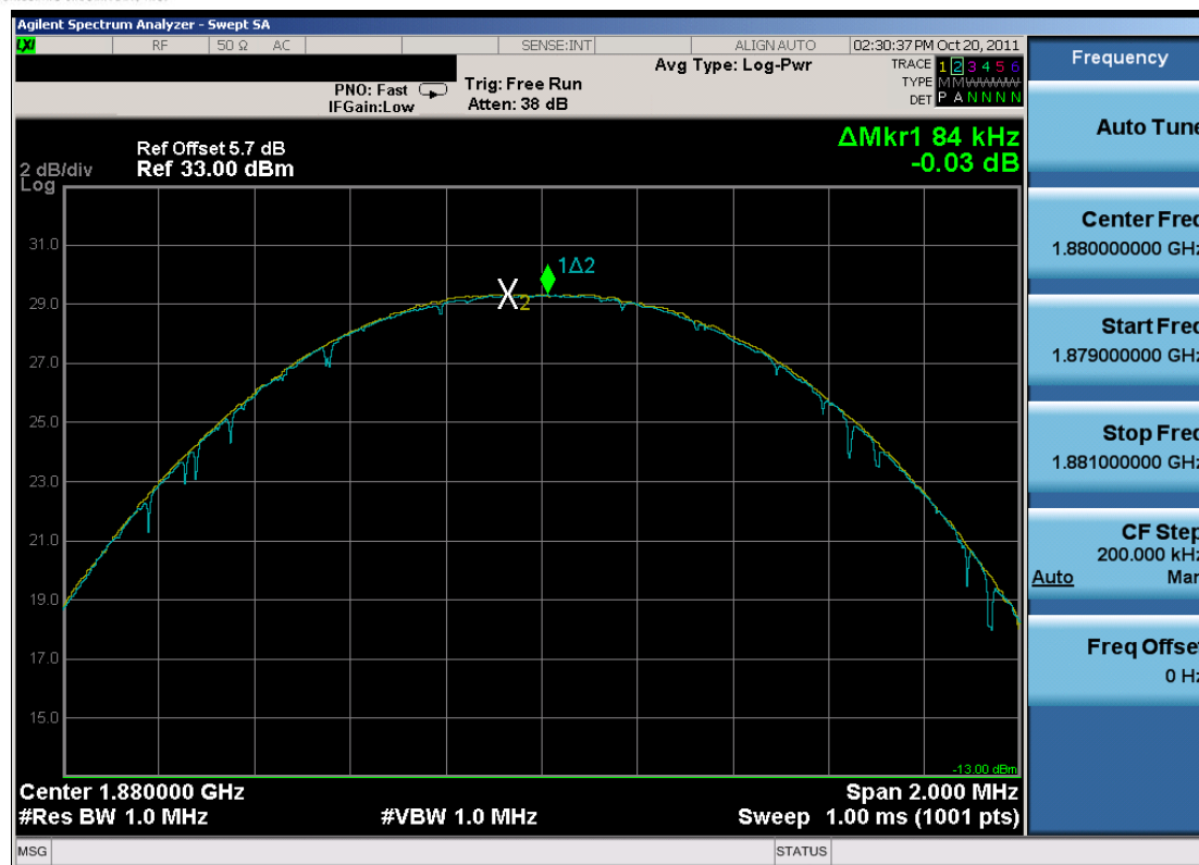
Plot 7-33. Peak-Average Ratio Plot (EDGE1900 Mode – Ch. 661)
