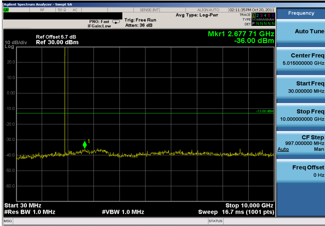
Plot 7-29. Conducted Spurious Plot (PCS GSM Mode – Ch. 810)
