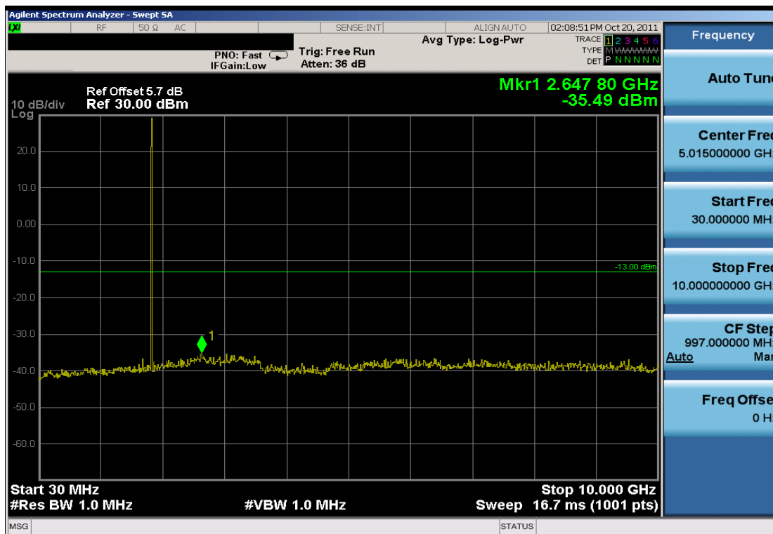
Plot 7-22. Conducted Spurious Plot (PCS GSM Mode – Ch. 512)
