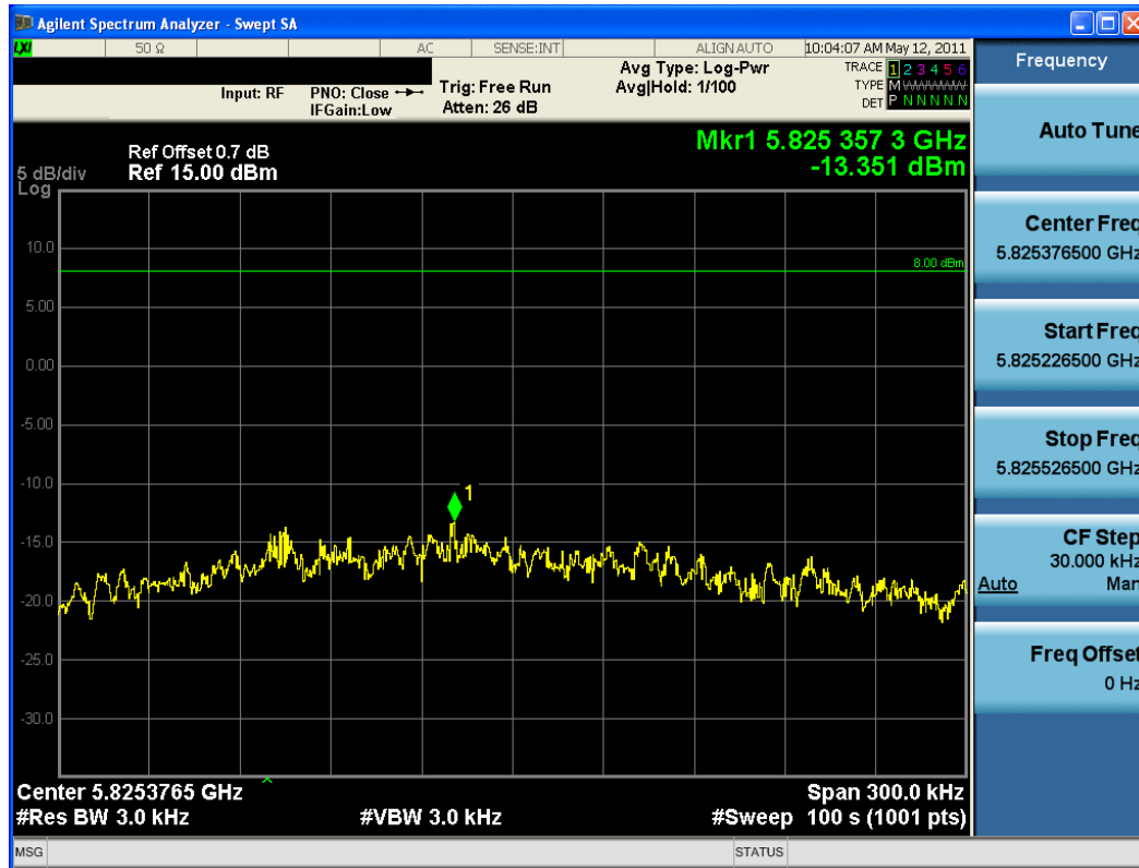
Plot 6-30. Power Spectral Density Plot (802.11n (5.8GHz) – Ch. 165)
