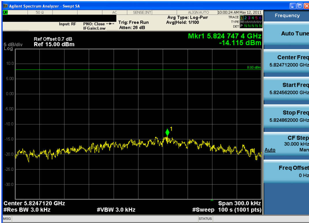
Plot 6-24. Power Spectral Density Plot (802.11a – Ch. 165)
