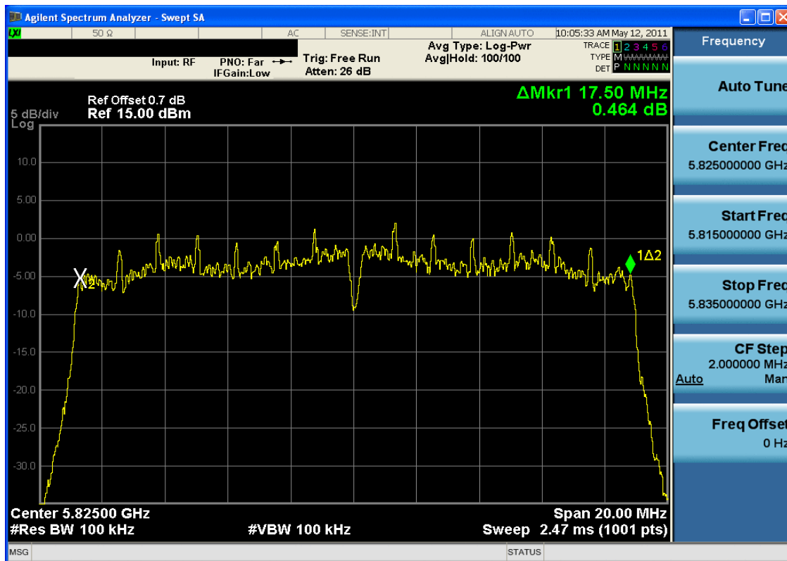
Plot 6-15. 6dB Bandwidth Plot (802.11n (5.8GHz) – Ch. 165)
