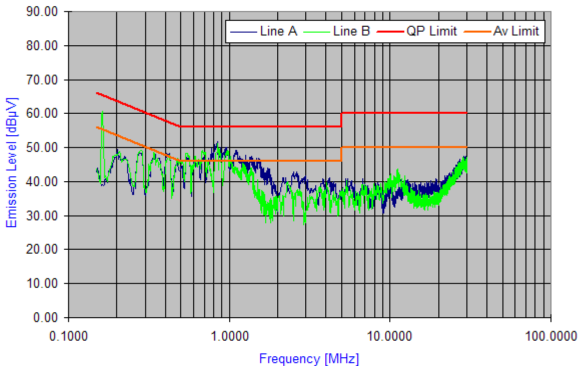
Plot 6-53. Line Conducted Plot with 802.11b
