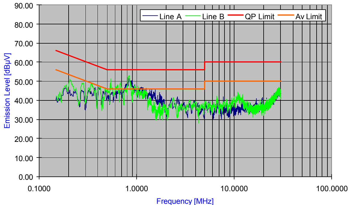
Plot 6-56. Line Conducted Plot with 802.11n (2.4GHz)
