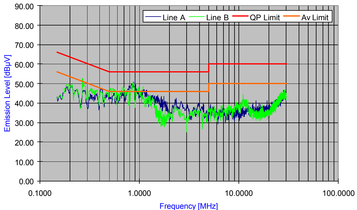
Plot 6-55. Line Conducted Plot with 802.11a
