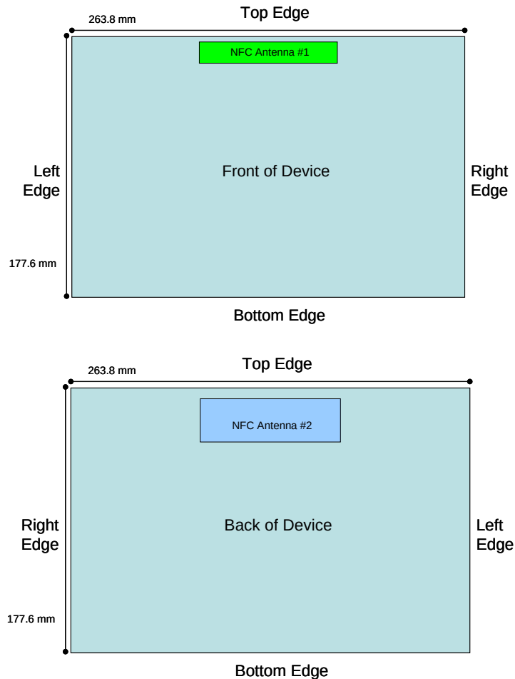
Figure 1-1 NFC Antenna Locations
