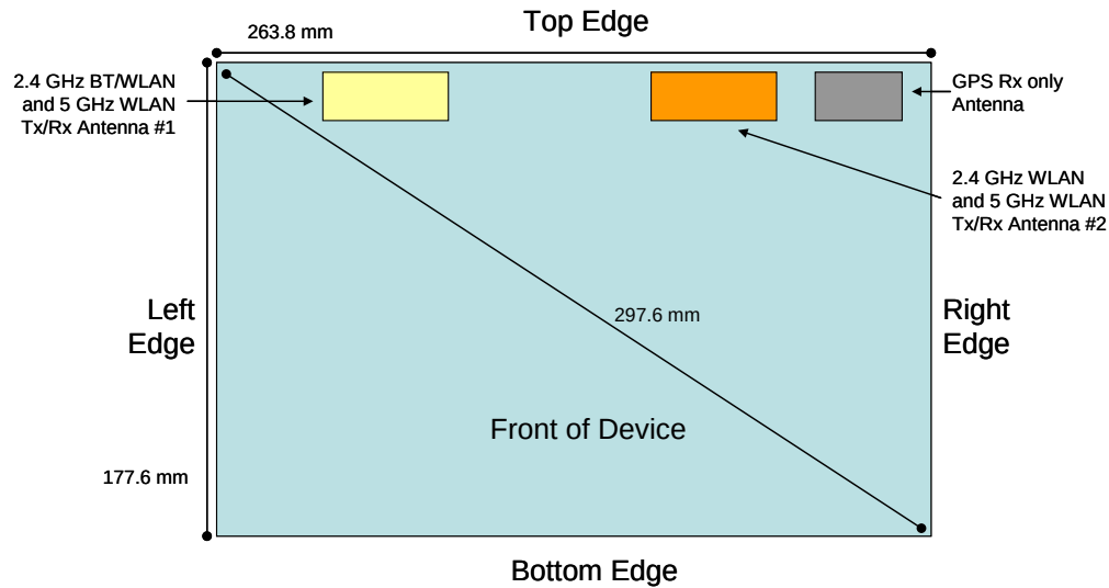
Figure 1-2 DUT Antenna Locations
