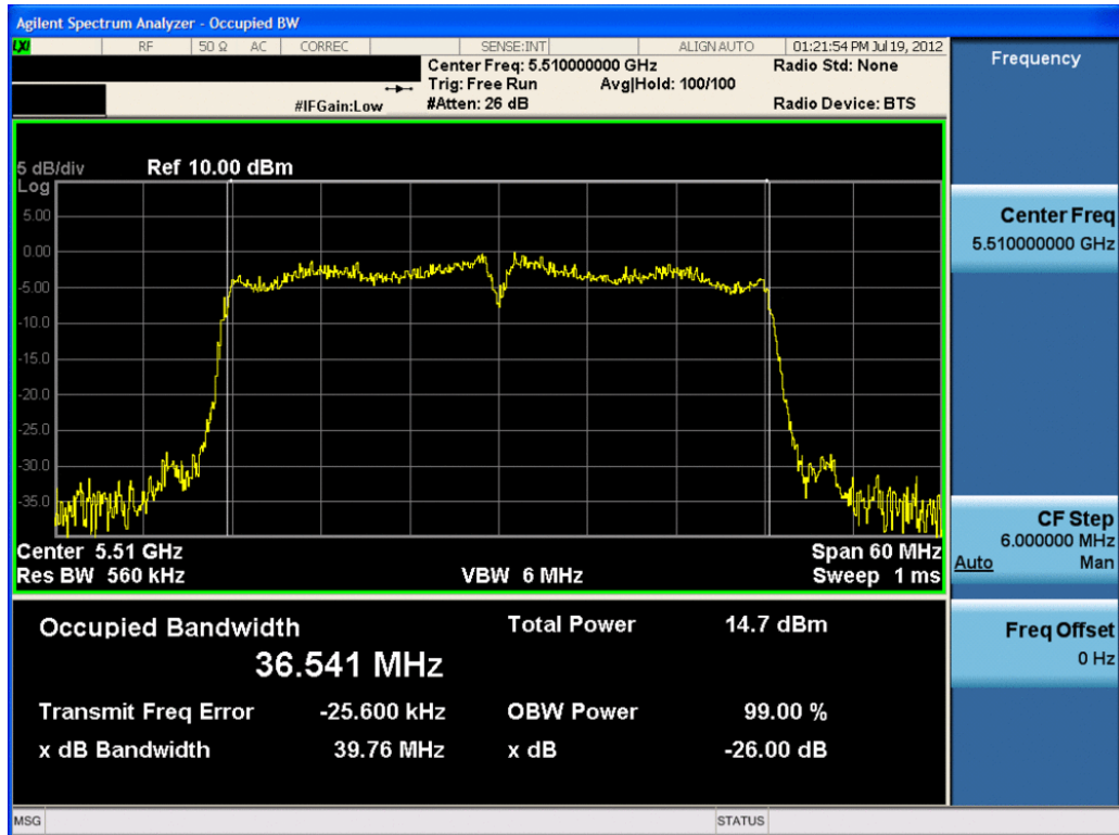
Plot 6-48. 26dB Bandwidth Plot (40MHz BW 802.11n (UNII Band 3) – Ch. 102) – Chain B
