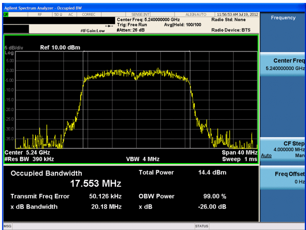
Plot 6-6. 26dB Bandwidth Plot (20MHz BW 802.11n (UNII Band 1) – Ch. 48) – Chain A
