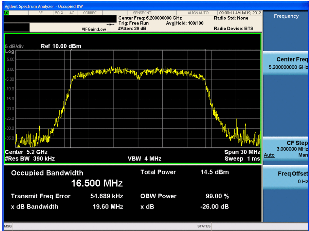
Plot 6-27. 26dB Bandwidth Plot (802.11a (UNII Band 1) – Ch. 40) – Chain B
