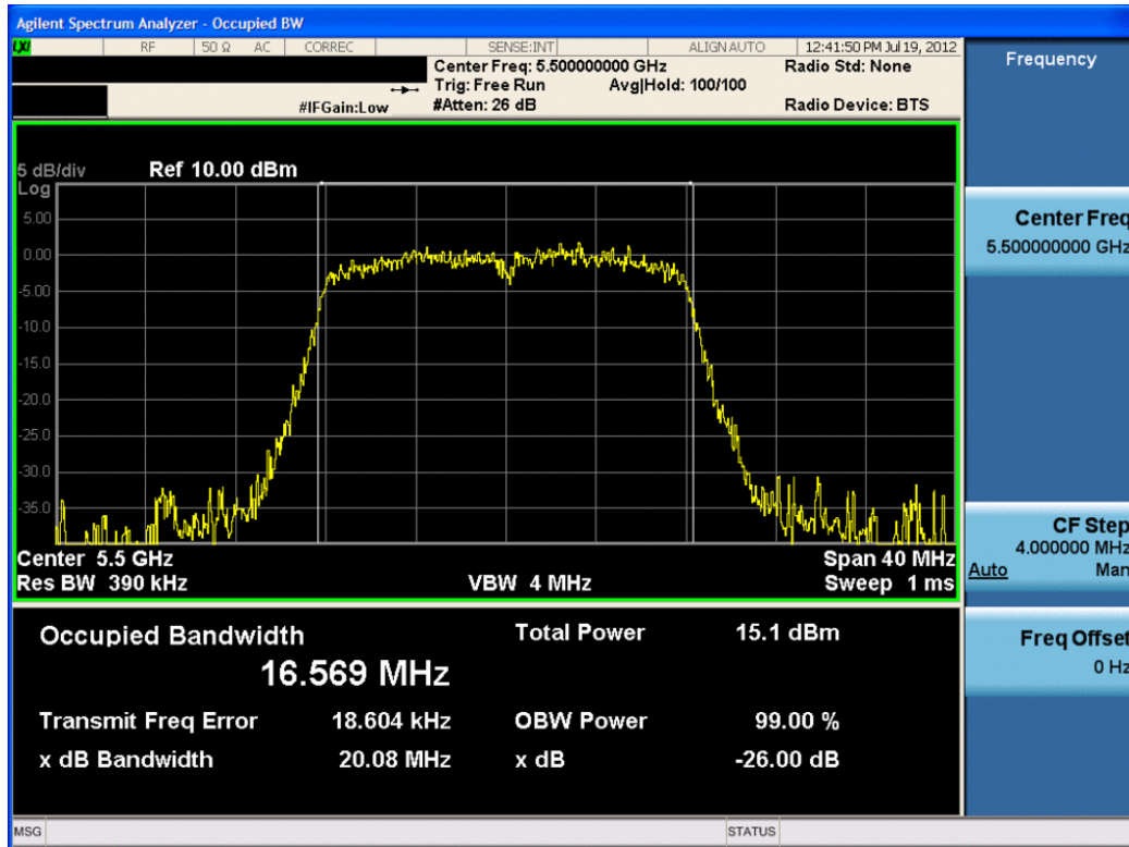
Plot 6-17. 26dB Bandwidth Plot (802.11a (UNII Band 3) – Ch. 100) – Chain A
