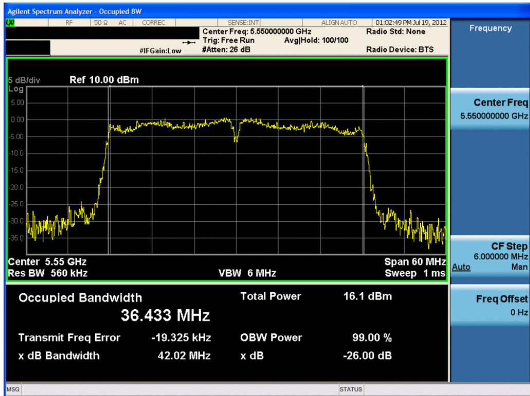
Plot 6-24. 26dB Bandwidth Plot (40MHz BW 802.11n (UNII Band 3) – Ch. 110) – Chain A
