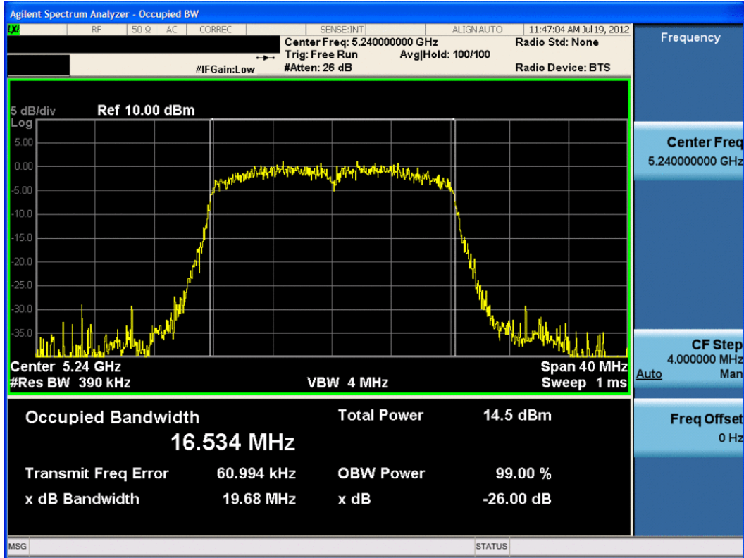
Plot 6-3. 26dB Bandwidth Plot (802.11a (UNII Band 1) – Ch. 48) – Chain A
