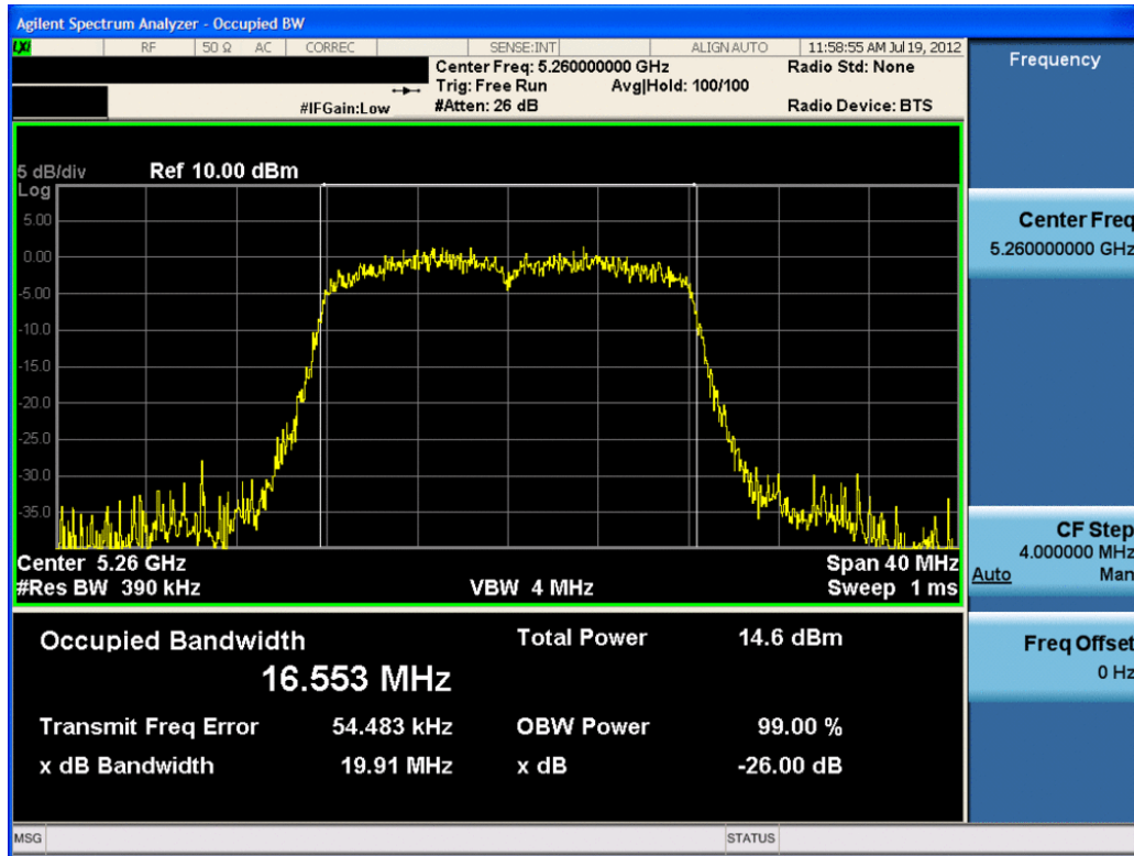
Plot 6-9. 26dB Bandwidth Plot (802.11a (UNII Band 2) – Ch. 52) – Chain A
