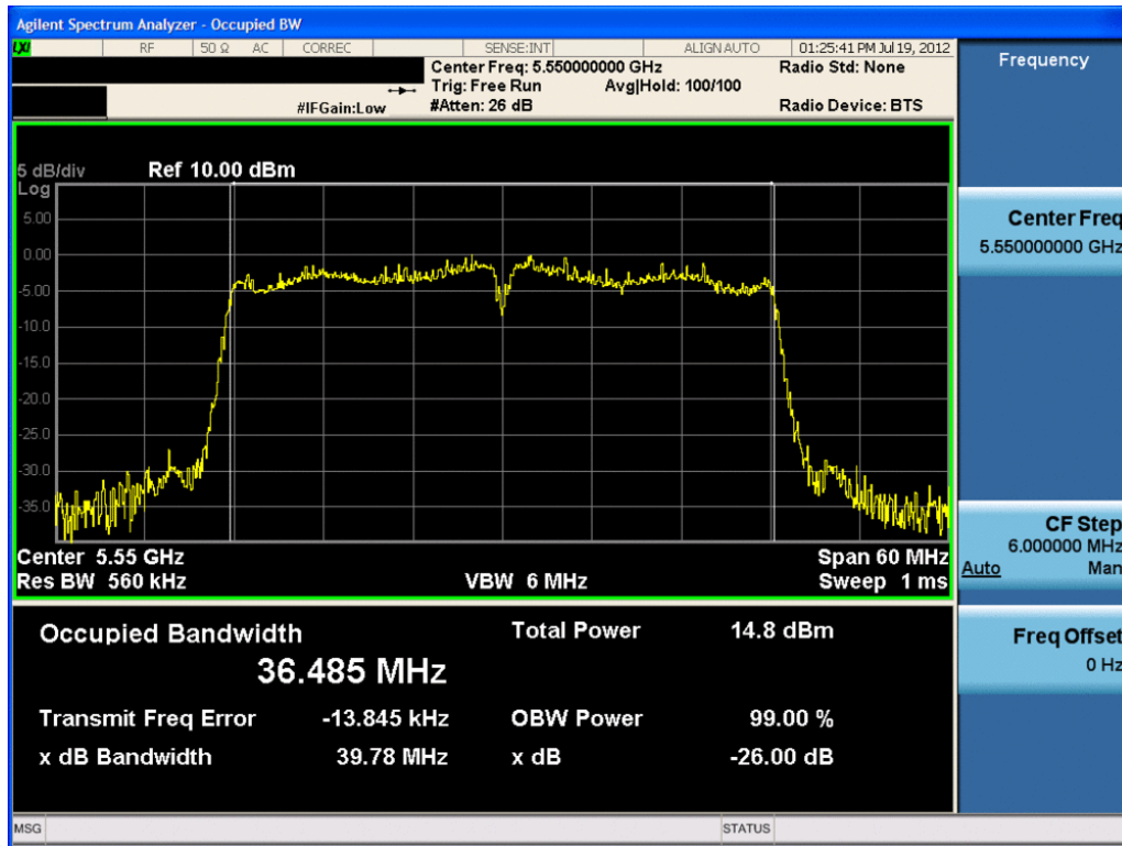
Plot 6-49. 26dB Bandwidth Plot (40MHz BW 802.11n (UNII Band 3) – Ch. 110) – Chain B
