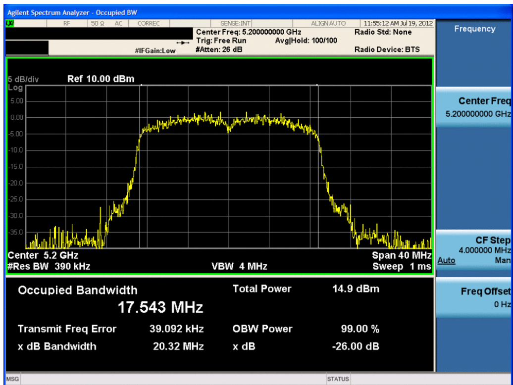
Plot 6-5. 26dB Bandwidth Plot (20MHz BW 802.11n (UNII Band 1) – Ch. 40) – Chain A
