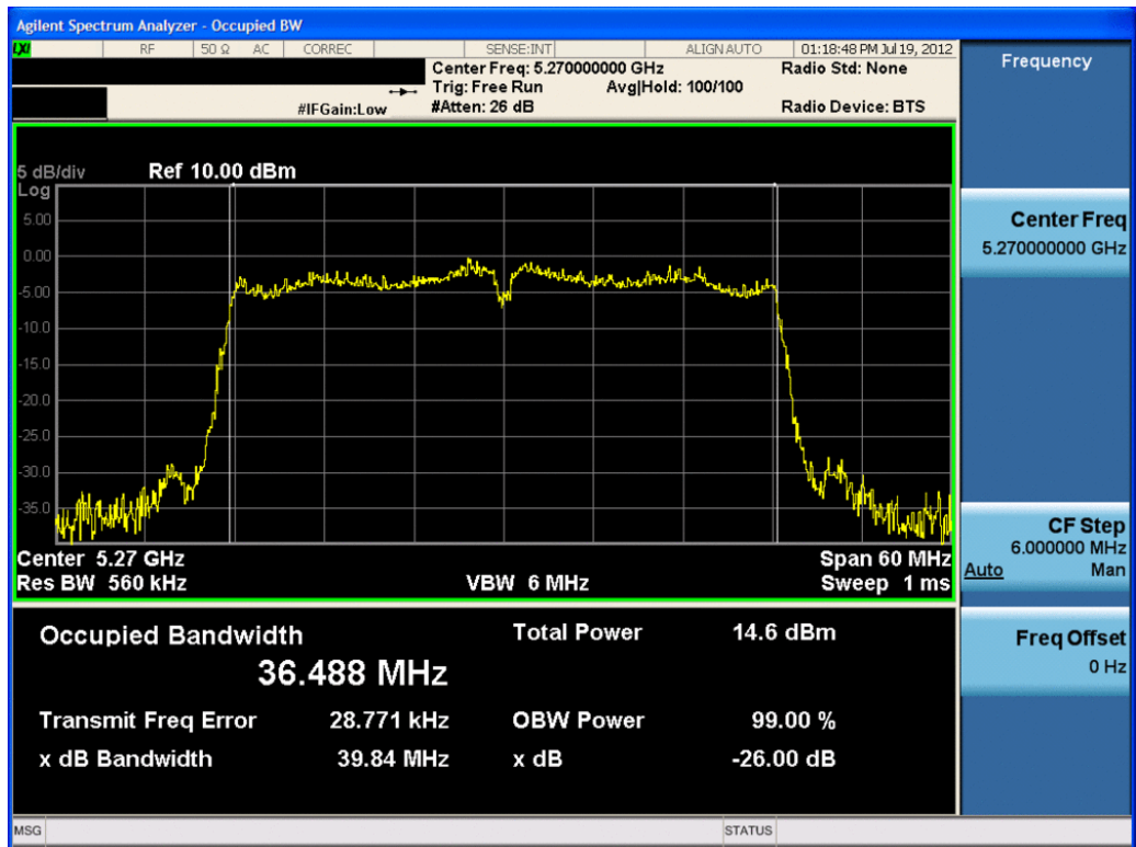
Plot 6-40. 26dB Bandwidth Plot (40MHz BW 802.11a/n (UNII Band 2) – Ch. 54) – Chain B
