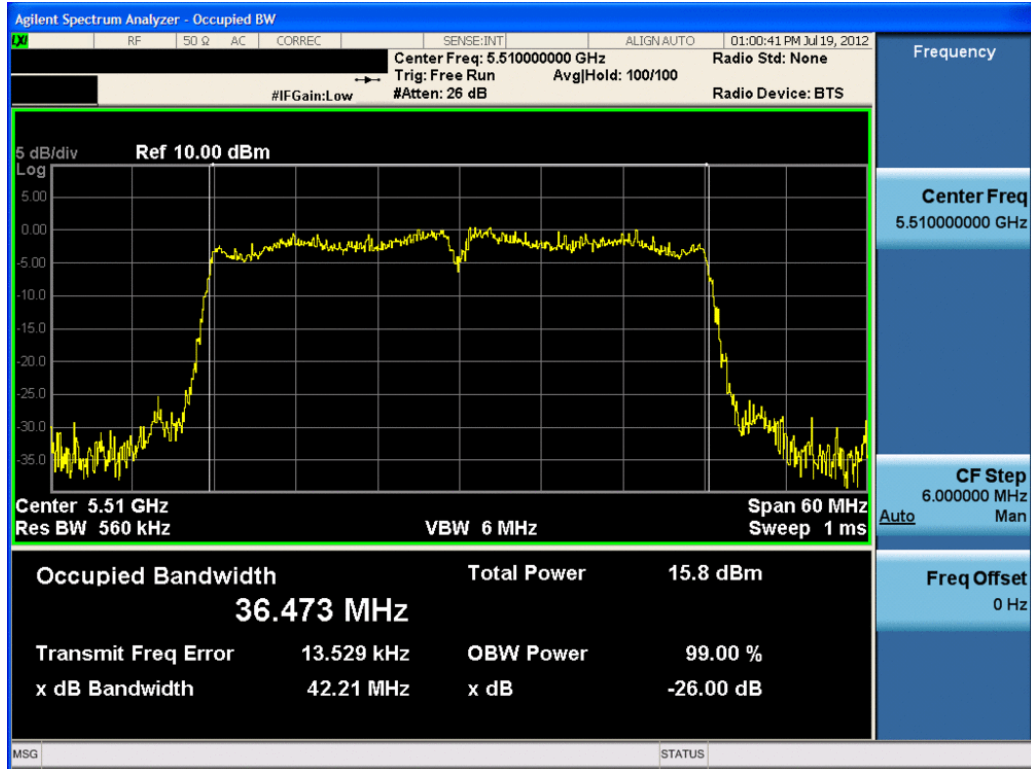
Plot 6-23. 26dB Bandwidth Plot (40MHz BW 802.11n (UNII Band 3) – Ch. 102) – Chain A
