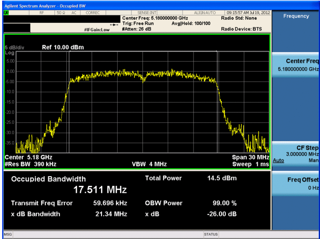
Plot 6-29. 26dB Bandwidth Plot (20MHz BW 802.11n (UNII Band 1) – Ch. 36) – Chain B
