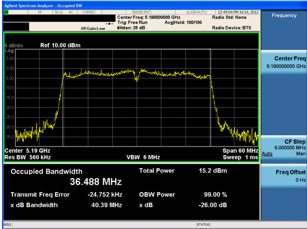
Plot 6-7. 26dB Bandwidth Plot (40MHz BW 802.11n (UNII Band 1) – Ch. 38) – Chain A
