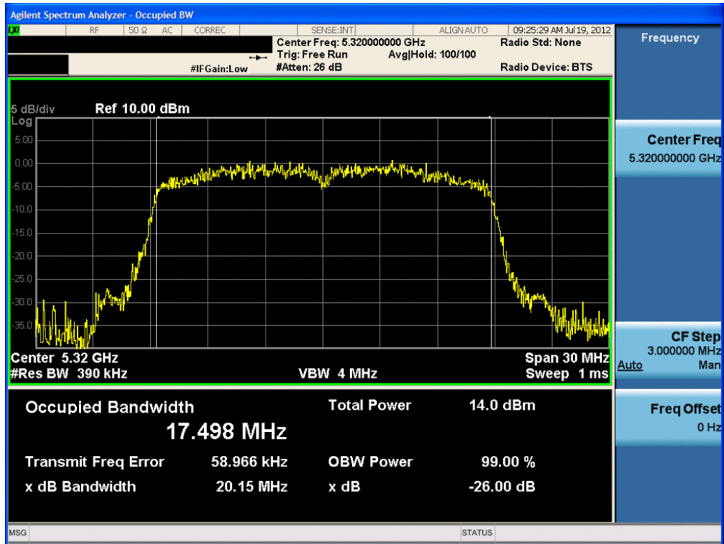
Plot 6-39. 26dB Bandwidth Plot (20MHz BW 802.11n (UNII Band 2) – Ch. 64) – Chain B
