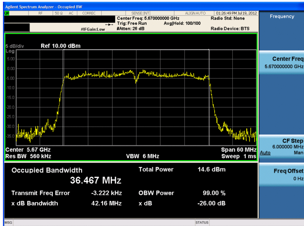
Plot 6-50. 26dB Bandwidth Plot (40MHz BW 802.11n (UNII Band 3) – Ch. 134) – Chain B
