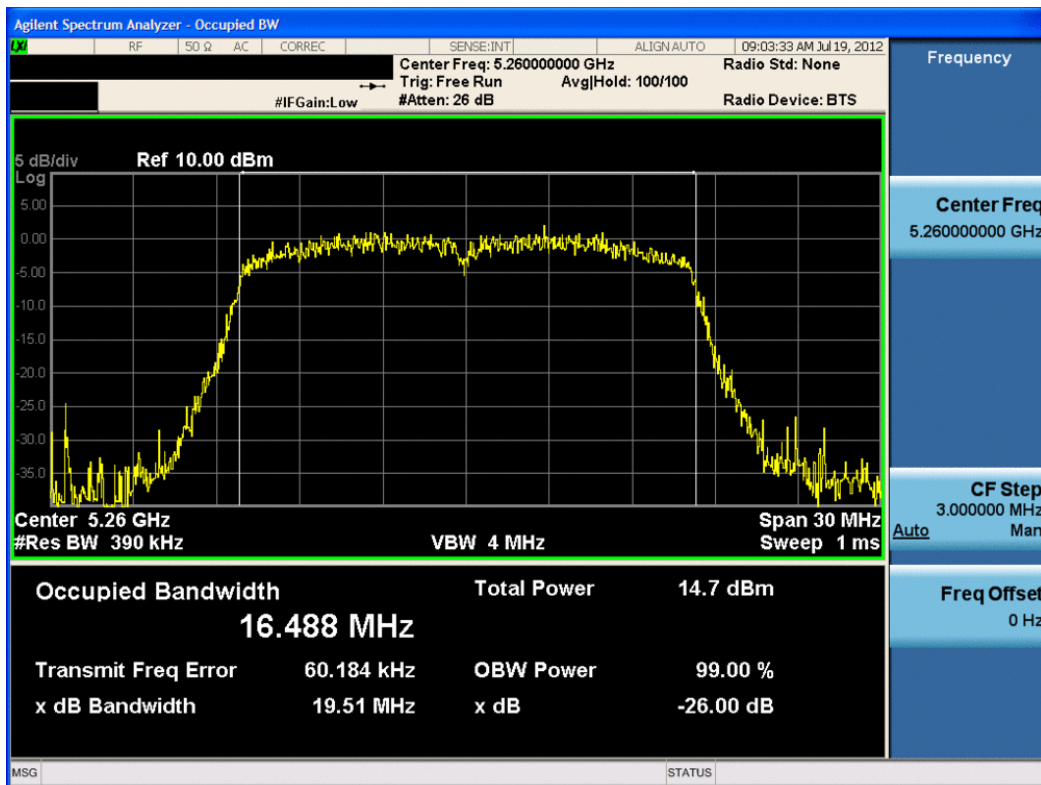
Plot 6-34. 26dB Bandwidth Plot (802.11a (UNII Band 2) – Ch. 52) – Chain B
