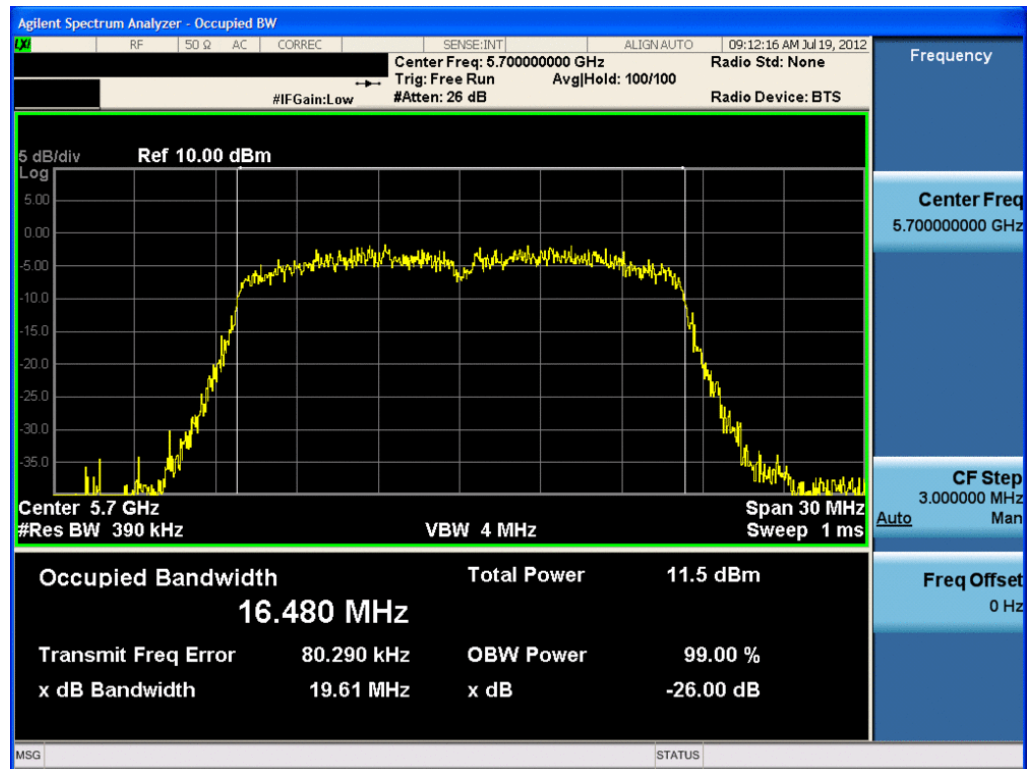
Plot 6-44. 26dB Bandwidth Plot (802.11a (UNII Band 3) – Ch. 140) – Chain B
