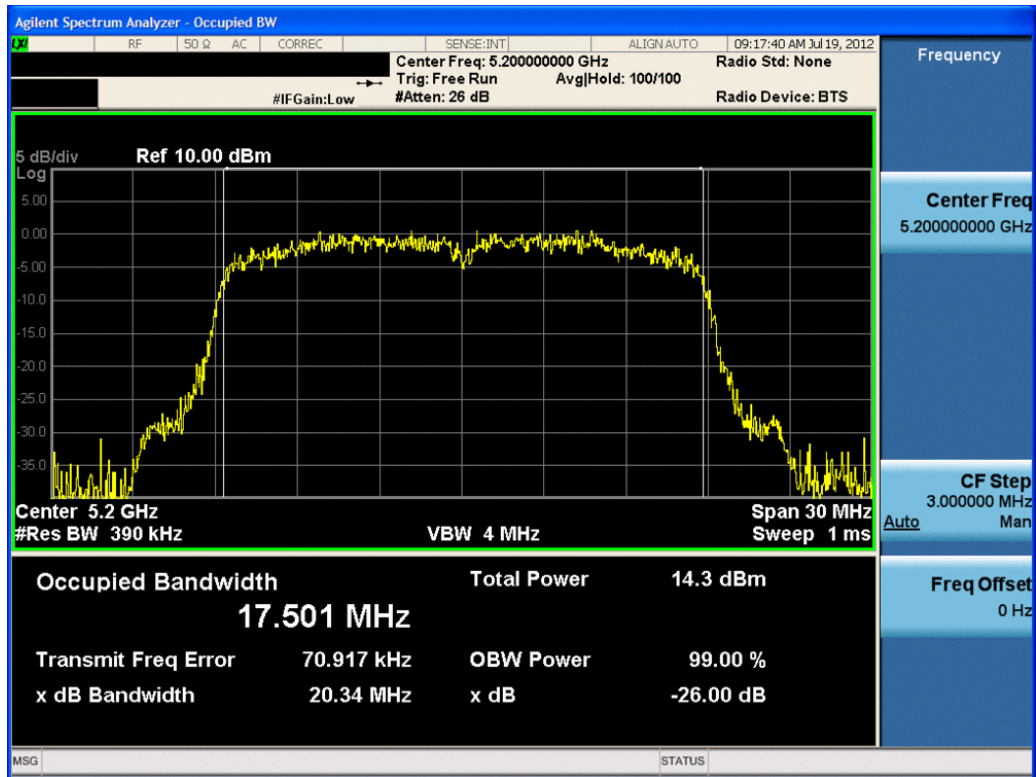
Plot 6-30. 26dB Bandwidth Plot (20MHz BW 802.11n (UNII Band 1) – Ch. 40) – Chain B
