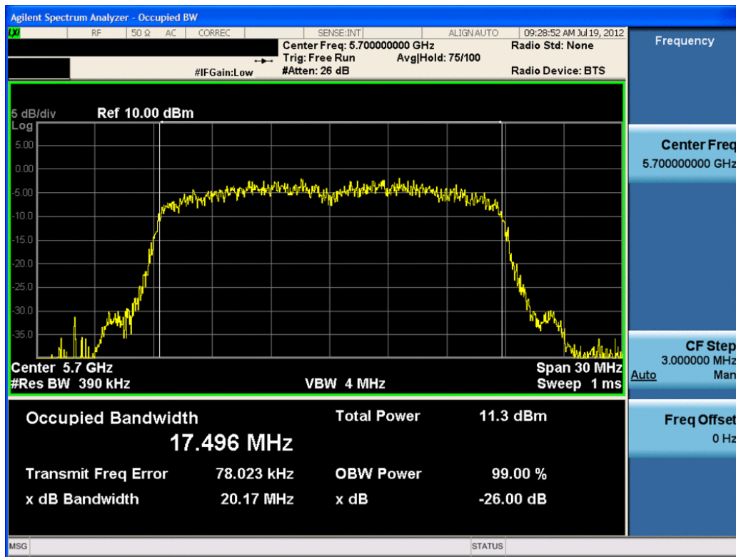
Plot 6-47. 26dB Bandwidth Plot (20MHz BW 802.11n (UNII Band 3) – Ch. 140) – Chain B
