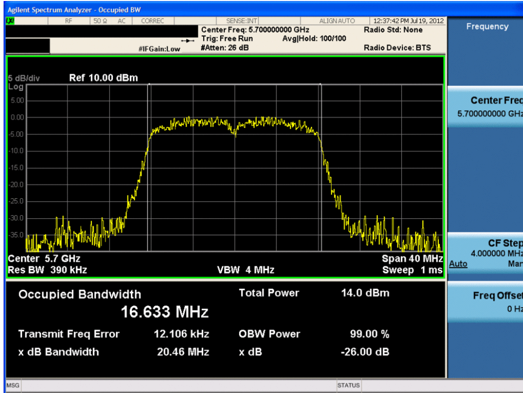
Plot 6-19. 26dB Bandwidth Plot (802.11a (UNII Band 3) – Ch. 140) – Chain A
