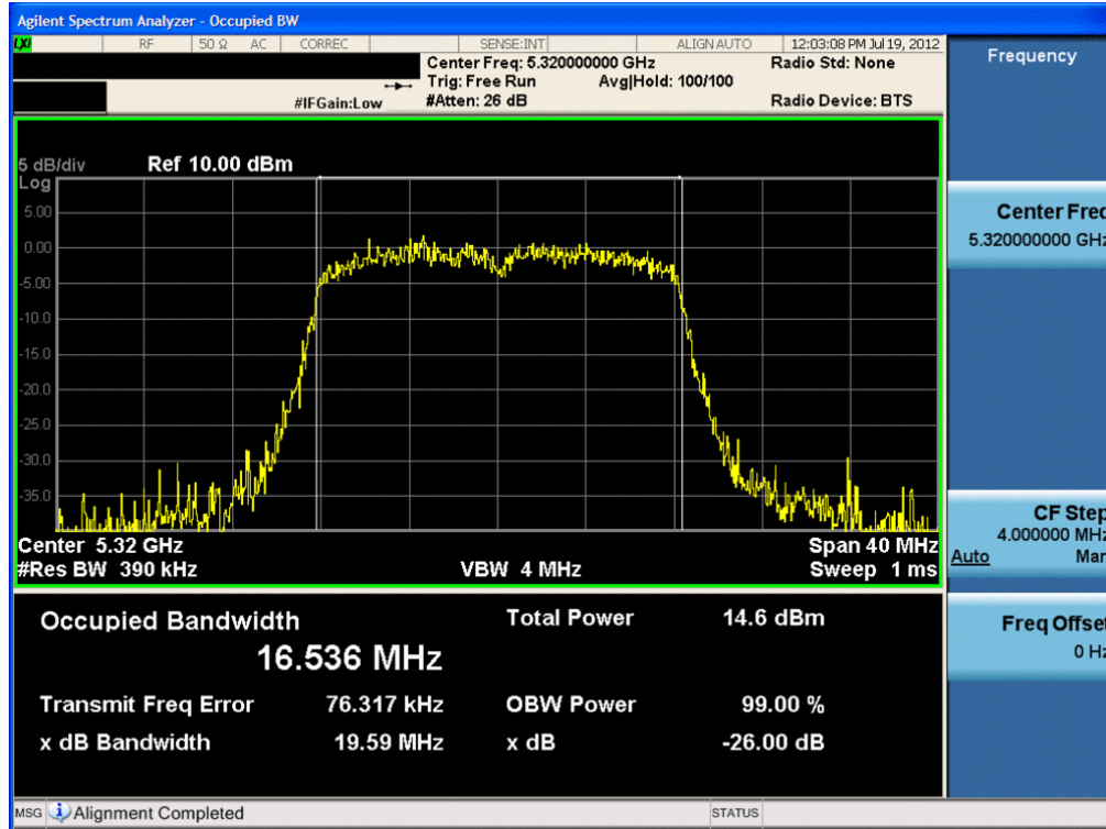
Plot 6-11. 26dB Bandwidth Plot (802.11a (UNII Band 2) – Ch. 64) – Chain A
