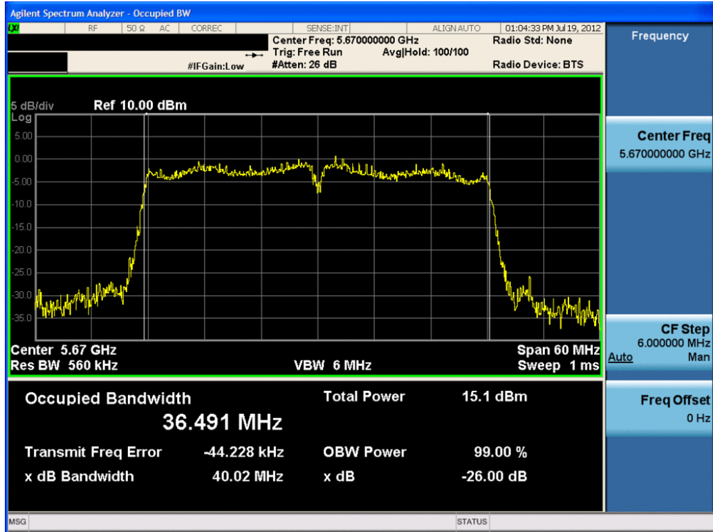
Plot 6-25. 26dB Bandwidth Plot (40MHz BW 802.11n (UNII Band 3) – Ch. 134) – Chain A
