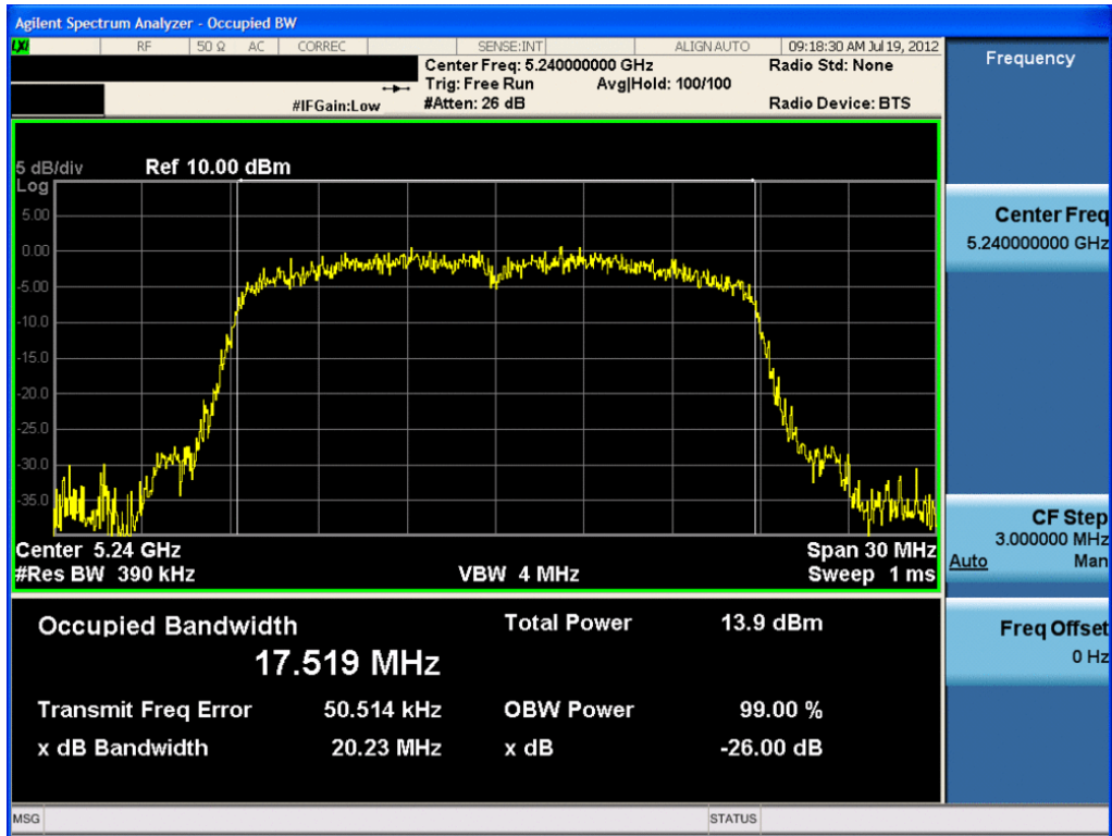
Plot 6-31. 26dB Bandwidth Plot (20MHz BW 802.11n (UNII Band 1) – Ch. 48) – Chain B
