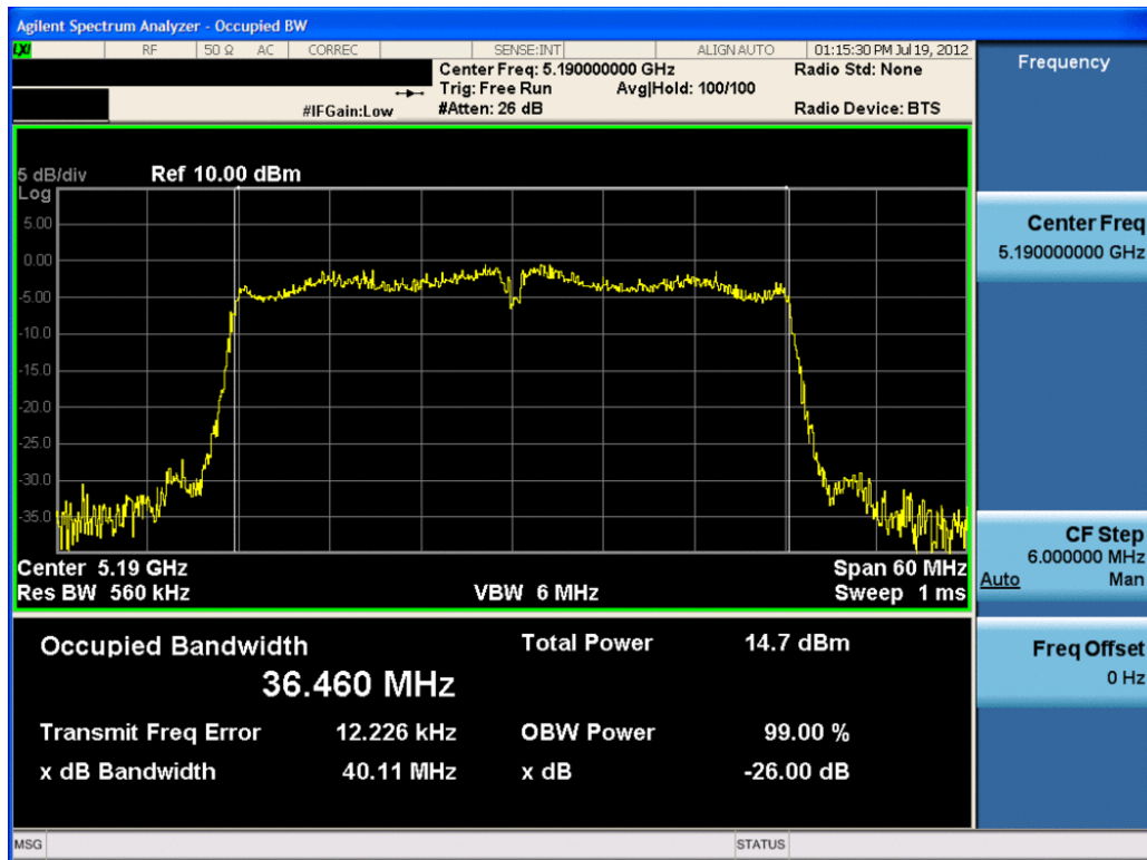
Plot 6-32. 26dB Bandwidth Plot (40MHz BW 802.11n (UNII Band 1) – Ch. 38) – Chain B
