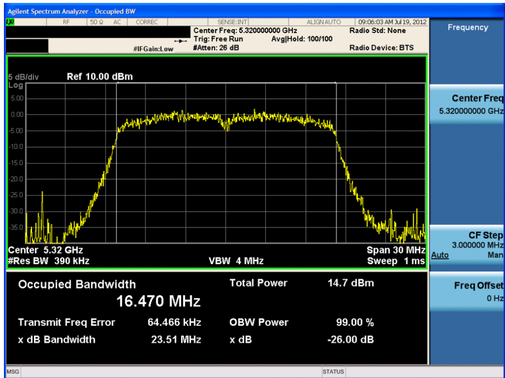
Plot 6-36. 26dB Bandwidth Plot (802.11a (UNII Band 2) - Ch. 64) - Chain B
