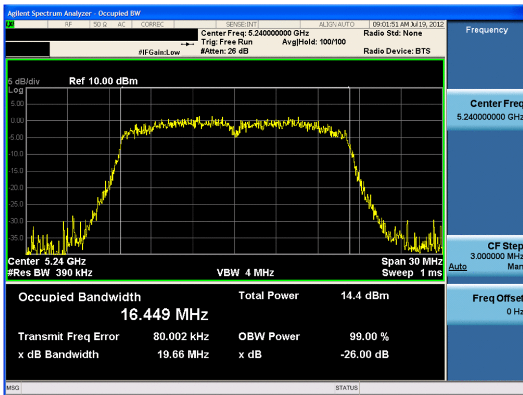
Plot 6-28. 26dB Bandwidth Plot (802.11a (UNII Band 1) – Ch. 48) – Chain B
