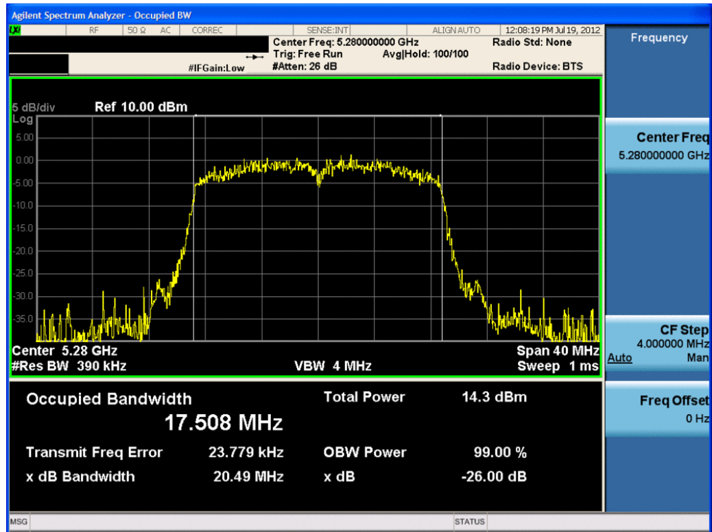
Plot 6-13. 26dB Bandwidth Plot (20MHz BW 802.11n (UNII Band 2) – Ch. 56) – Chain A
