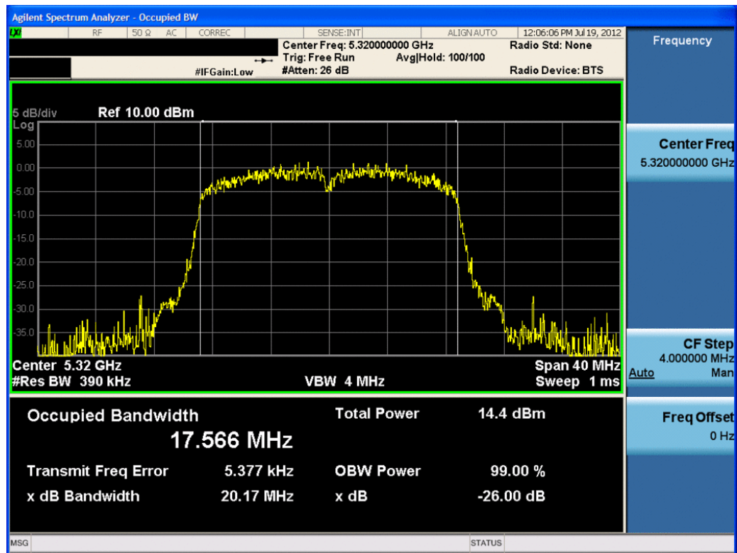
Plot 6-14. 26dB Bandwidth Plot (20MHz BW 802.11n (UNII Band 2) – Ch. 64) – Chain A
