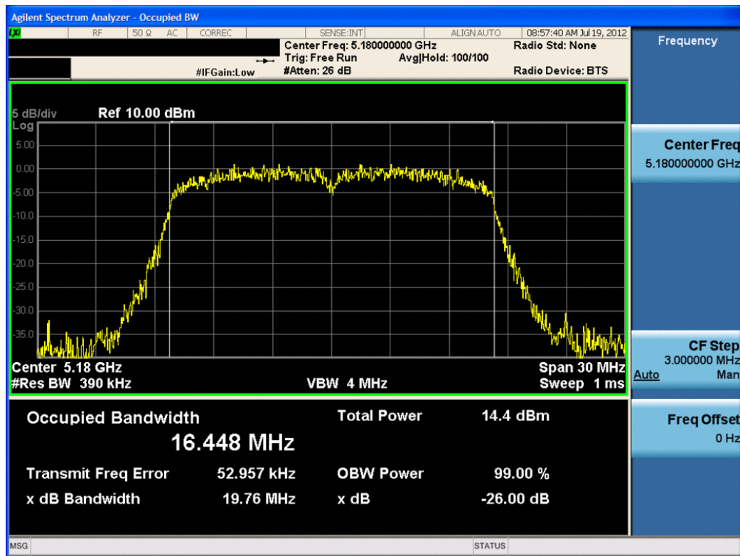
Plot 6-26. 26dB Bandwidth Plot (802.11a (UNII Band 1) – Ch. 36) – Chain B
