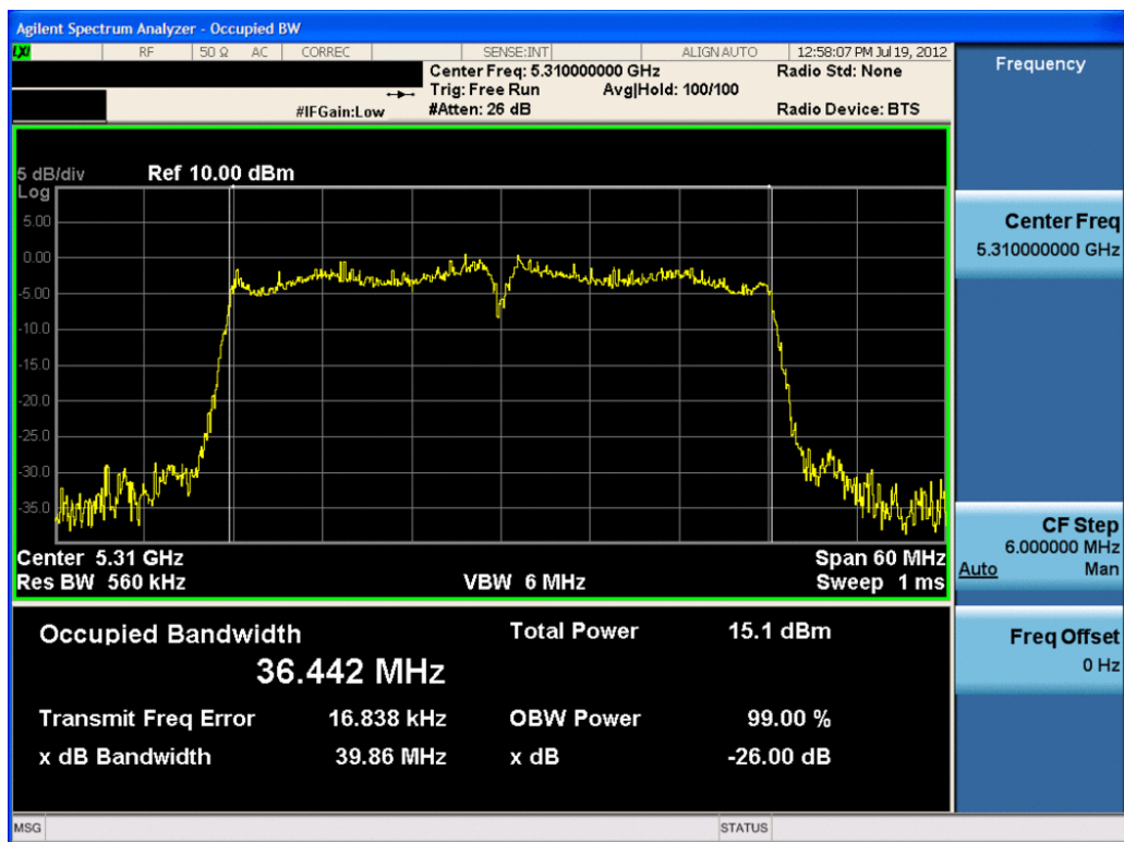
Plot 6-16. 26dB Bandwidth Plot (40MHz BW 802.11n (UNII Band 2) – Ch. 62) – Chain A
