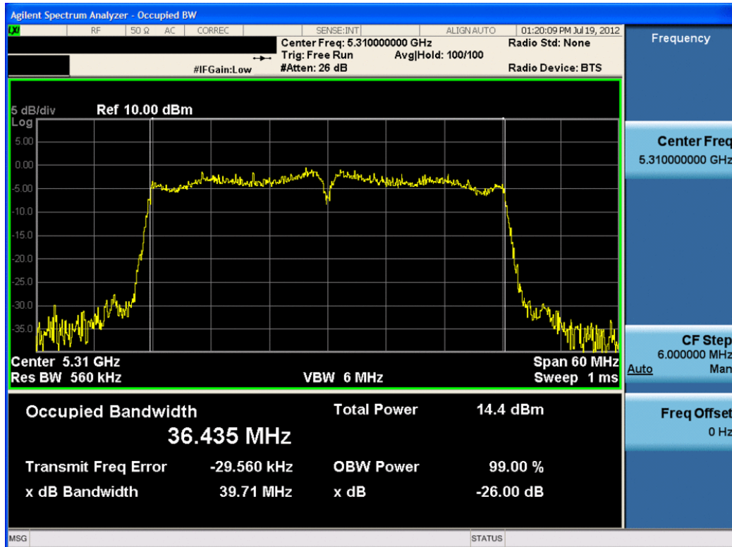
Plot 6-41. 26dB Bandwidth Plot (40MHz BW 802.11n (UNII Band 2) – Ch. 62) – Chain B
