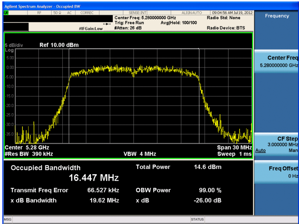
Plot 6-35. 26dB Bandwidth Plot (802.11a (UNII Band 2) - Ch. 56) - Chain B
