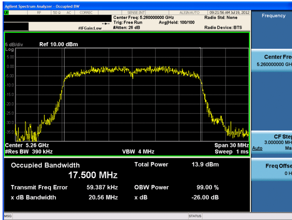
Plot 6-37. 26dB Bandwidth Plot (20MHz BW 802.11n (UNII Band 2) – Ch. 52) – Chain B
