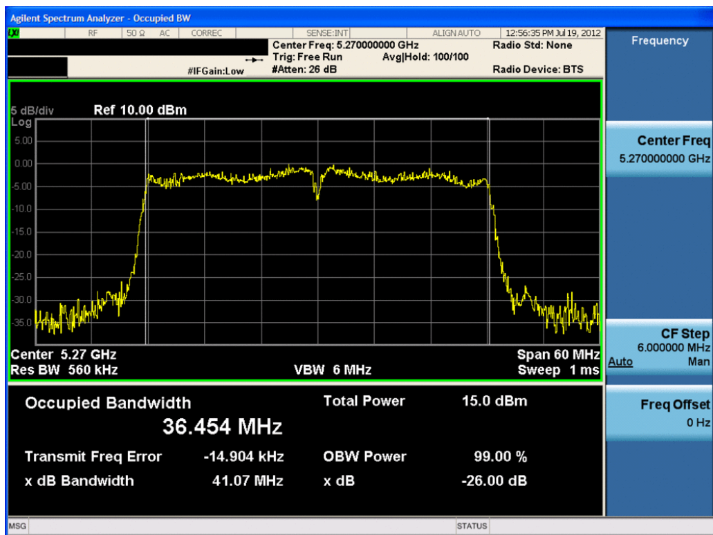
Plot 6-15. 26dB Bandwidth Plot (40MHz BW 802.11n (UNII Band 2) – Ch. 54) – Chain A
