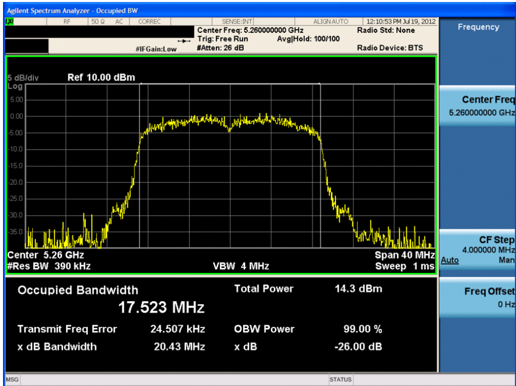
Plot 6-12. 26dB Bandwidth Plot (20MHz BW 802.11n (UNII Band 2) – Ch. 52) – Chain A
