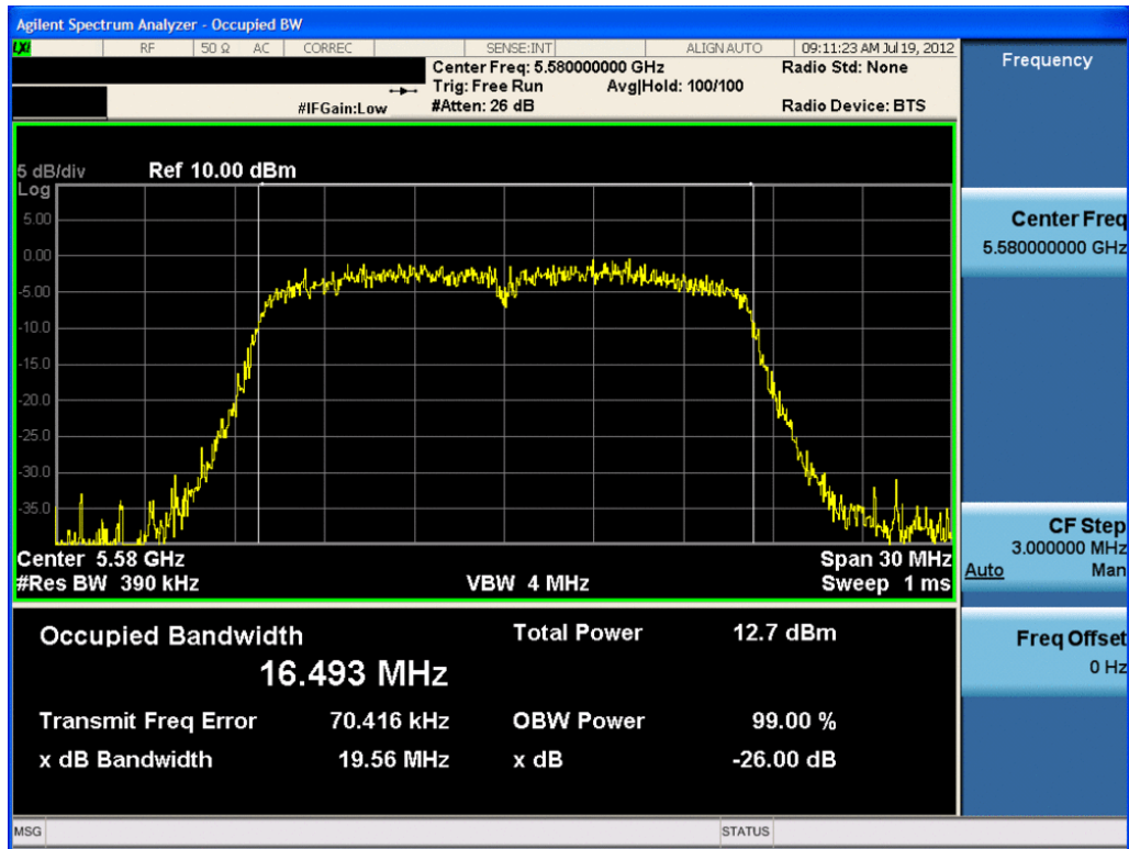
Plot 6-43. 26dB Bandwidth Plot (802.11a (UNII Band 3) – Ch. 116) – Chain B
