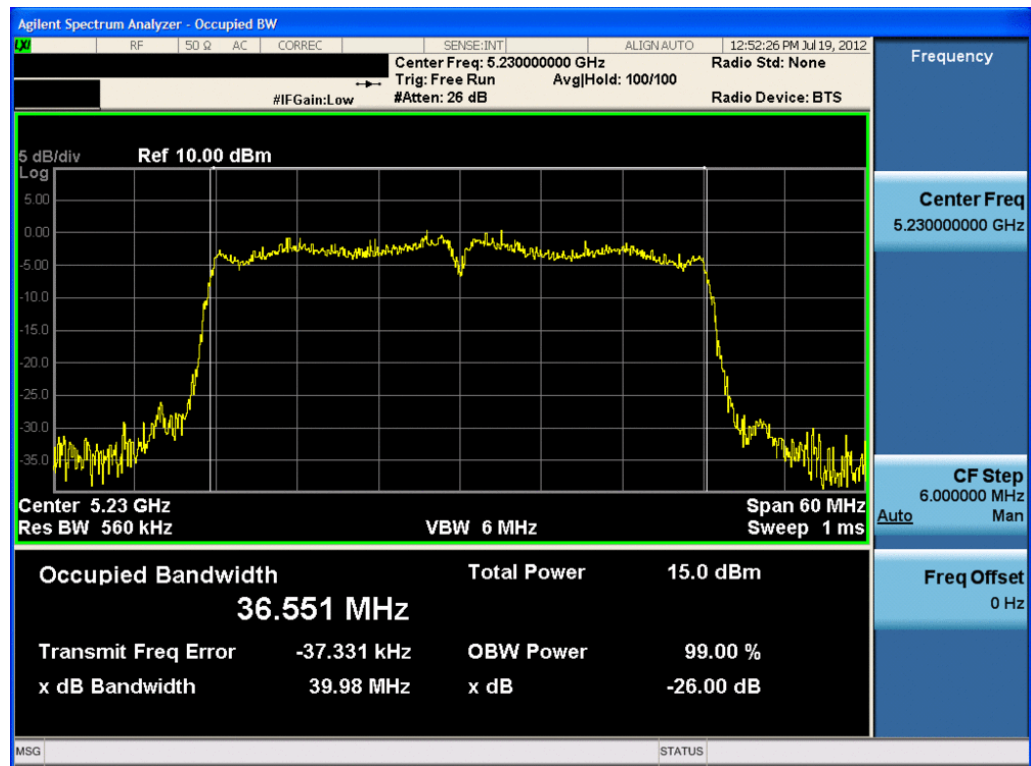
Plot 6-8. 26dB Bandwidth Plot (40MHz BW 802.11n (UNII Band 1) – Ch. 46) – Chain A
