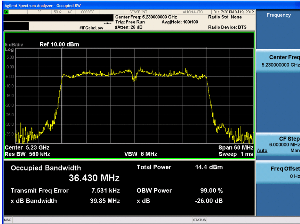
Plot 6-33. 26dB Bandwidth Plot (40MHz BW 802.11n (UNII Band 1) – Ch. 46) – Chain B
