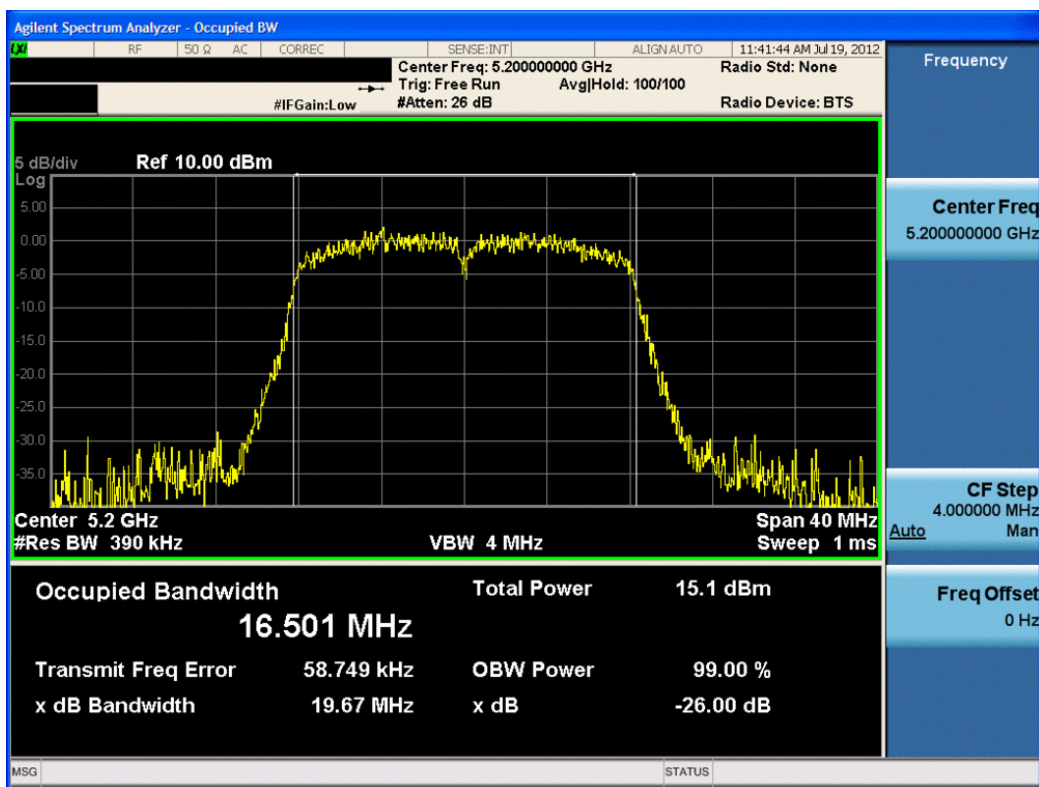
Plot 6-2. 26dB Bandwidth Plot (802.11a (UNII Band 1) – Ch. 40) – Chain A
