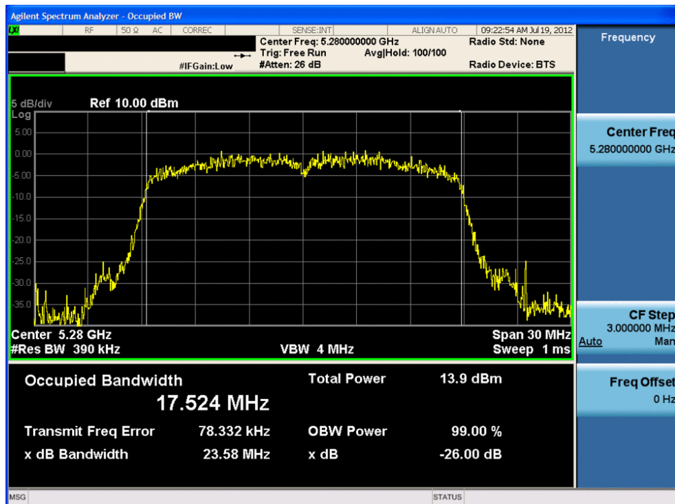
Plot 6-38. 26dB Bandwidth Plot (20MHz BW 802.11n (UNII Band 2) – Ch. 56) – Chain B
