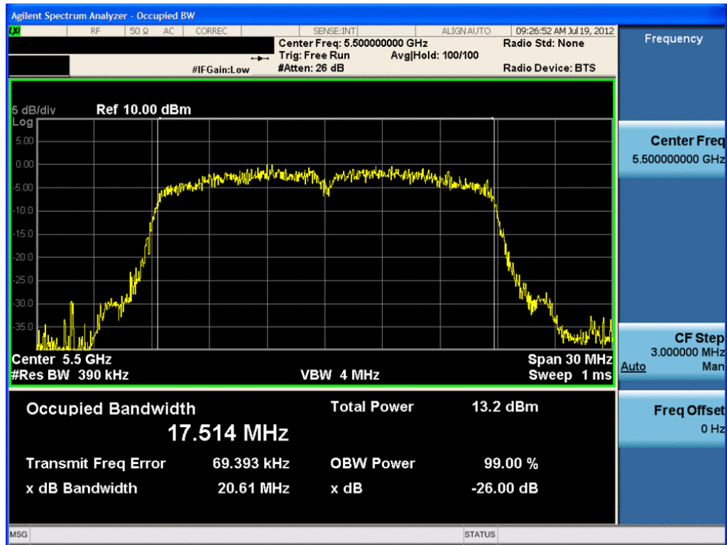
Plot 6-45. 26dB Bandwidth Plot (20MHz BW 802.11n (UNII Band 3) – Ch. 100) – Chain B
