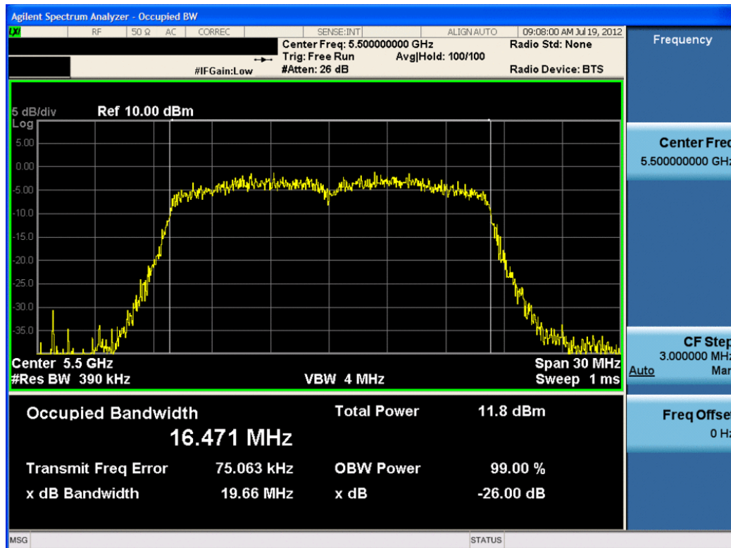
Plot 6-42. 26dB Bandwidth Plot (802.11a (UNII Band 3) – Ch. 100) – Chain B
