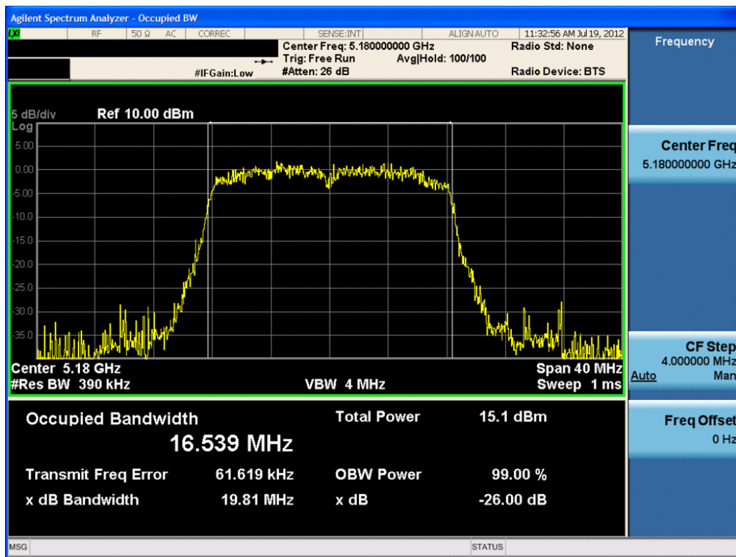
Plot 6-1. 26dB Bandwidth Plot (802.11a (UNII Band 1) – Ch. 36) – Chain A
