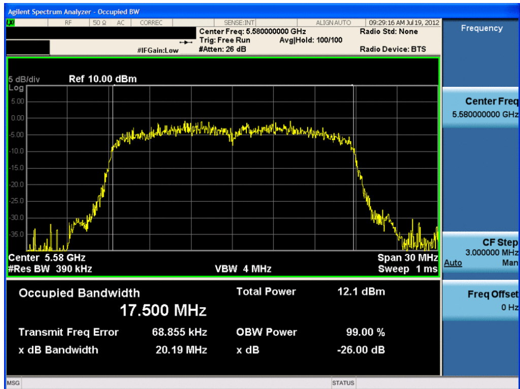
Plot 6-46. 26dB Bandwidth Plot (20MHz BW 802.11n (UNII Band 3) – Ch. 116) – Chain B
