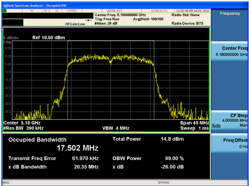
Plot 6-4. 26dB Bandwidth Plot (20MHz BW 802.11n (UNII Band 1) – Ch. 36) – Chain A
