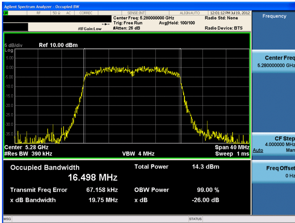
Plot 6-10. 26dB Bandwidth Plot (802.11a (UNII Band 2) – Ch. 56) – Chain A
