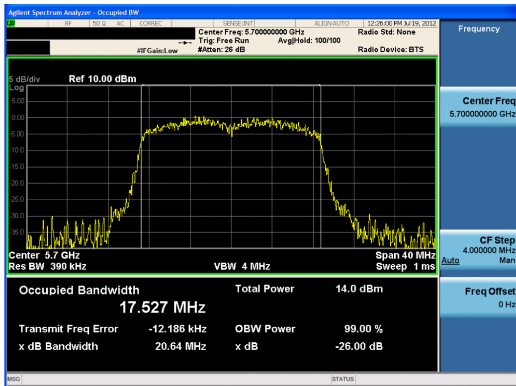
Plot 6-22. 26dB Bandwidth Plot (20MHz BW 802.11n (UNII Band 3) – Ch. 140) – Chain A
