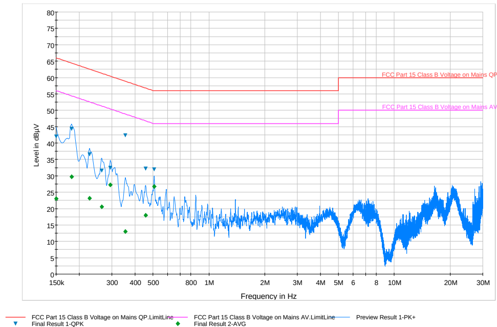
Plot 6-59. Line Conducted Plot with 802.11b (L1)
