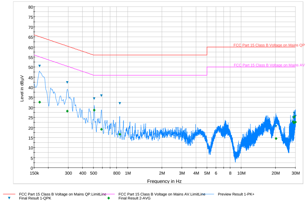
Plot 6-78. Line Conducted Plot with 802.11a UNII Band 2 (L1)
