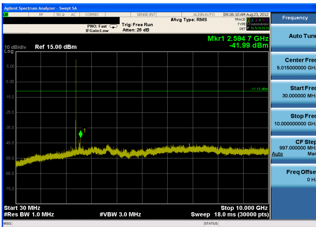
Plot 6-36. Conducted Spurious Plot (Bluetooth, 3Mbps – Ch. 0)
