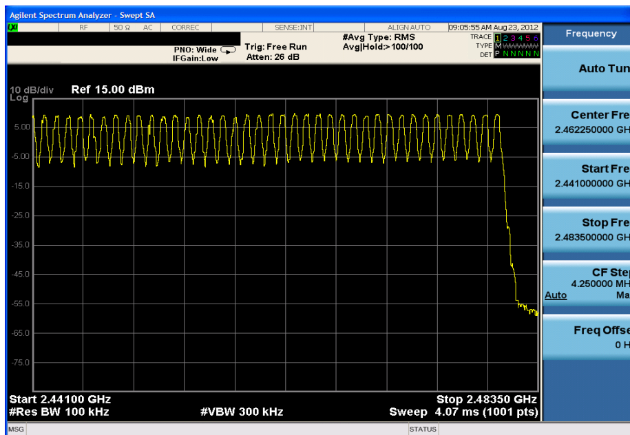
Plot 6-35. High End Spectrum Channel Hopping Plot (Bluetooth)
