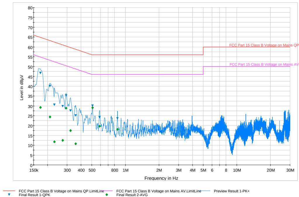
Plot 6-42. Line-Conducted Test Plot (L1)
