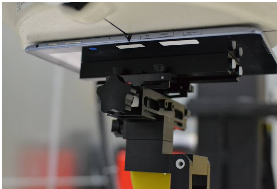
SAR Test Setup Photo 1 – Back Side Touching
