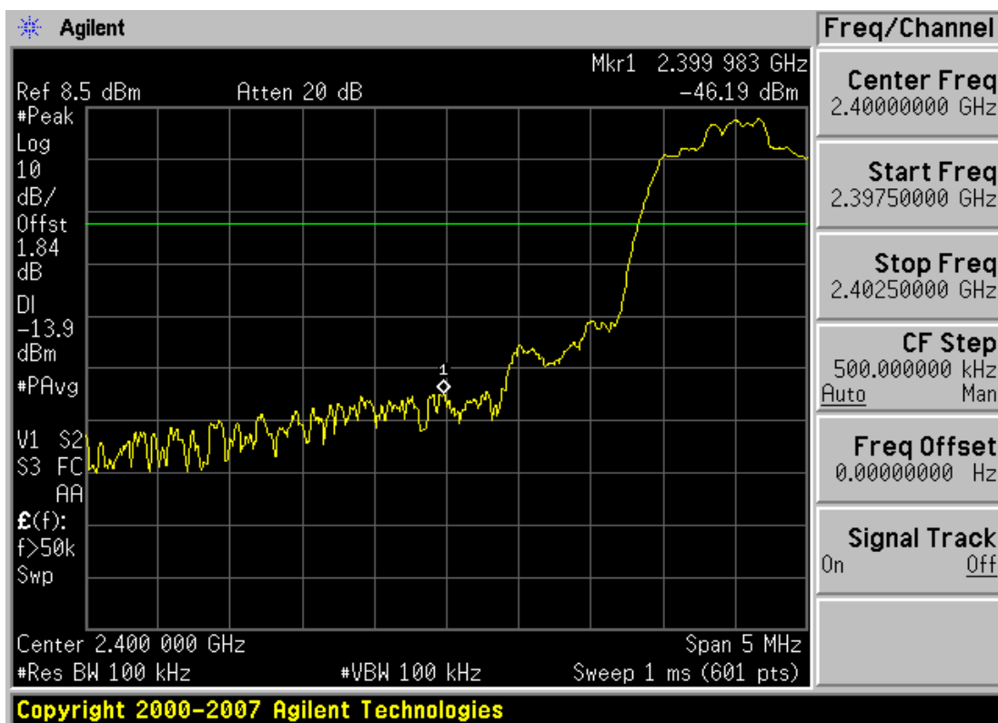
Plot 6-6. Band Edge Plot (Bluetooth 2.1 with Enhanced Data Rate – Ch. 0)
