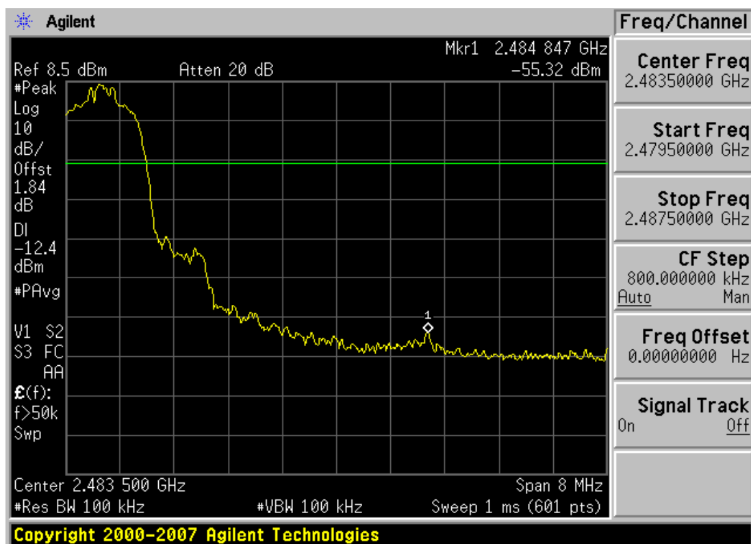
Plot 6-7. Band Edge Plot (Bluetooth 2.1 with Enhanced Data Rate – Ch. 78)
