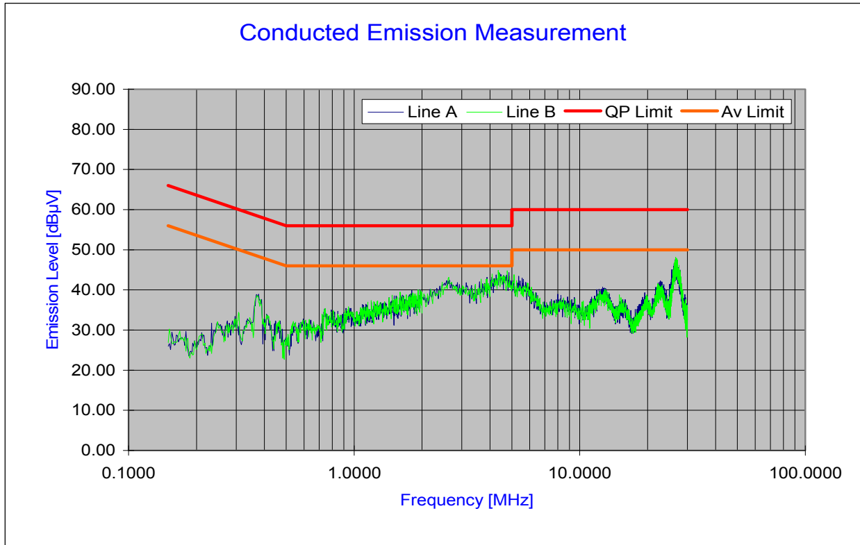
Plot 6-31. Line Conducted Plot with 802.11b
