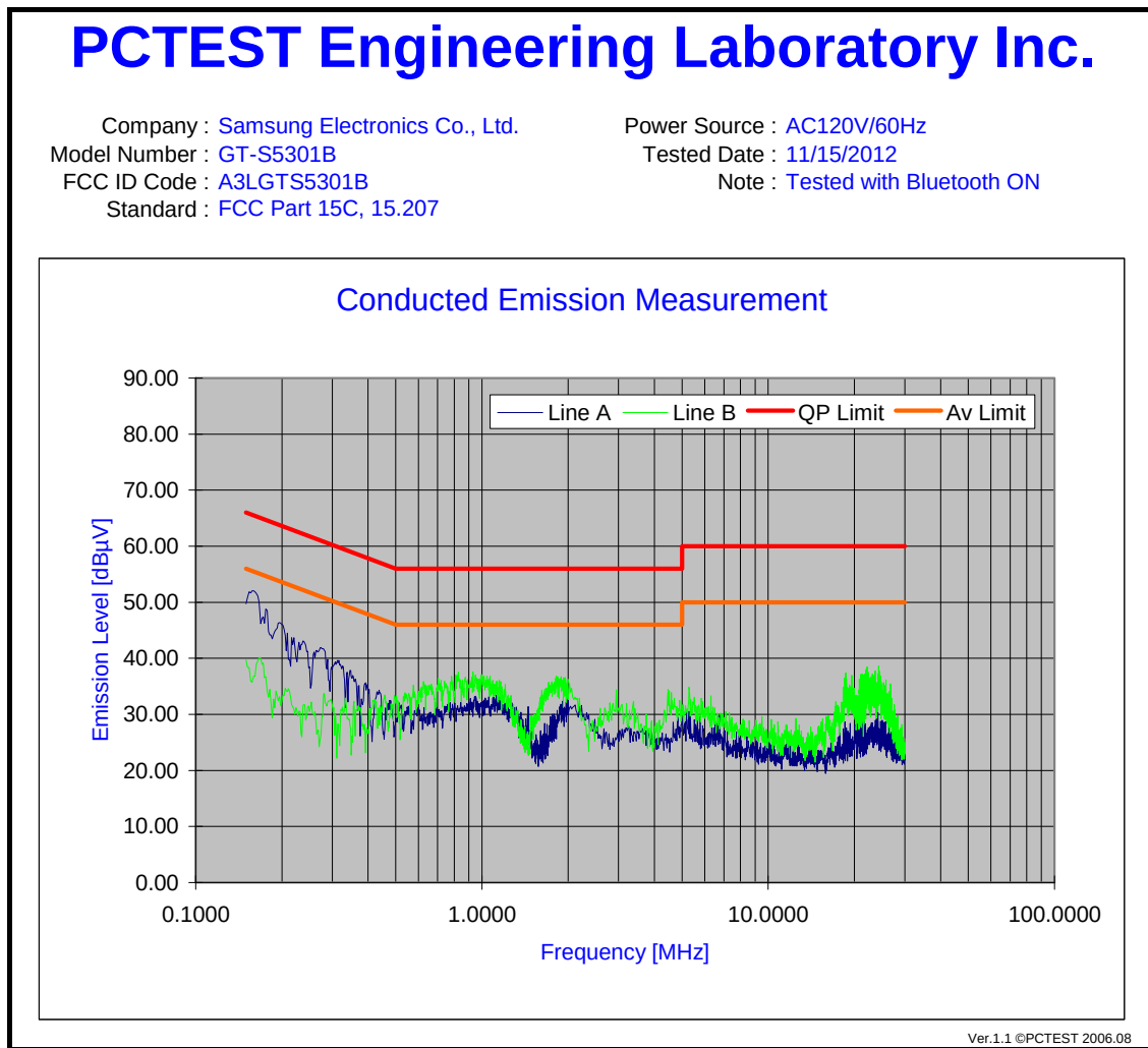
Plot 6-42. Line Conducted Plot with Bluetooth
