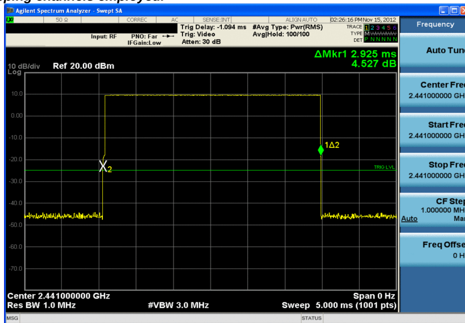
Plot 6-33. Time of Occupancy Plot (Bluetooth)
