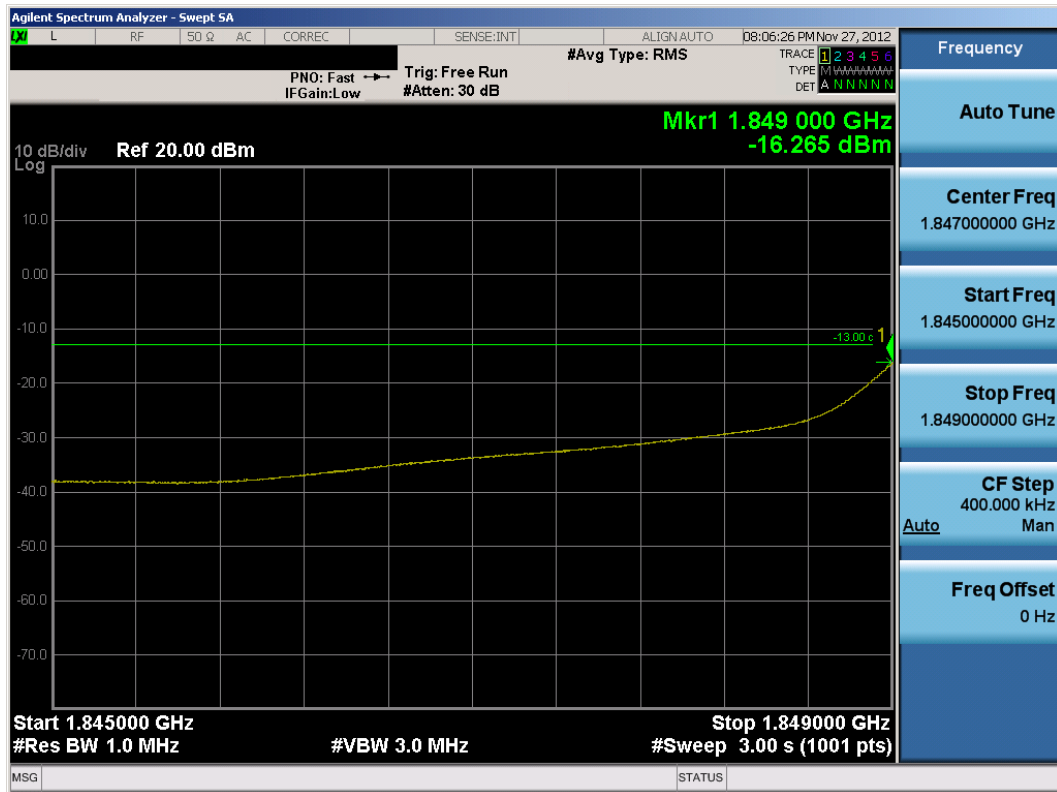
Plot 7-34. 4MHz Span Plot (PCS WCDMA Mode – Ch. 9262)
