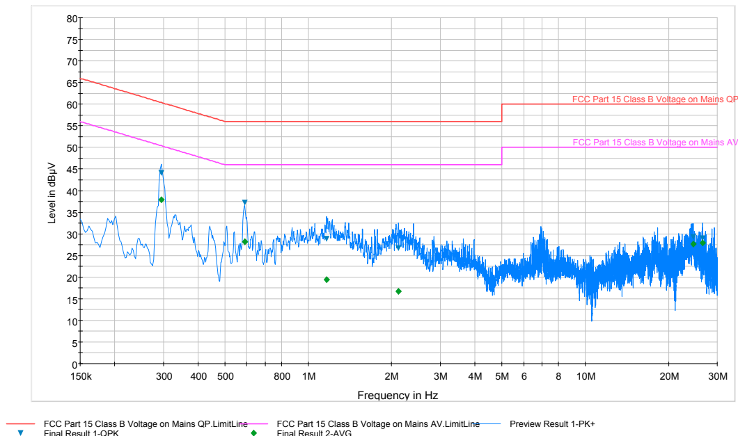
Plot 6-31. Line Conducted Plot with 802.11a (L1)
