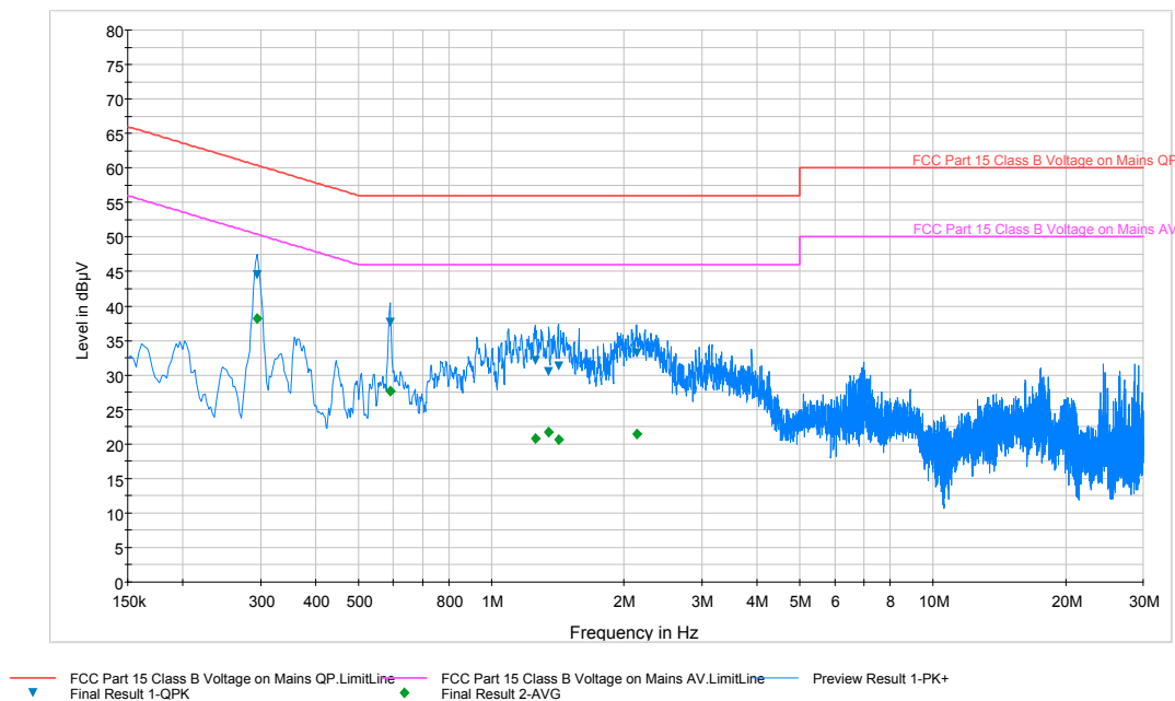
Plot 6-32. Line Conducted Plot with 802.11a (N)
