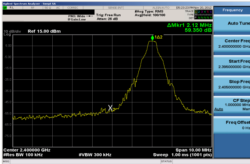
Plot 6-28. Band Edge Plot (Bluetooth with Hopping Disabled, 1Mbps – Ch. 0)
