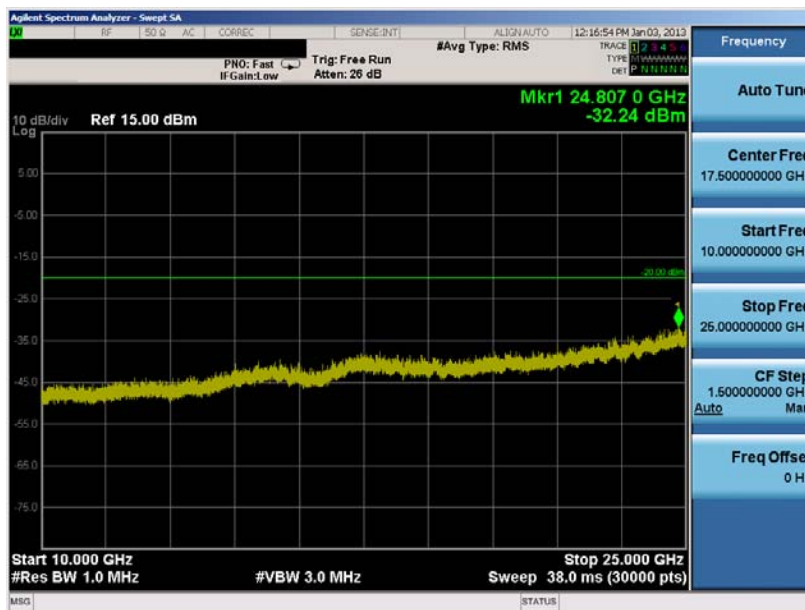
Plot 6-26. Conducted Spurious Plot (802.11b – Ch. 1)
