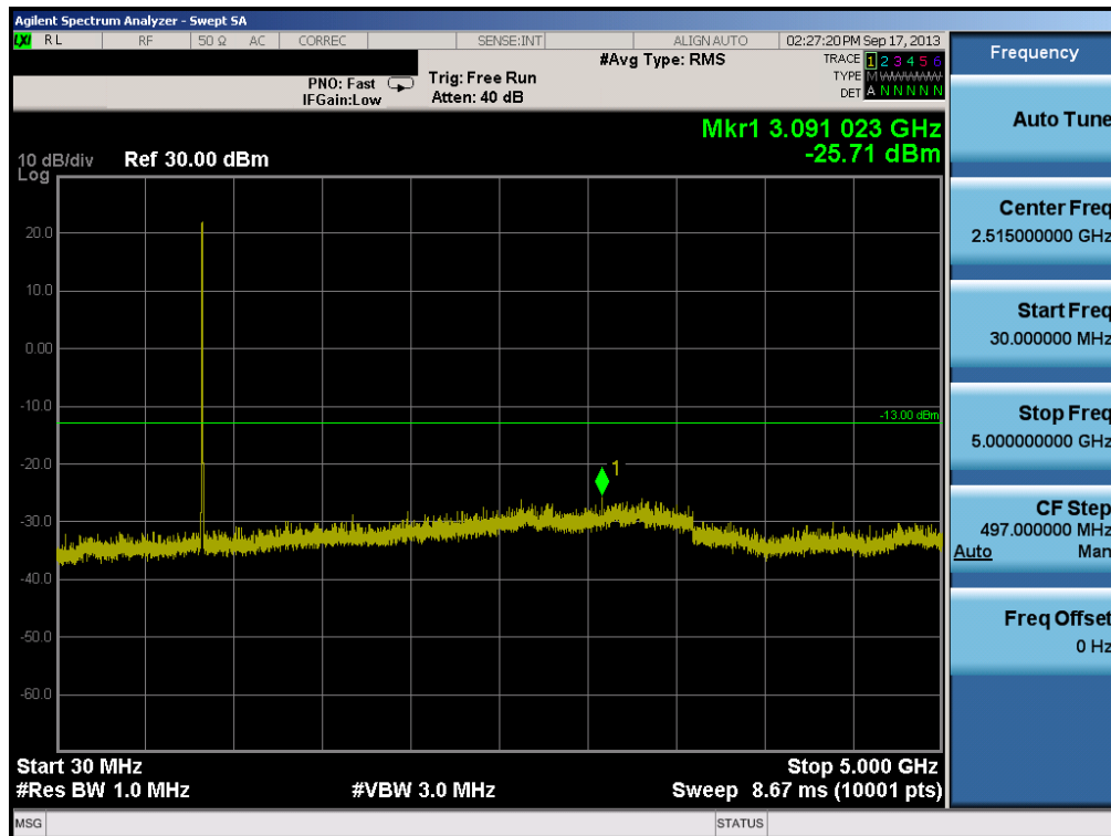
Plot 6-23. Conducted Spurious Plot (Cellular WCDMA Mode – Ch. 4233)
