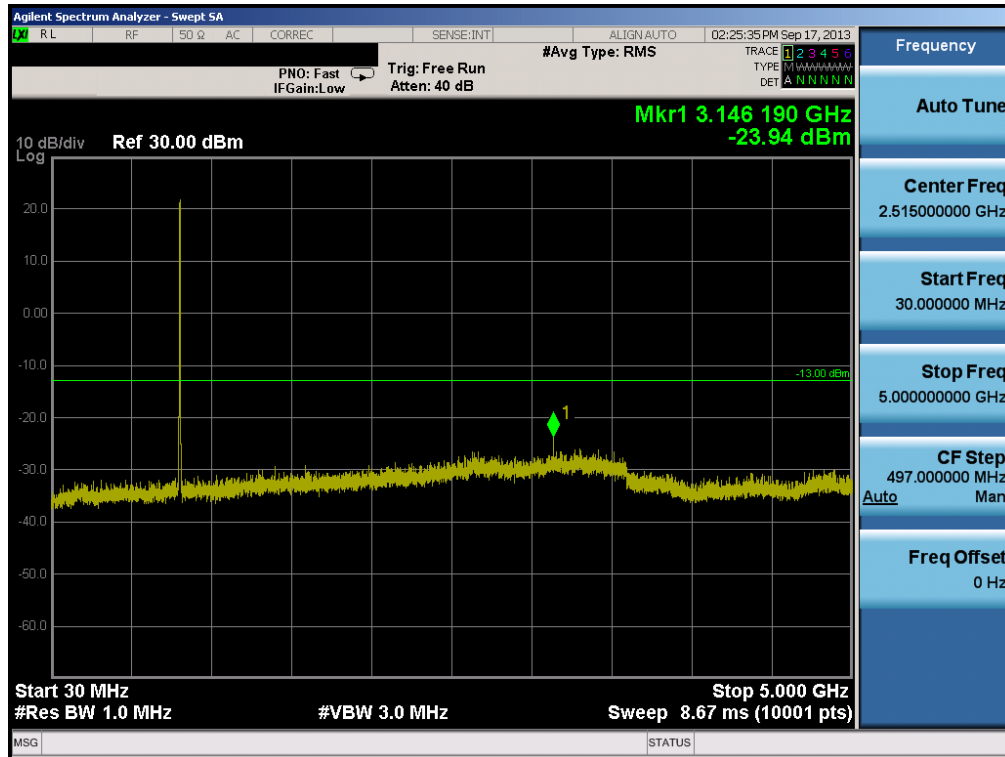
Plot 6-19. Conducted Spurious Plot (Cellular WCDMA Mode – Ch. 4132)
