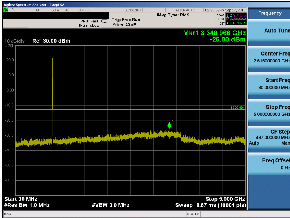
Plot 6-21. Conducted Spurious Plot (Cellular WCDMA Mode – Ch. 4183)
