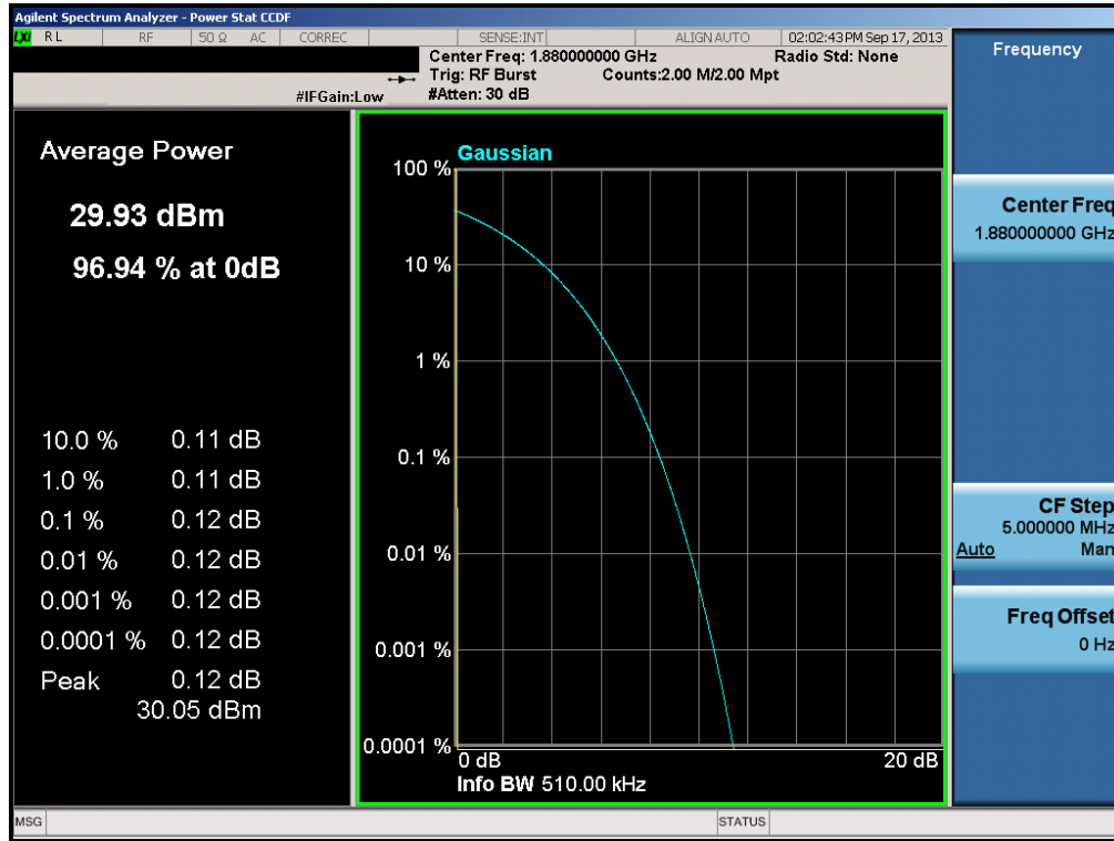
Plot 6-31. Peak-Average Ratio Plot (PCS GSM Mode – Ch. 661)
