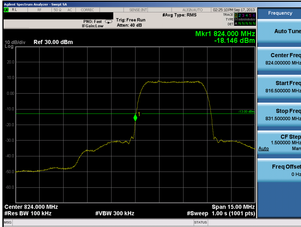
Plot 6-29. Band Edge Plot (Cellular WCDMA Mode – Ch. 4132)
