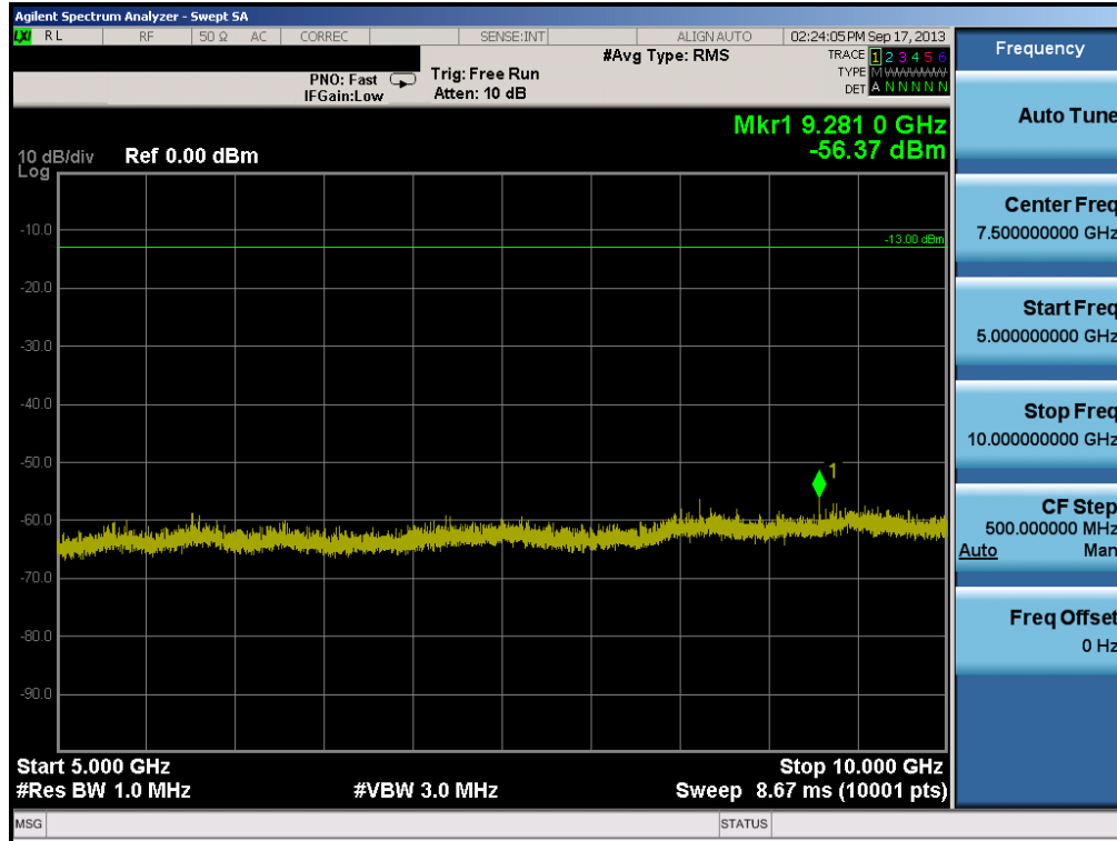
Plot 6-22. Conducted Spurious Plot (Cellular WCDMA Mode – Ch. 4183)
