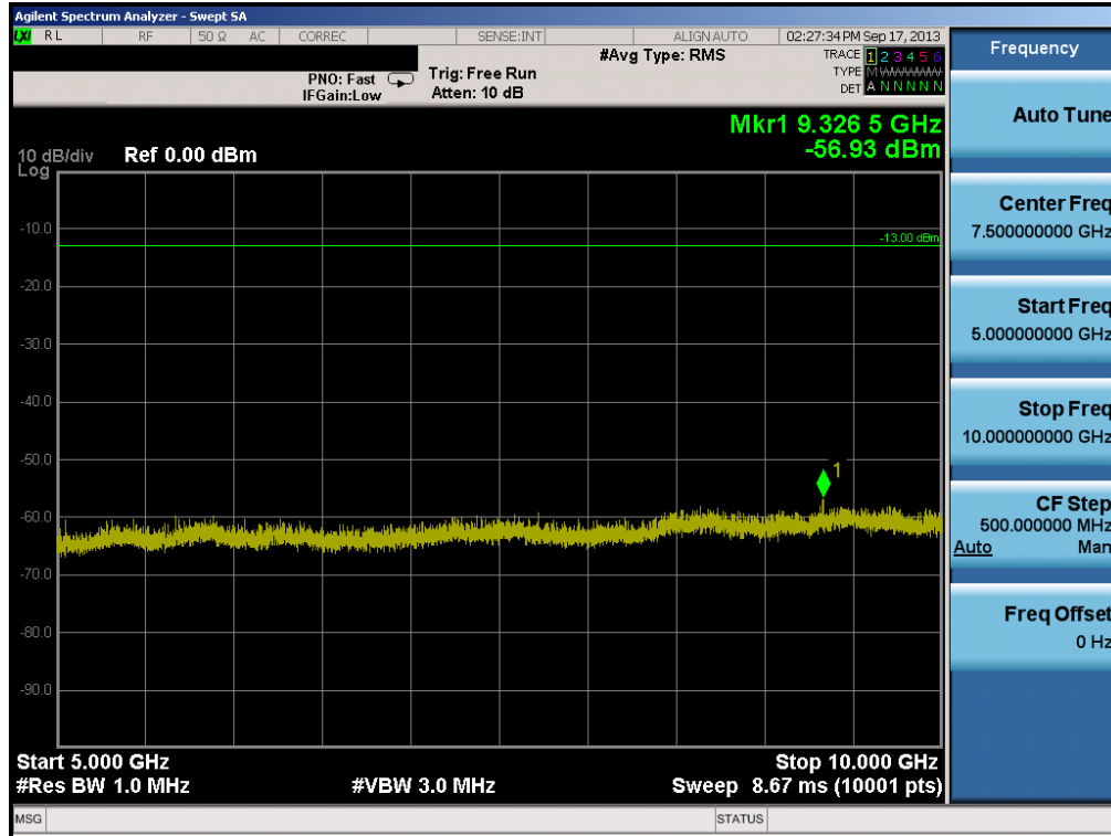
Plot 6-24. Conducted Spurious Plot (Cellular WCDMA Mode – Ch. 4233)
