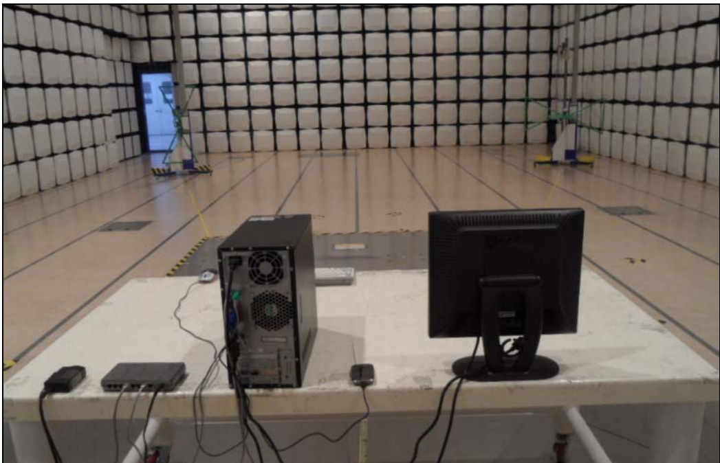
[ Radiated Disturbance for Below 1 GHz – Rear ]
