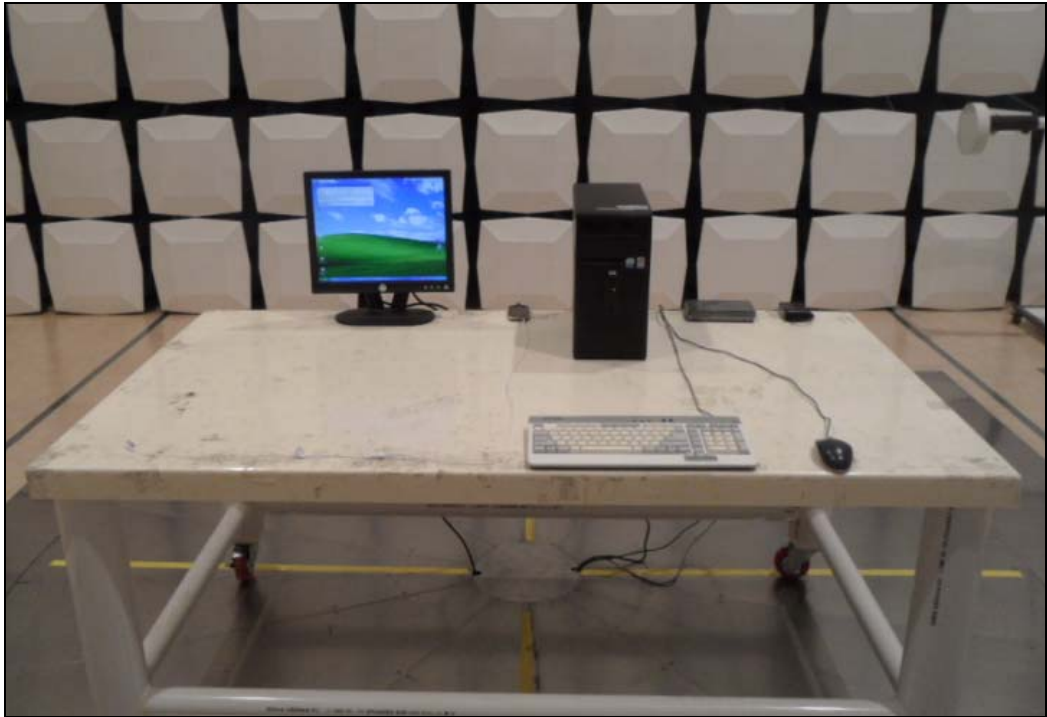
[ Radiated Disturbance for Below 1 GHz – Front ]
