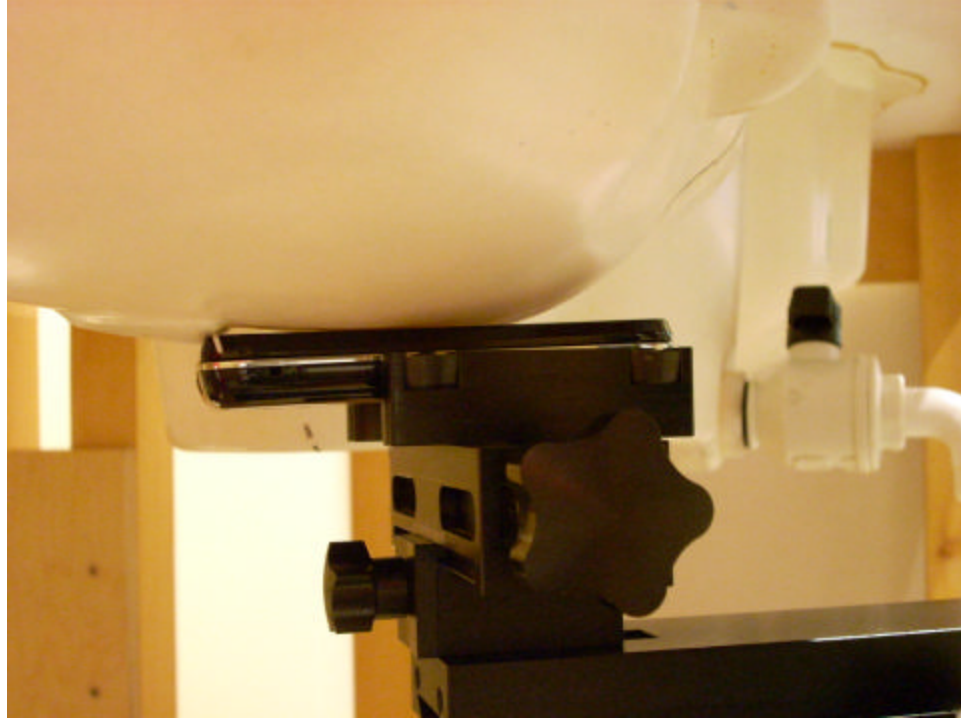
Figure 20-1 SAR Test Setup Photo 1
