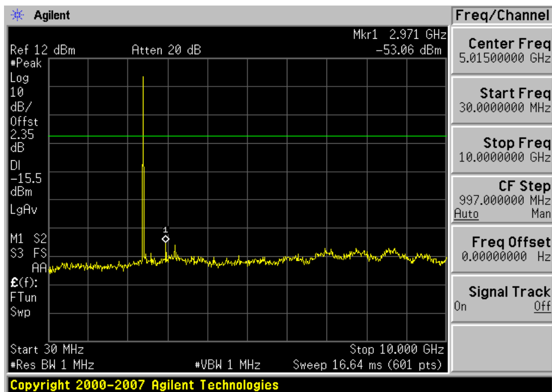
Plot 6-18. Conducted Spurious Plot (Bluetooth, 3Mbps – Ch. 0)
