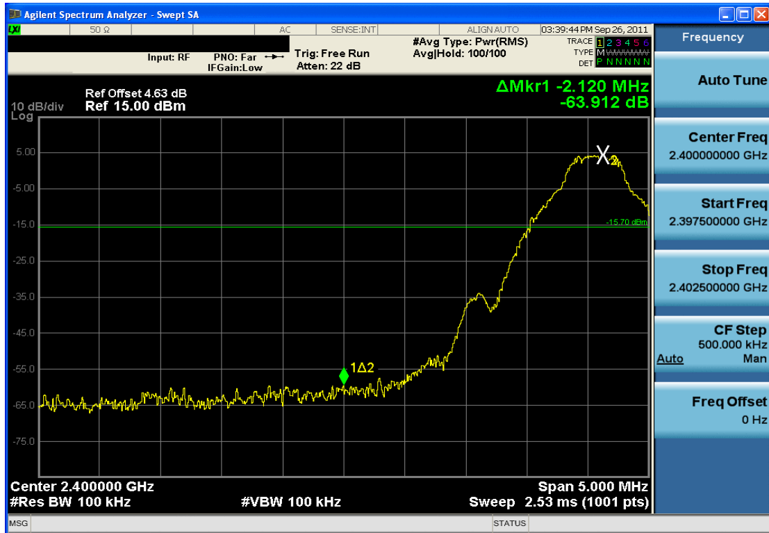
Plot 6-10. Band Edge Plot (Bluetooth, 1Mbps – Ch. 0)
