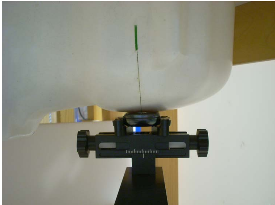
Figure 19-6 SAR Test Setup Photo 6
