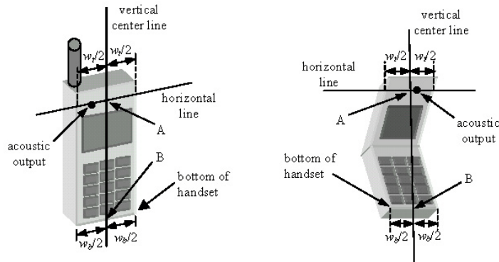
Figure 7-5 Handset Vertical Center & Horizontal Line Reference Points
