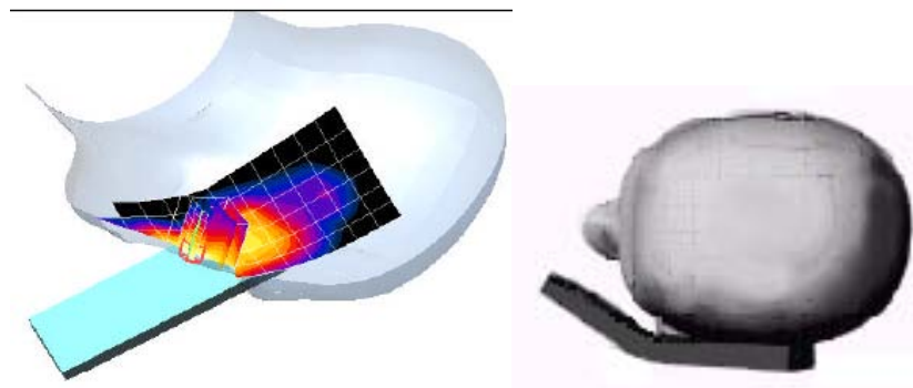
Figure 8-5 SAR Scans near the Jaw/Mouth
