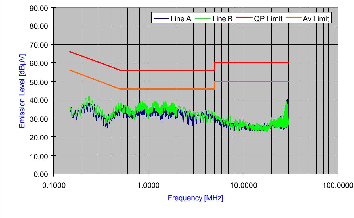
Plot 6-33. Line Conducted Plot with 802.11n
