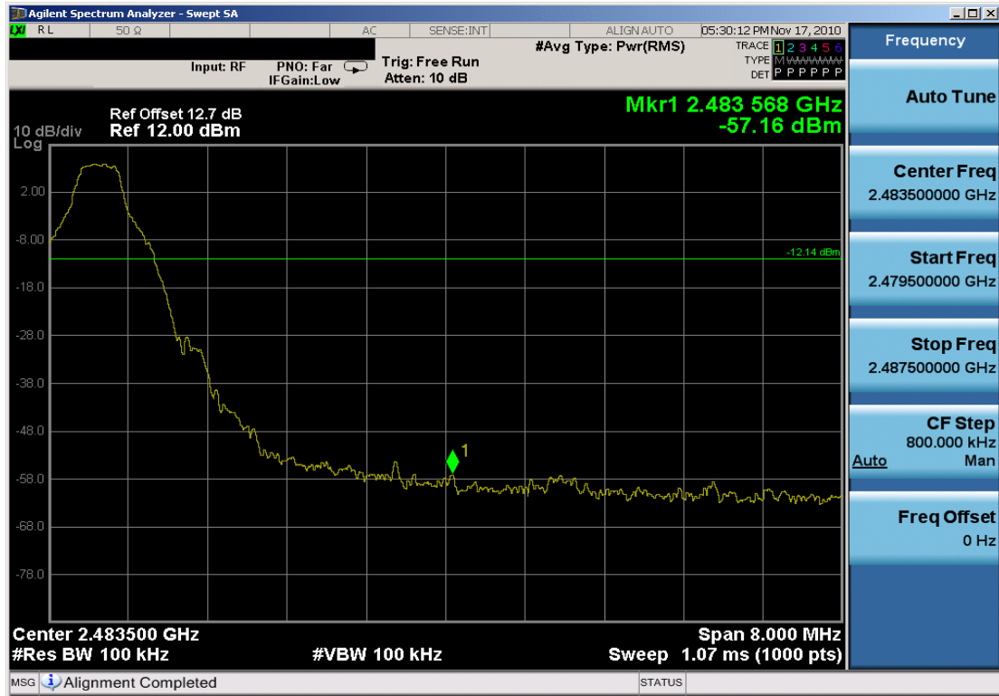
Plot 6-11. Band Edge Plot (Bluetooth, 1Mbps – Ch. 78)
