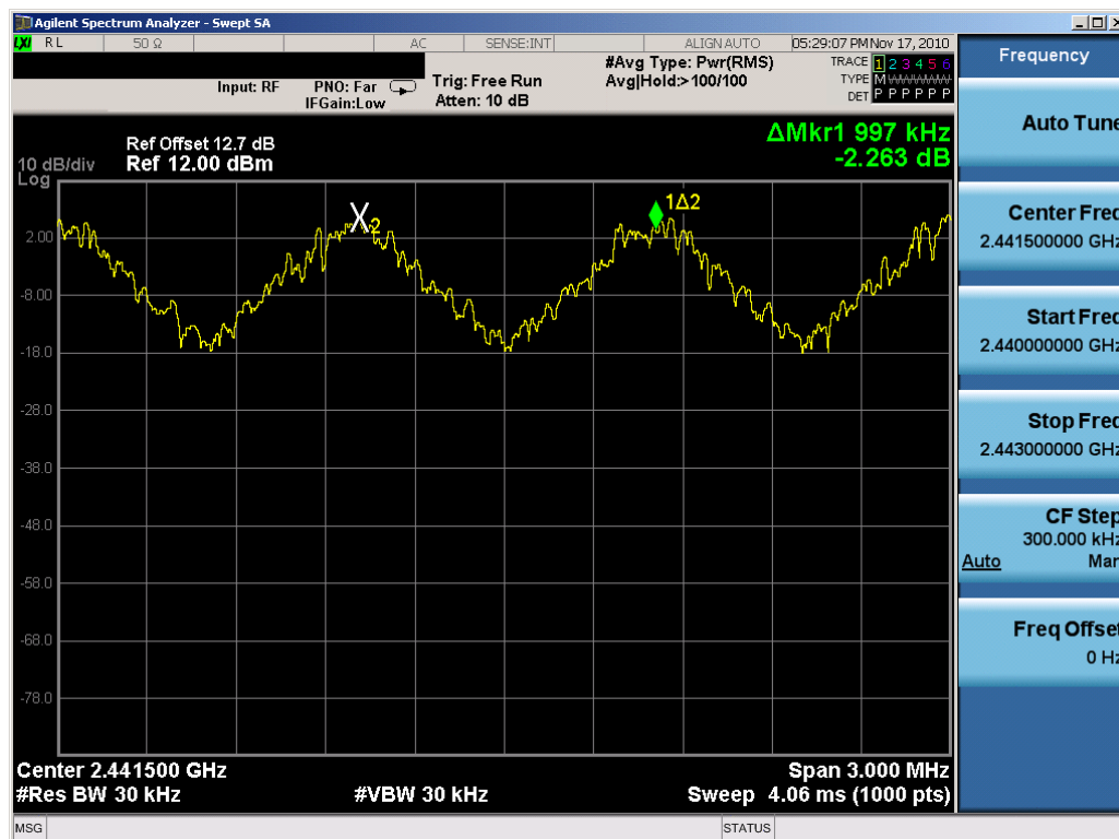
Plot 6-14. Channel Spacing Plot (Bluetooth)
