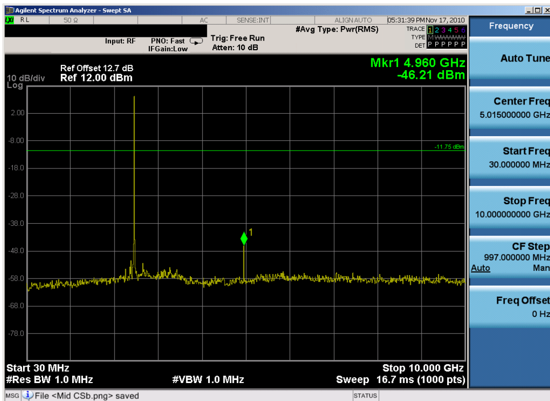
Plot 6-22. Conducted Spurious Plot (Bluetooth, 3Mbps – Ch. 78)
