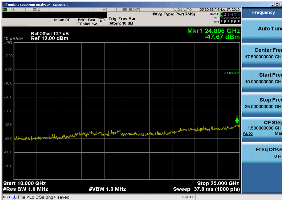
Plot 6-19. Conducted Spurious Plot (Bluetooth, 3Mbps – Ch. 0)
