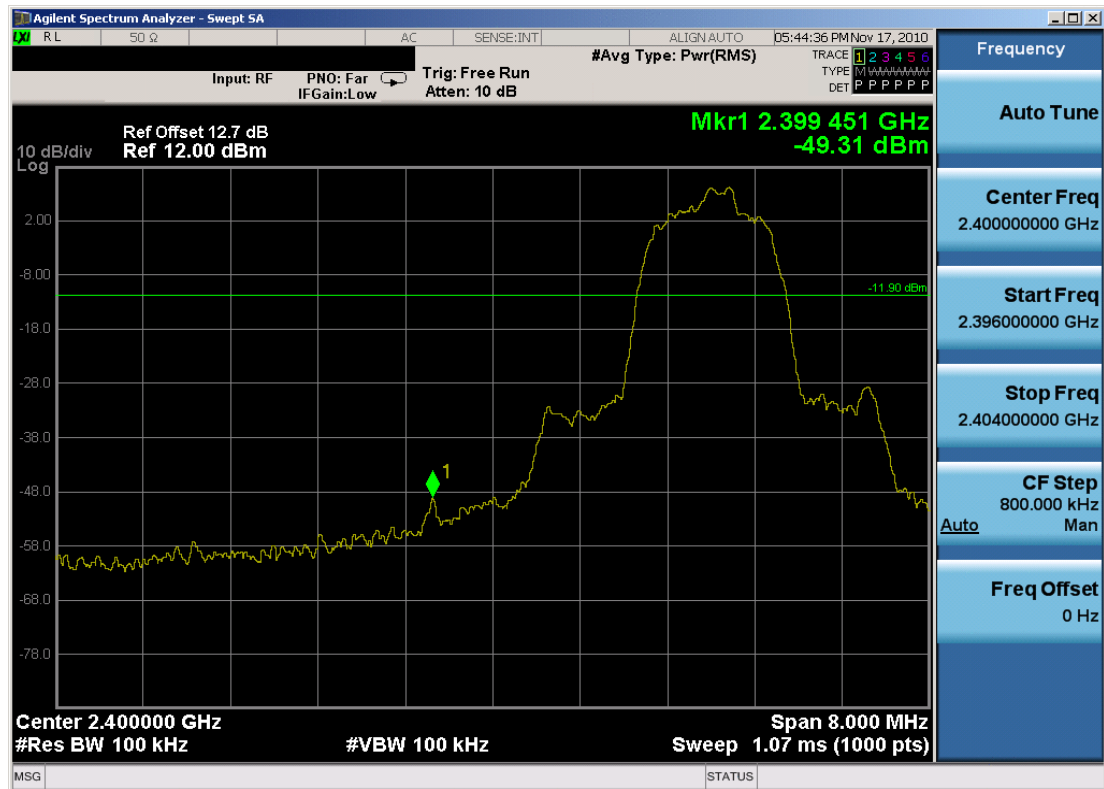
Plot 6-12. Band Edge Plot (Bluetooth, 3Mbps – Ch. 0)
