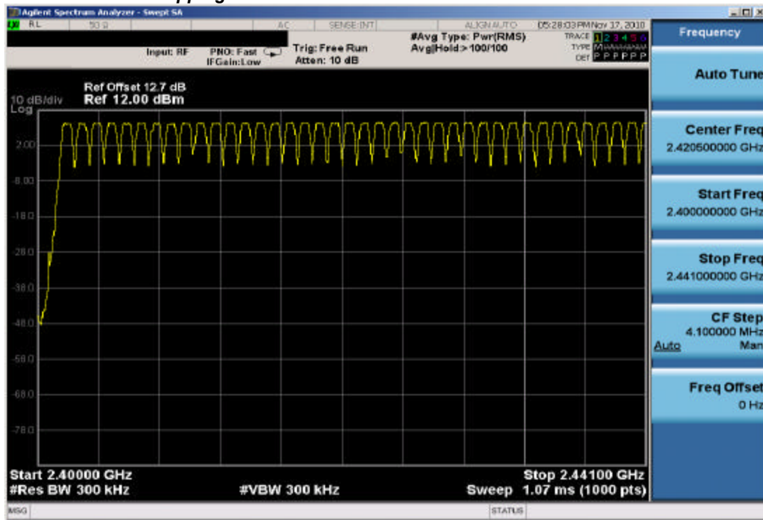
Plot 6-16. Low End Spectrum Channel Hopping Plot (Bluetooth)
