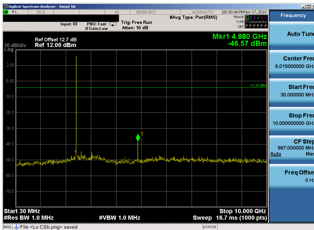
Plot 6-20. Conducted Spurious Plot (Bluetooth, 3Mbps – Ch. 39)
