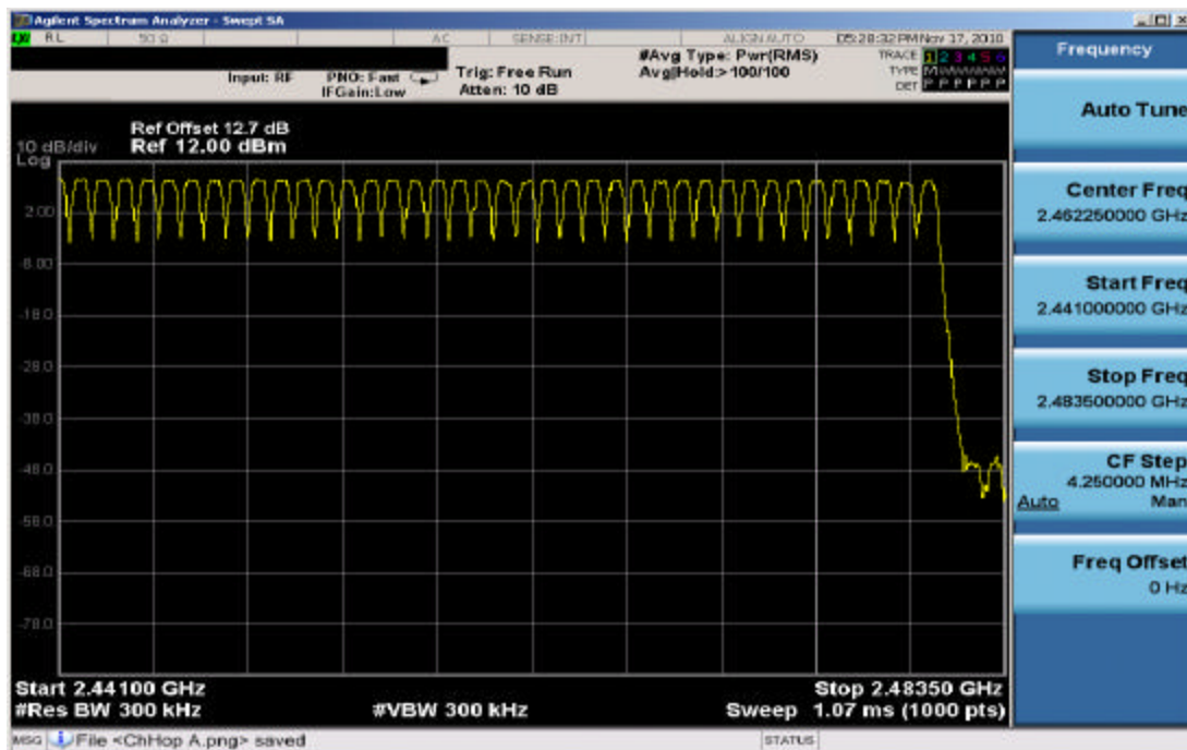
Plot 6-17. High End Spectrum Channel Hopping Plot (Bluetooth)
