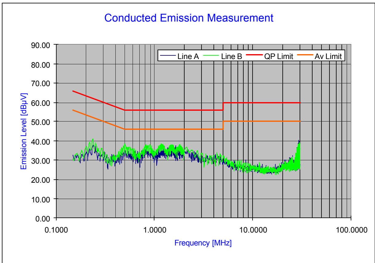
Plot 6-24. Line Conducted Plot with Bluetooth
