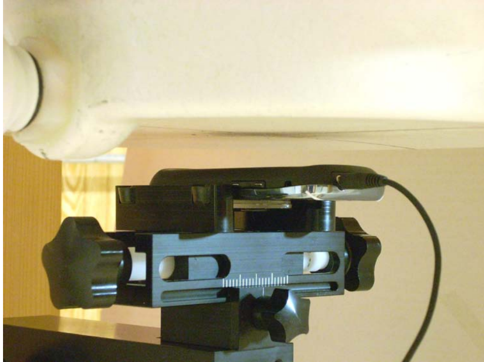
Figure 19-5 SAR Setup Photo 5
