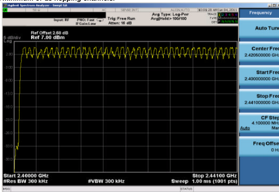
Plot 6-16. Low End Spectrum Channel Hopping Plot (Bluetooth)
