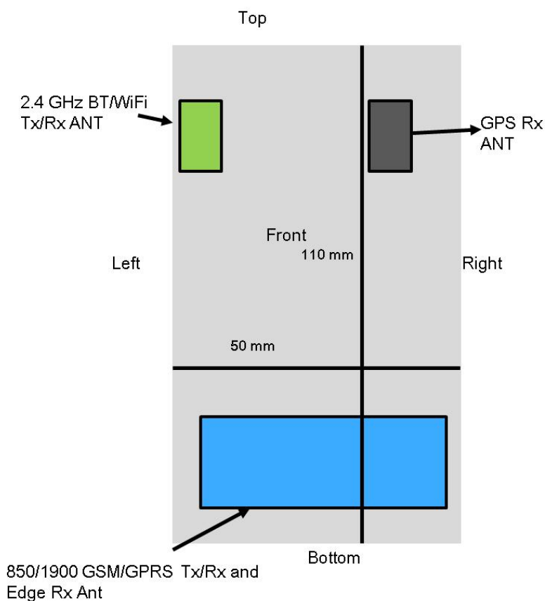
Figure 13-1 Identification of Sides for SAR Testing
