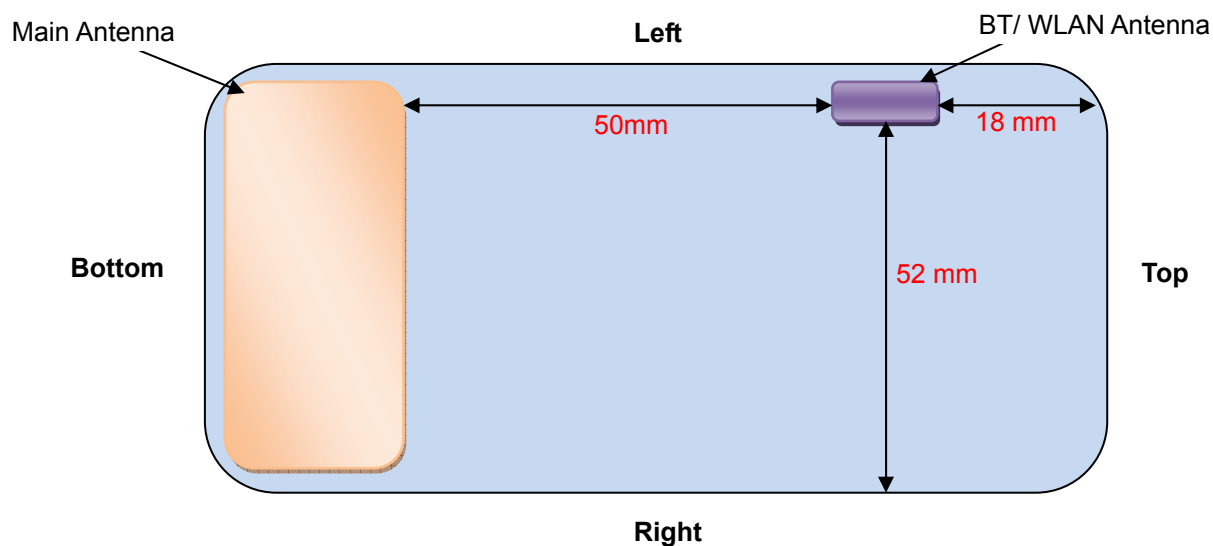
Figure 8.2 Identification of Sides for SAR Testing
