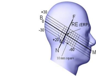
Figure 5.3 Side view of the phantom showing relevant markings
