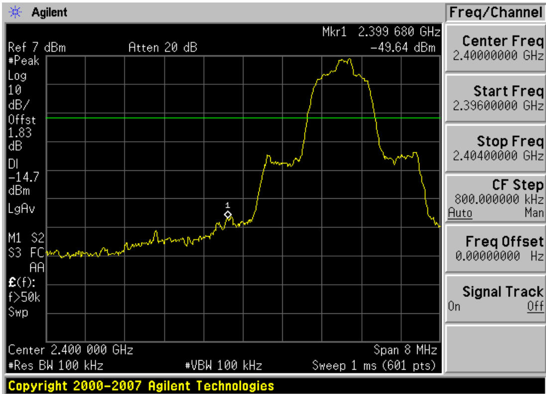
Plot 6-6. Band Edge Plot (Bluetooth 2.1 with Enhanced Data Rate – Ch. 0)
