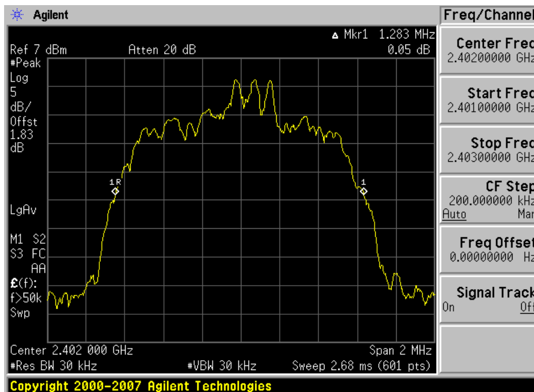
Plot 6-1. 20dB Bandwidth Plot (Bluetooth 2.1 with Enhanced Data Rate – Ch. 0)
