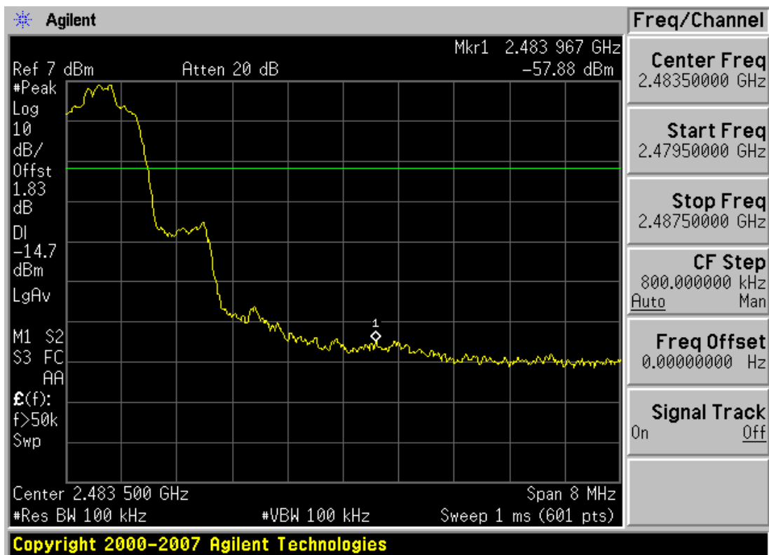
Plot 6-7. Band Edge Plot (Bluetooth 2.1 with Enhanced Data Rate – Ch. 78)
