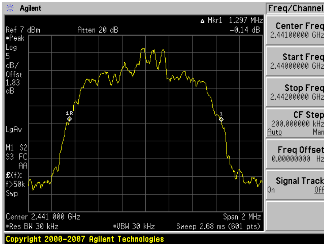
Plot 6-2. 20dB Bandwidth Plot (Bluetooth 2.1 with Enhanced Data Rate – Ch. 39)
