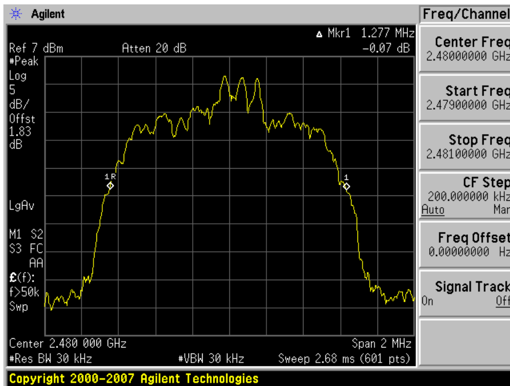
Plot 6-3. 20dB Bandwidth Plot (Bluetooth 2.1 with Enhanced Data Rate – Ch. 78)
