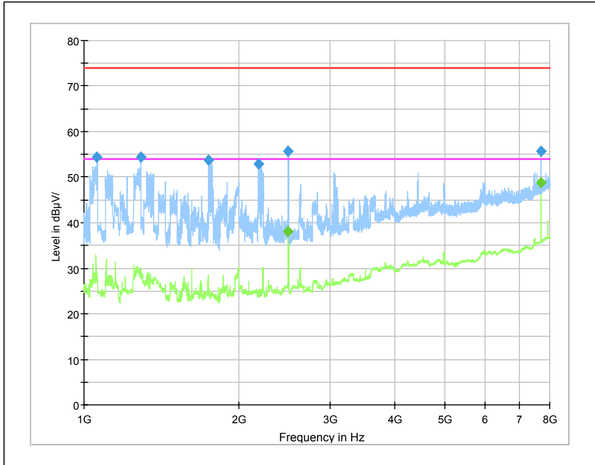
Quasi-peak/ Average final measurement results table:
