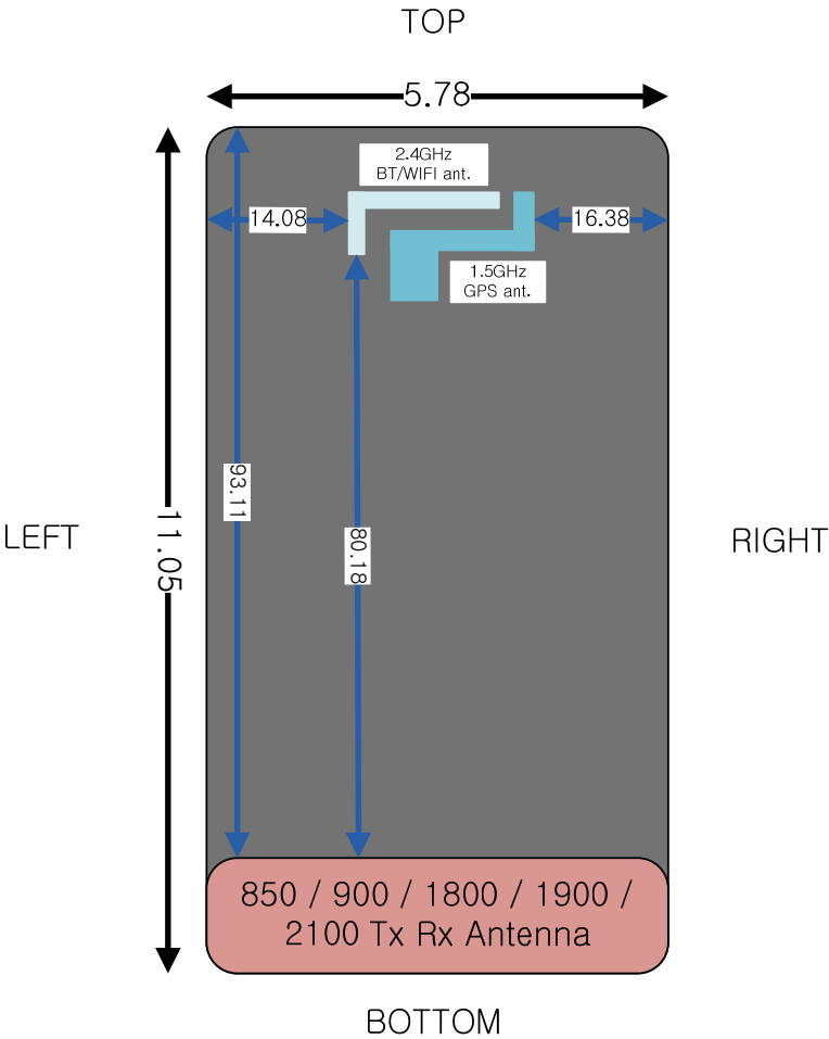
Figure 5.9 Antenna Locations, as viewed from Front of device
