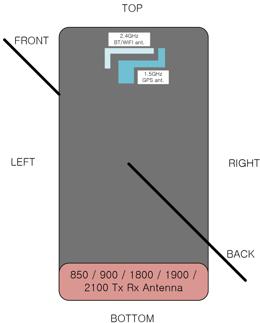
Figure 5.8 Identification of Sides for SAR Testing
