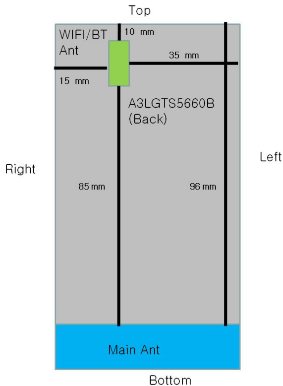
Figure 13-1 Identification of Sides for SAR Testing
