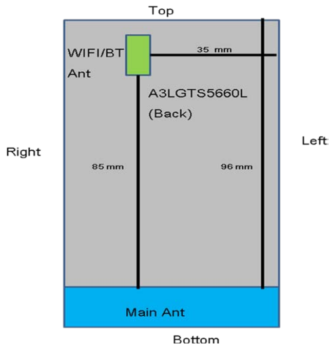
Figure 13-1 Identification of Sides for SAR Testing
