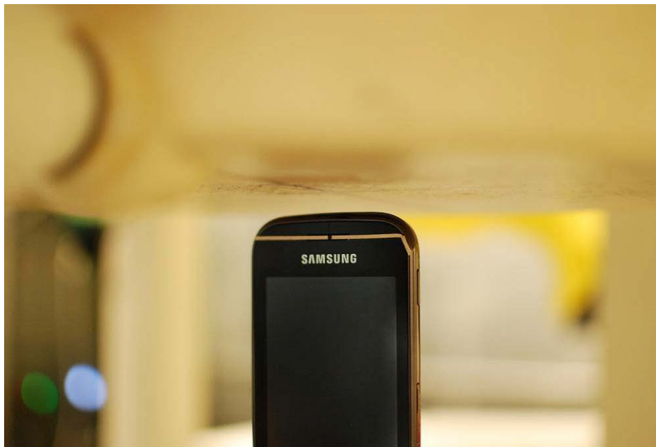
Figure 21-9 SAR Test Setup Photo 9 – Top at 1.0 cm
