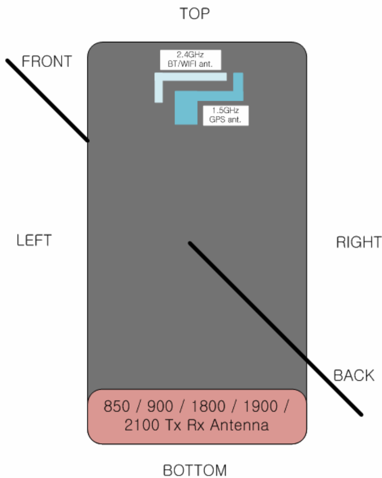
Figure 5.7 Identification of Sides for SAR Testing
