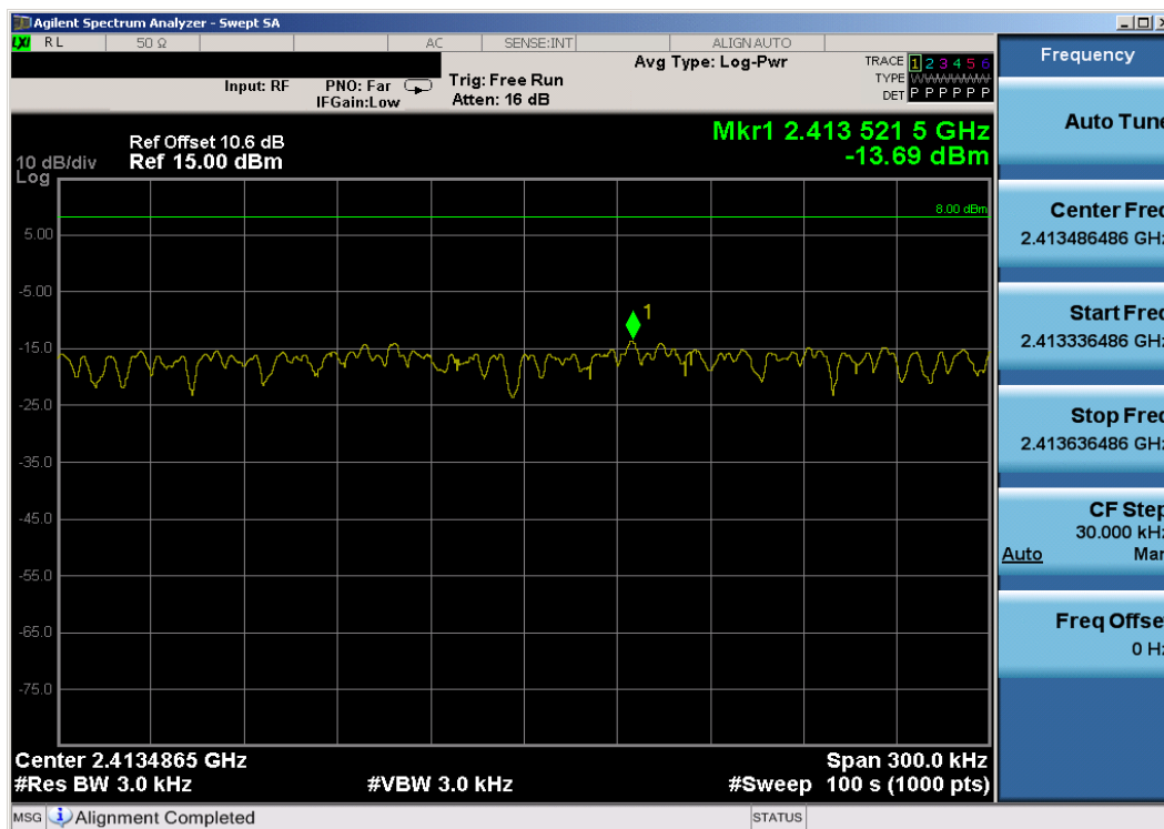
Plot 6-10. Power Spectral Density Plot (802.11b – Ch. 1)
