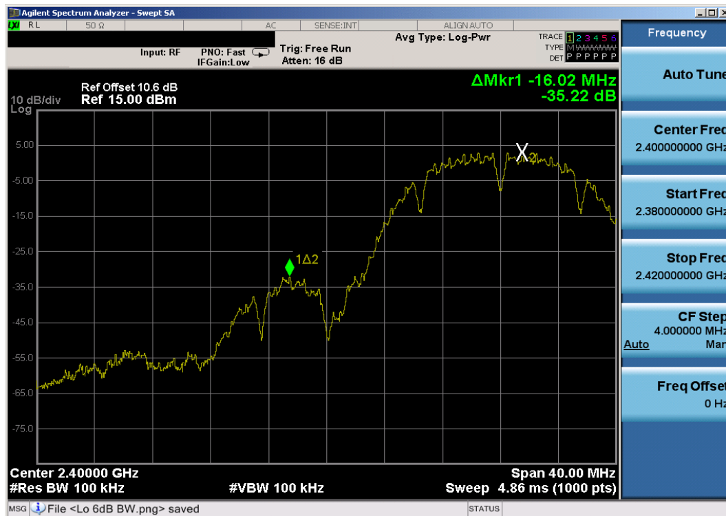
Plot 6-19. Band Edge Plot (802.11b – Ch. 1)
