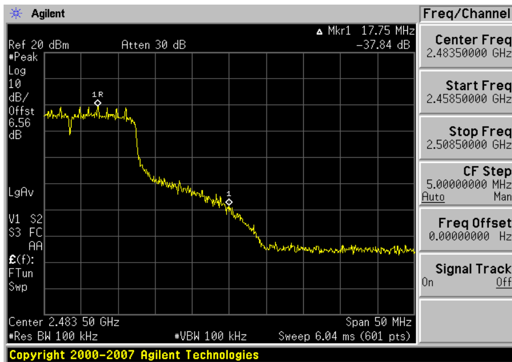
Plot 6-24. Band Edge Plot (802.11n – Ch. 11)
