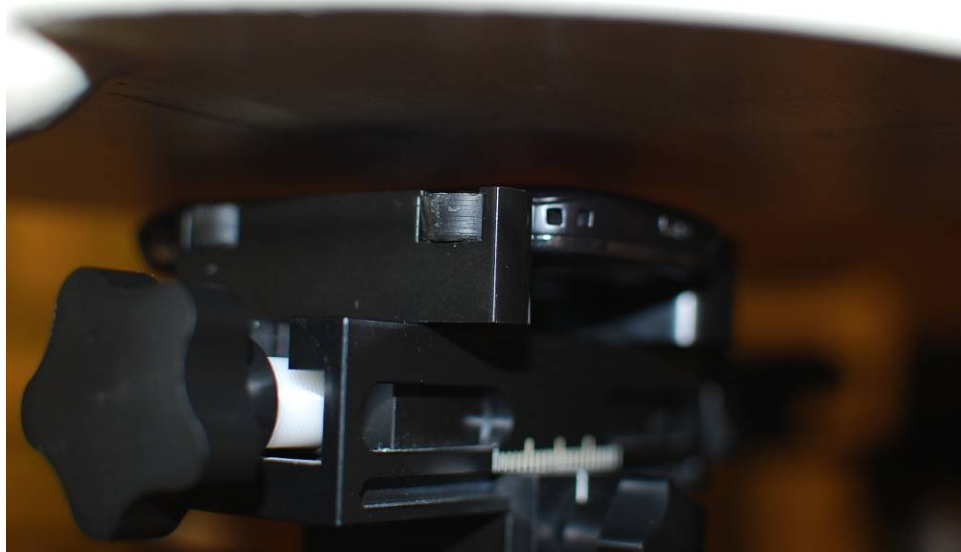
Figure 21-5 SAR Test Setup Photo 5 Body Back at 1.0 cm
