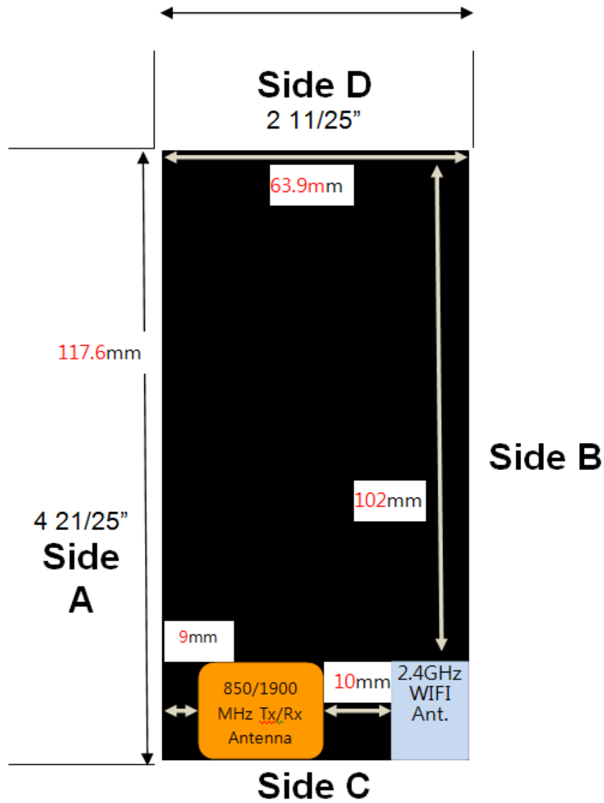
Figure 5.8 Antenna Locations, as viewed from back of device
