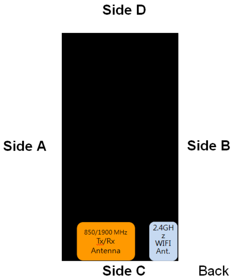
Figure 5.7 Identification of Sides for SAR Testing
