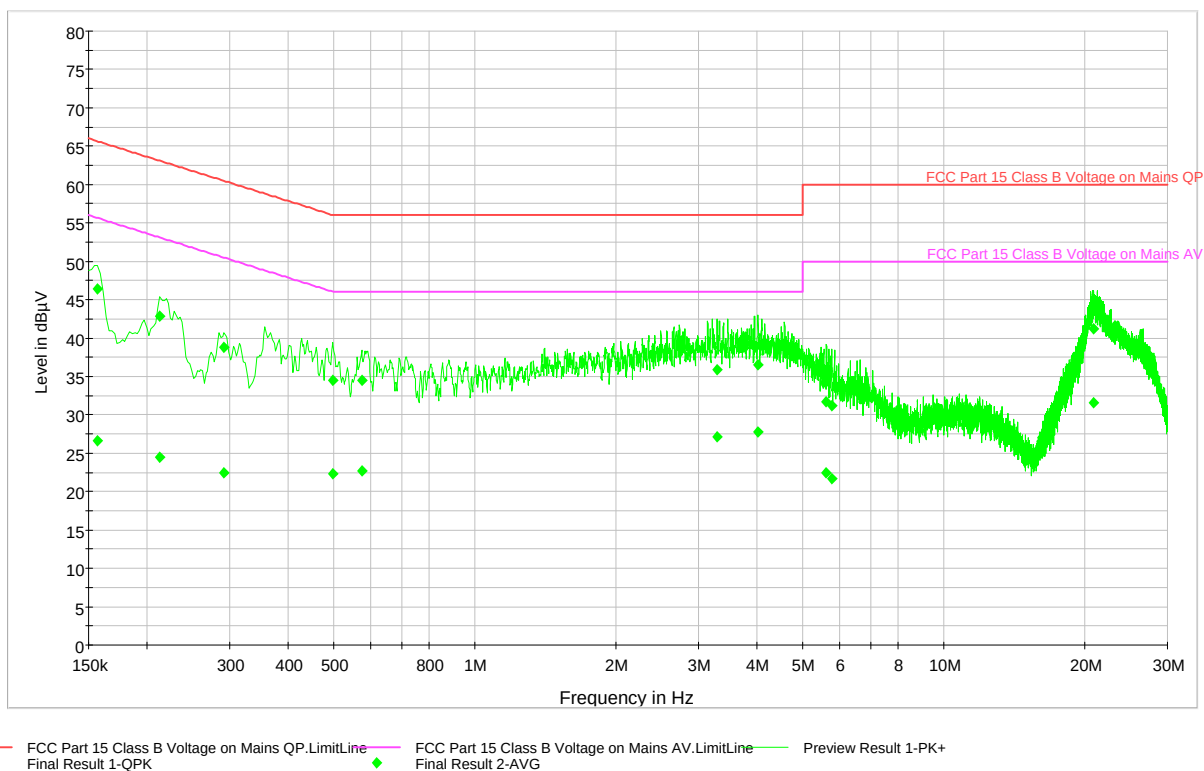
Plot 6-32. Line Conducted Plot with 802.11b (N)
