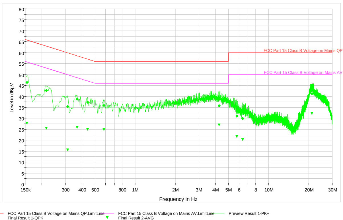
Plot 6-34. Line Conducted Plot with 802.11g (N)
