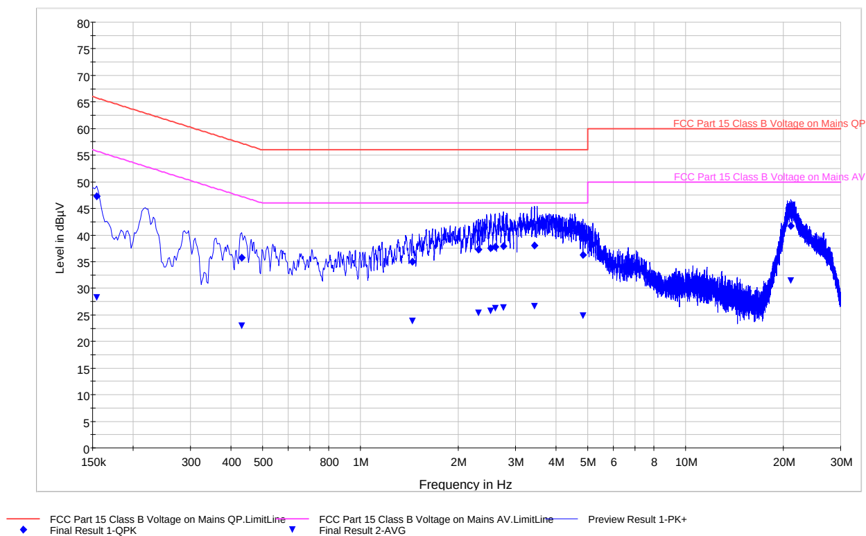
Plot 6-33. Line Conducted Plot with 802.11g (L1)
