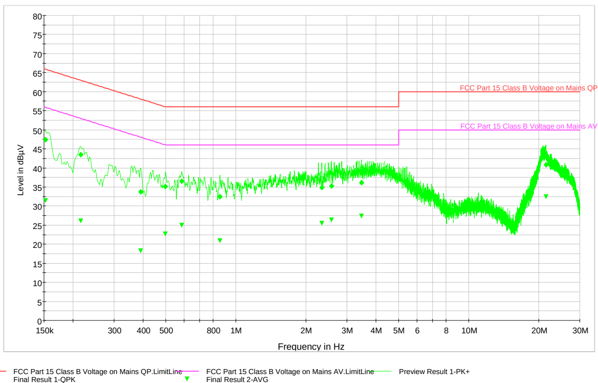
Plot 6-36. Line Conducted Plot with 802.11n (N)
