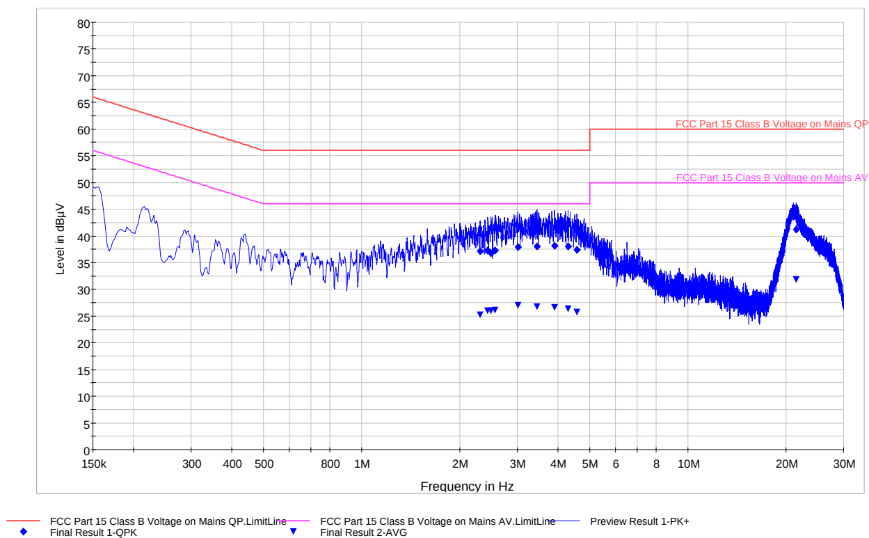
Plot 6-35. Line Conducted Plot with 802.11n (L1)
